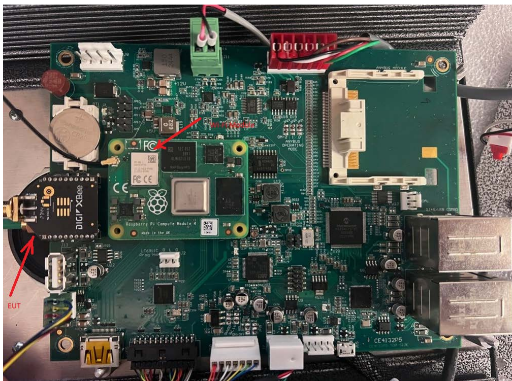
Figure 10 Main PCB View showing two RF Modules
