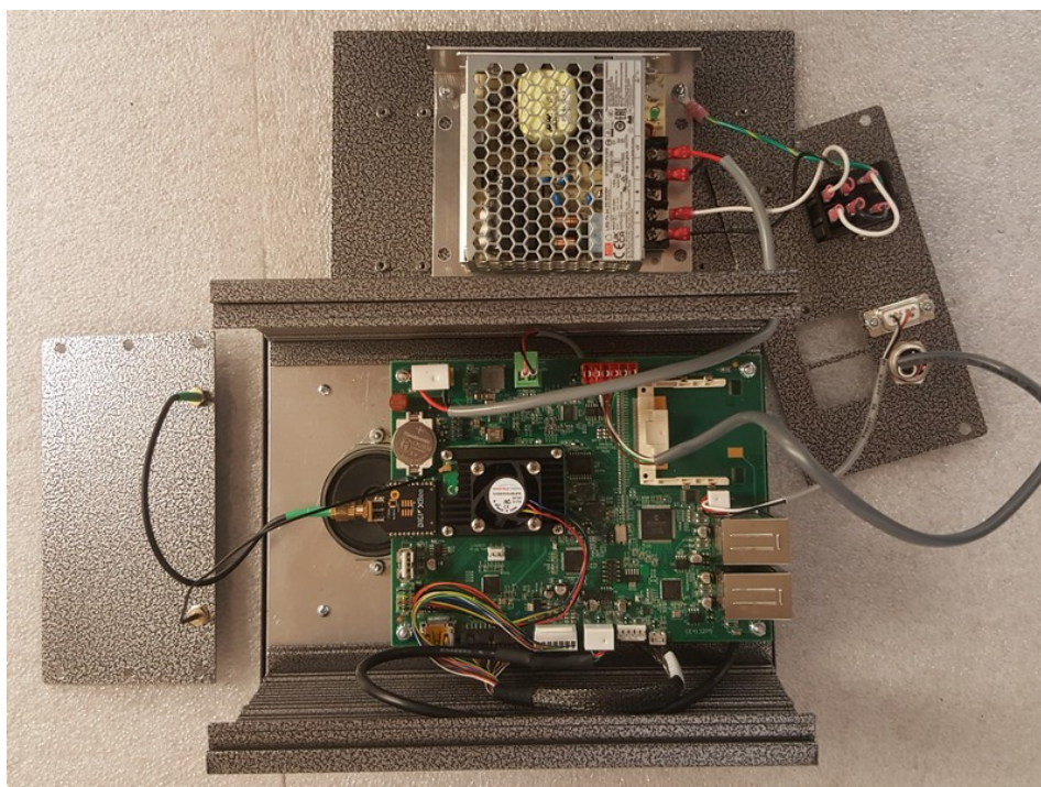
Figure 7 Cover Open View
