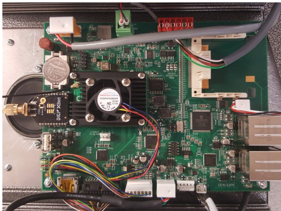
Figure 8 Main PCB Component Side View
