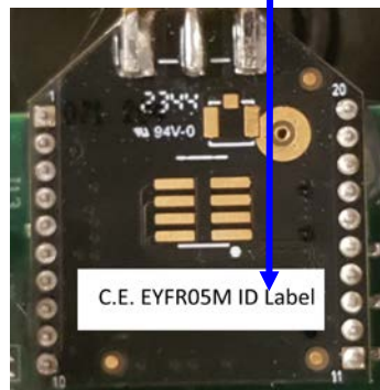
Product Sticker with FCC/IC ID
