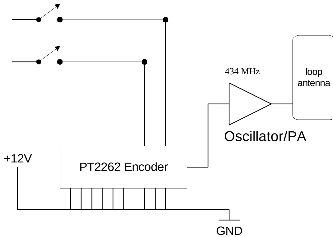
BLOCK DIAGRAM
