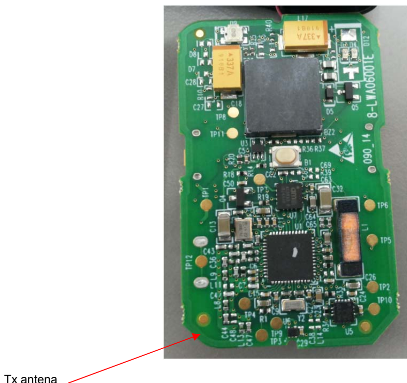
Photograph 7.4.1 Antenna assembly
