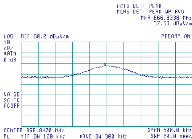
Plot 7.3.13 Radiated emission measurements at the second harmonic frequency
