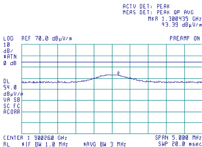
Plot 7.3.15 Radiated emission measurements at the third harmonic frequency
