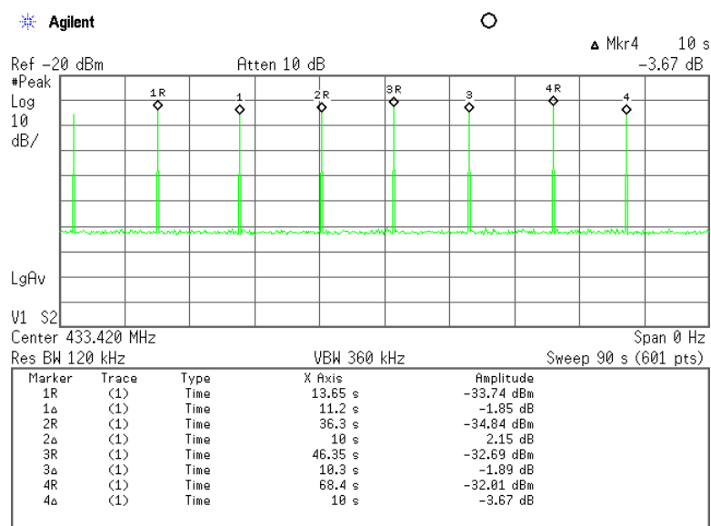
Plot 7.1.7 Polling / supervision transmission period
