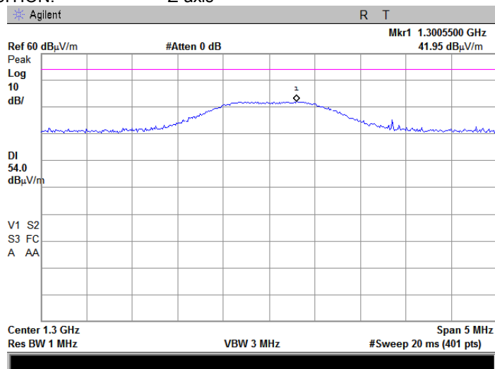
Plot 7.2.8 Radiated emission measurements at the third harmonic frequency
