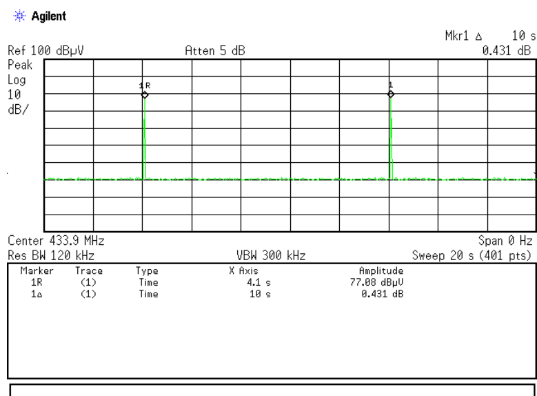
Plot 7.1.3 Polling / supervision transmission period
