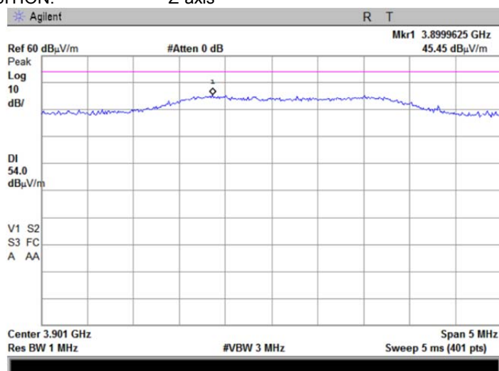
Plot 7.3.17 Radiated emission measurements at the nine harmonic frequency
