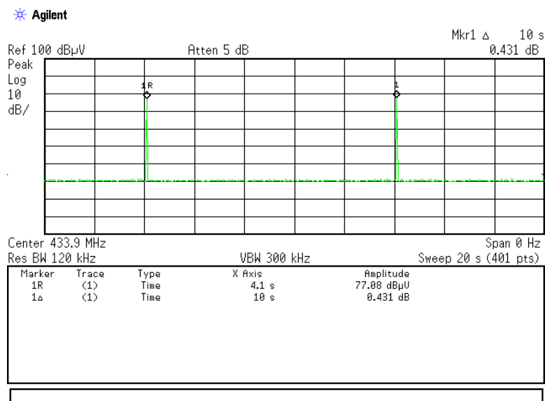
Plot 7.2.12 Transmission pulse period
