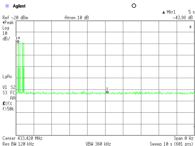
Plot 7.1.4 Transmitter shut down test result
