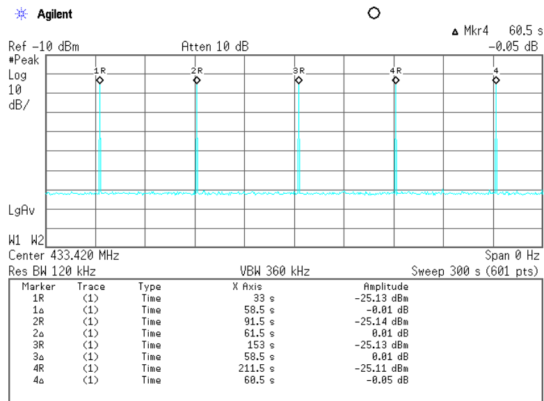
Plot 7.1.6 Polling / supervision transmission period
