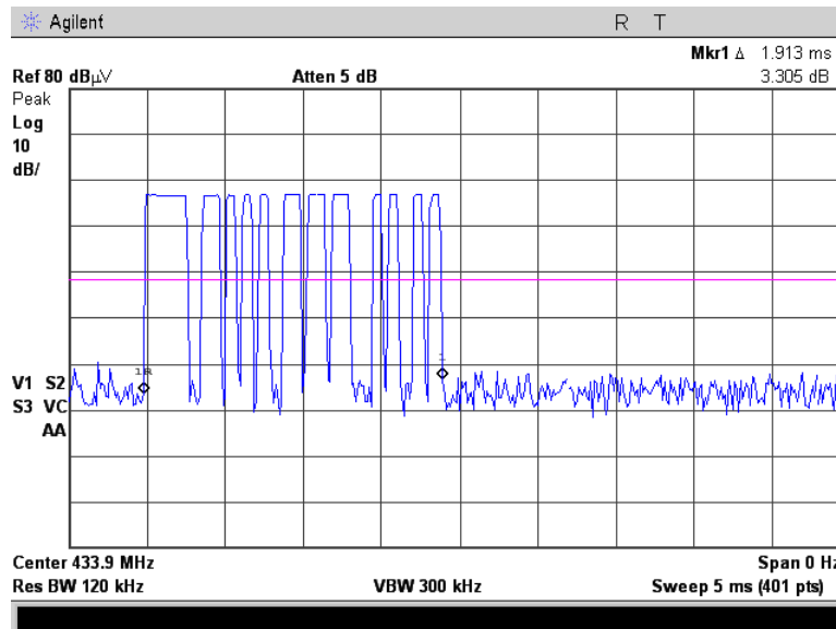
Plot 7.2.12 Transmission pulse period
