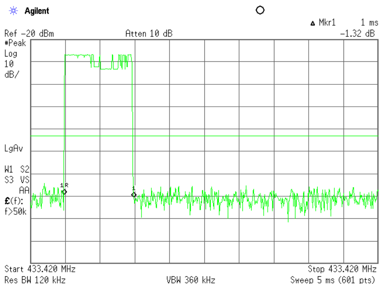
Plot 7.1.5 Polling / supervision transmission duration
