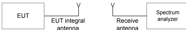
Figure 7.2.1 Setup for transmitter shut down test
