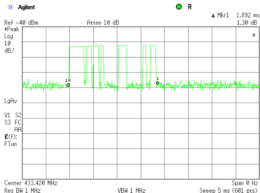
Plot 7.2.3 Supervision transmission duration
