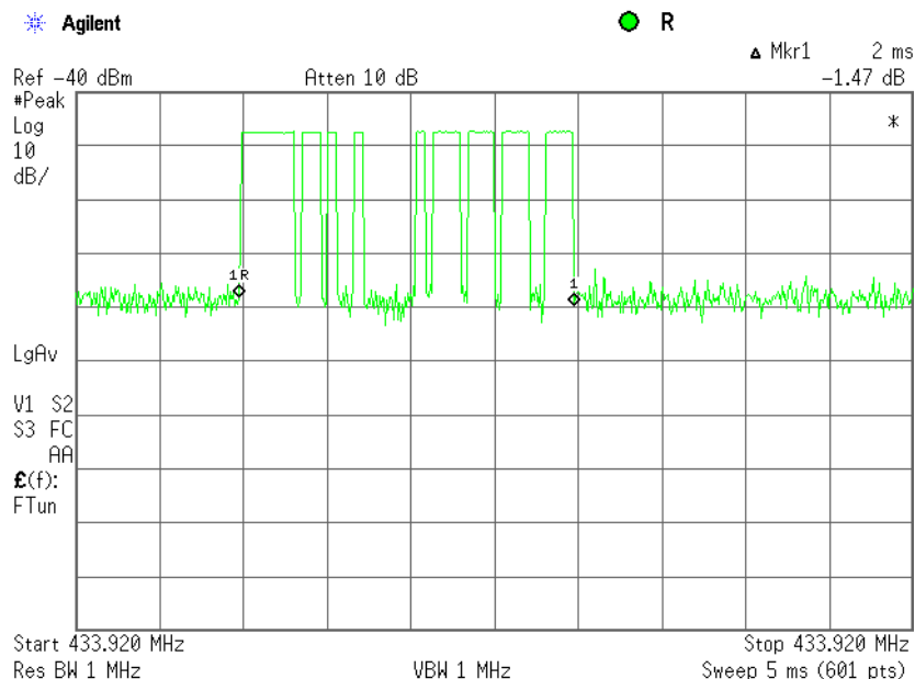
Plot 7.1.3 Supervision transmission duration
