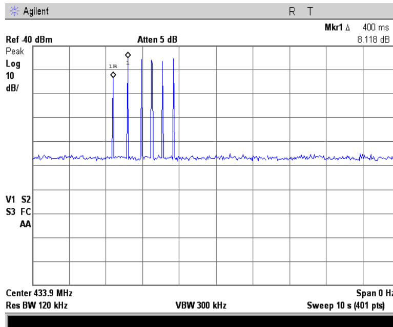
Plot 7.1.2 Transmission burst period
