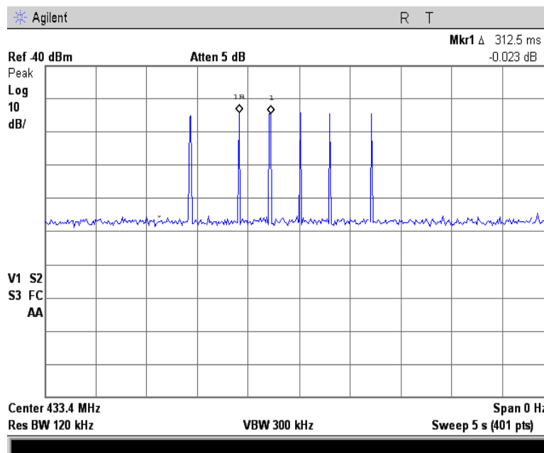
Plot 7.4.14 Transmission burst period
