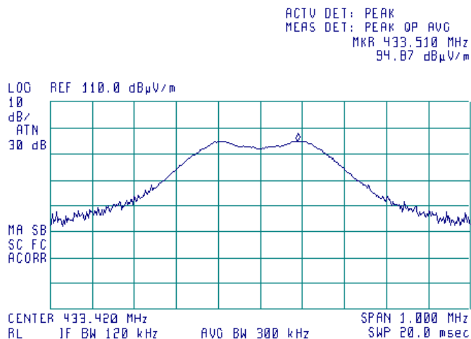
Plot 7.3.2 Radiated emission measurements at the fundamental frequency
