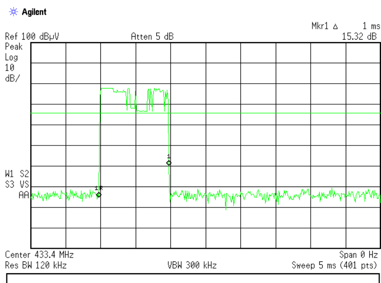
Plot 7.3.15 Transmission pulse period
