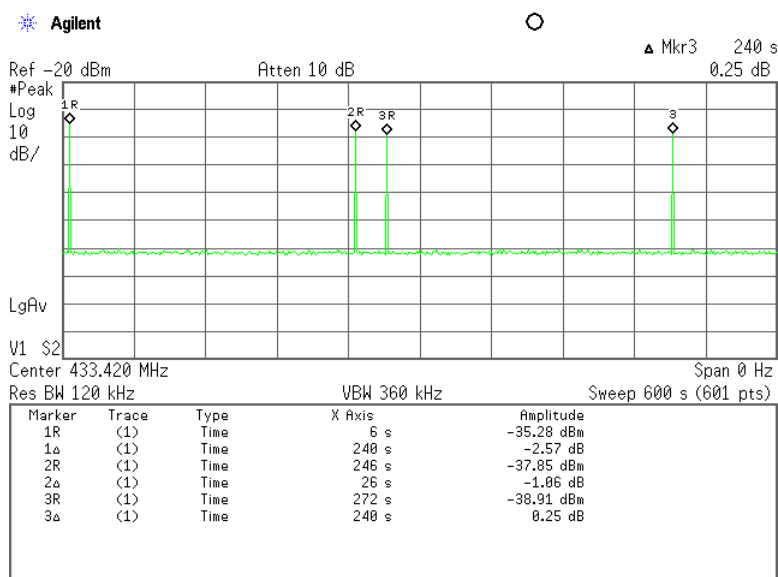
Plot 7.1.3 Polling / supervision transmissions during 10 min period
