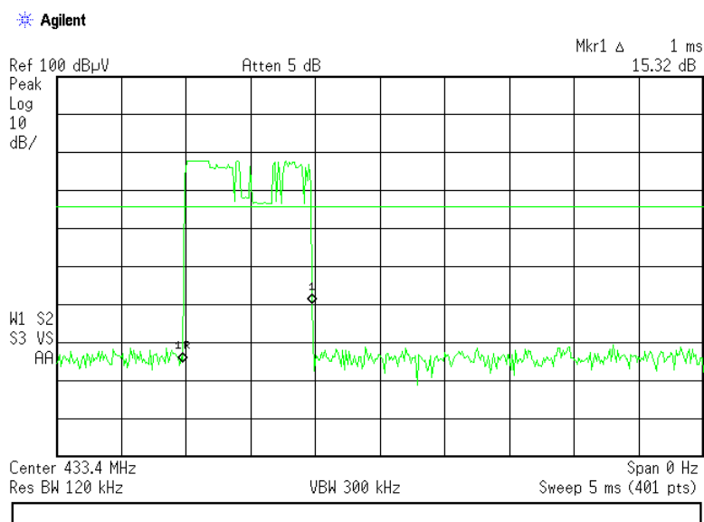
Plot 7.2.15 Transmission pulse period
