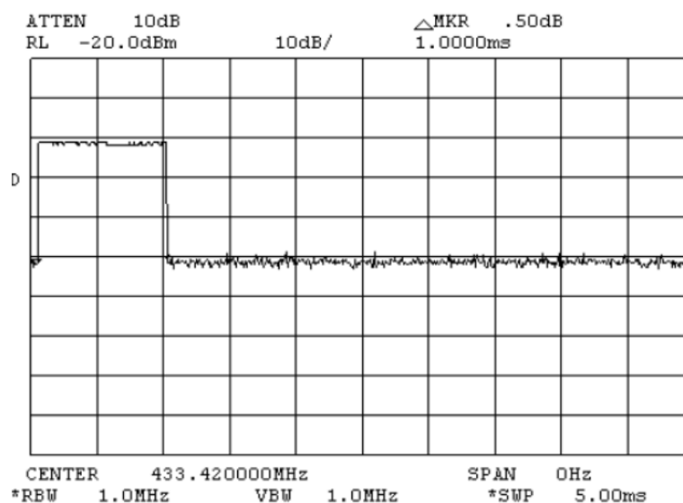
Plot 7.1.3 Polling / supervision transmission duration
