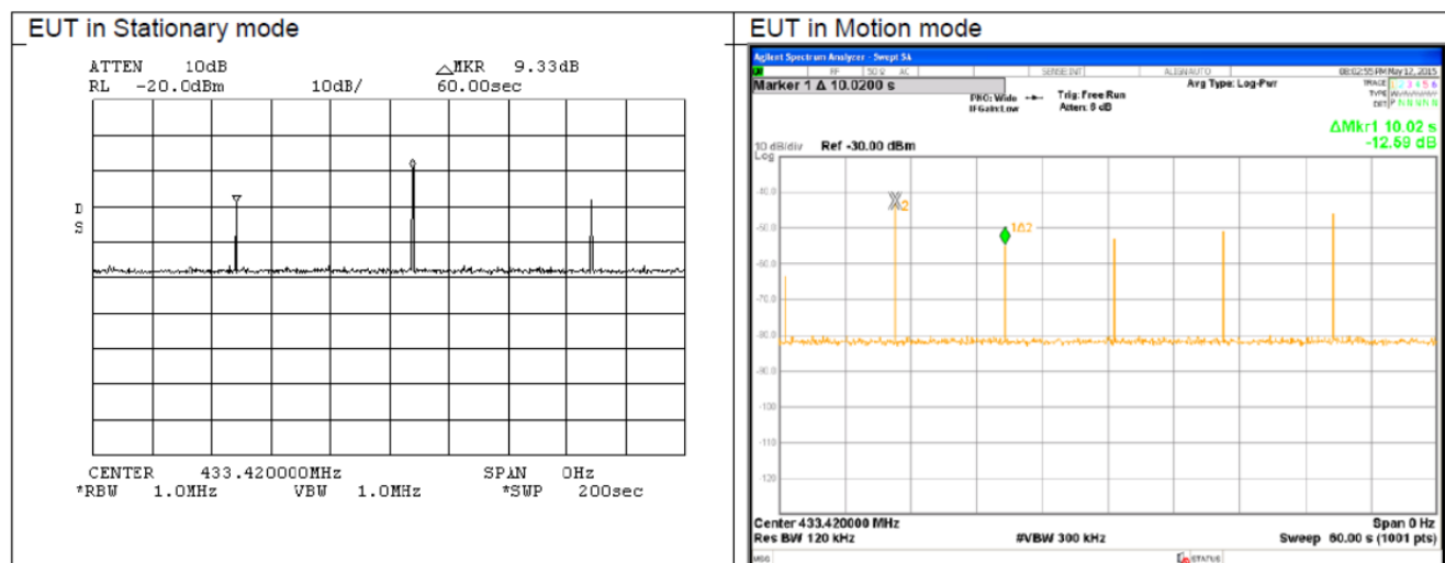
Plot 7.1.3 Polling / supervision transmission duration
