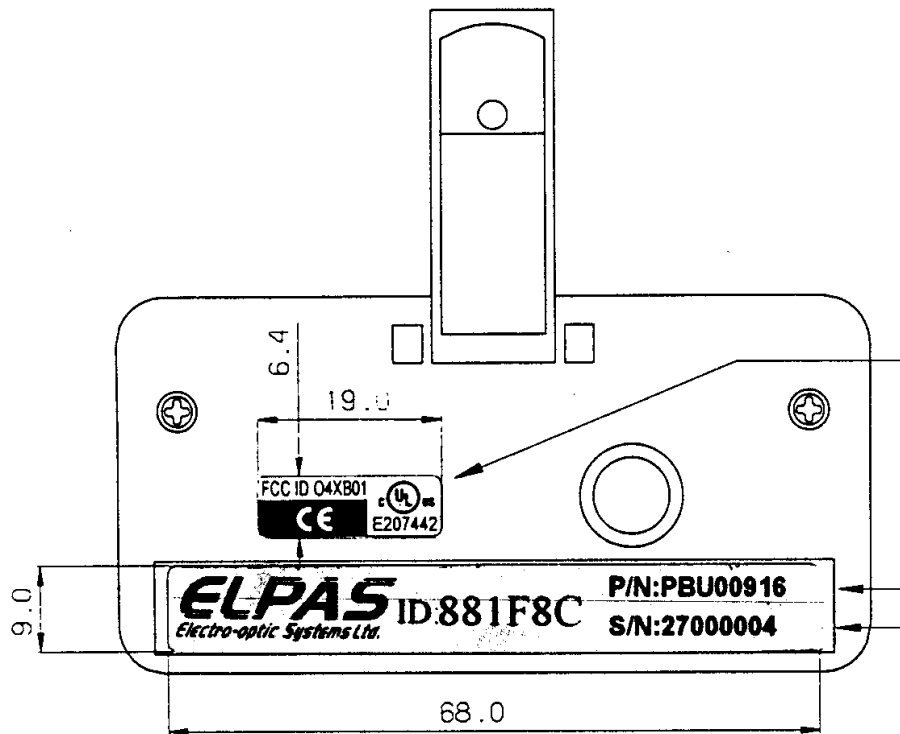
FCC Label
