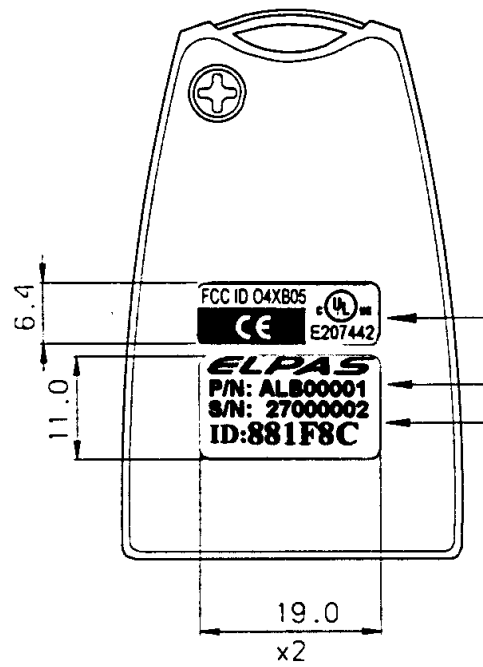
FCC Label
