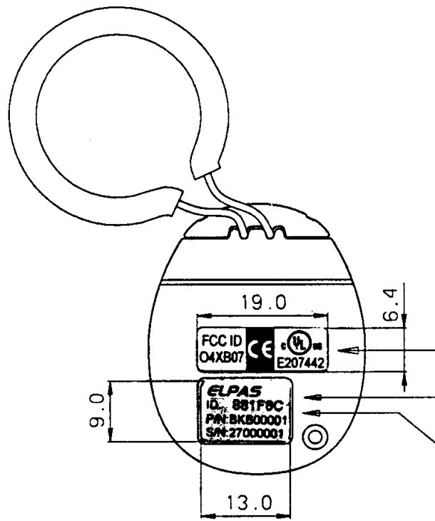
FCC Label
