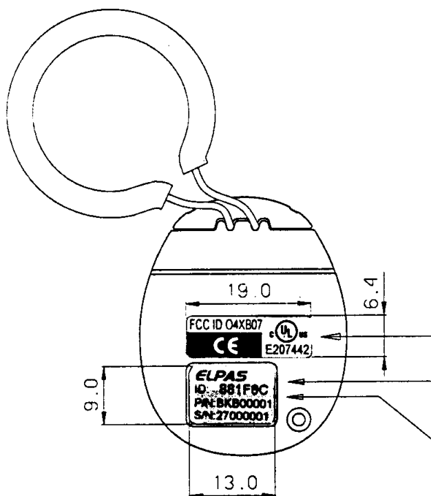
FCC Label
