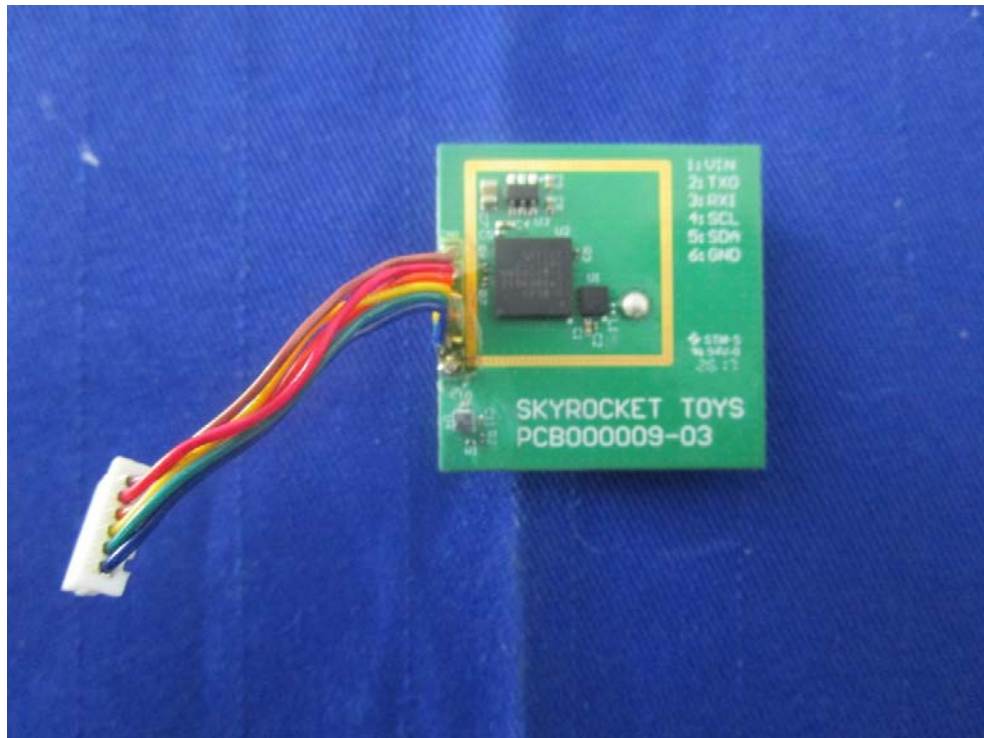
EUT – Board Bottom View
