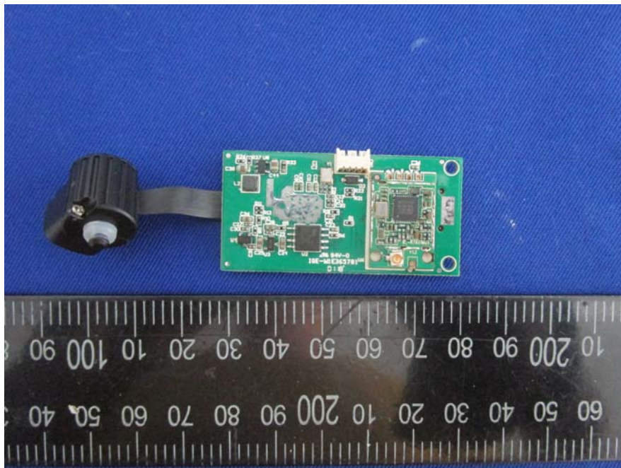
EUT – Camera Board Top Unshielded View
