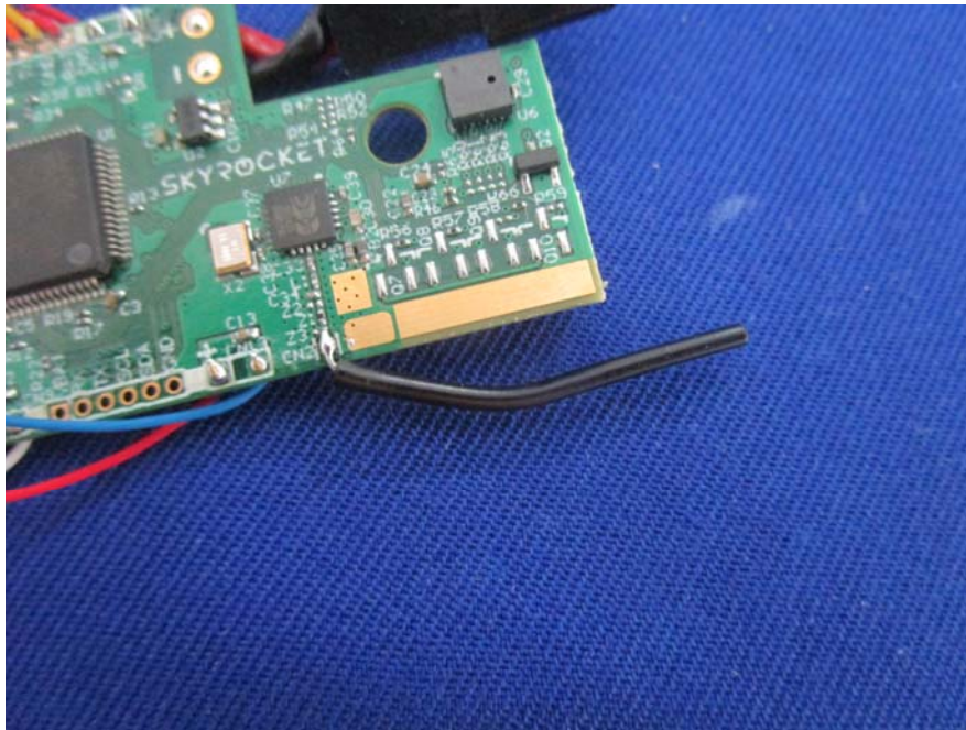
EUT – 2.4G SDR Antenna View
