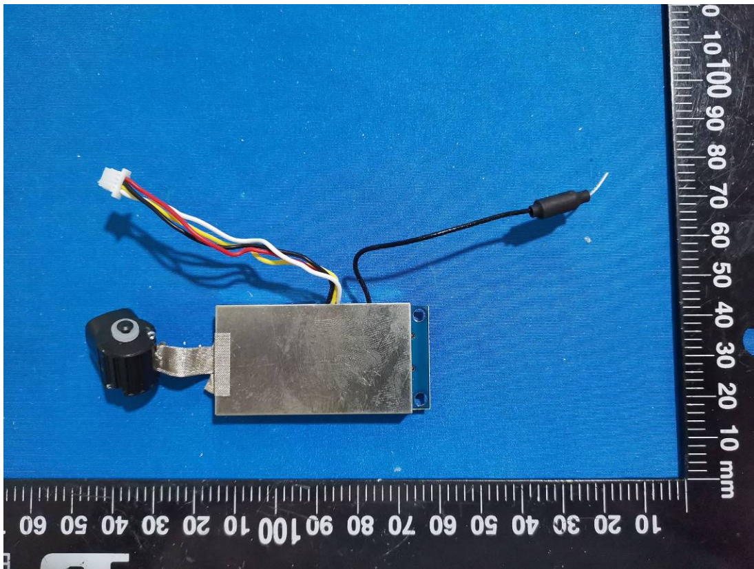
WiFi Board And Antenna
