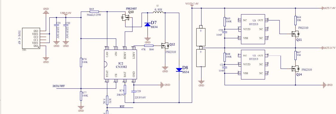
electronic switch/LDO
