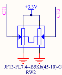
Universal potentiometer
