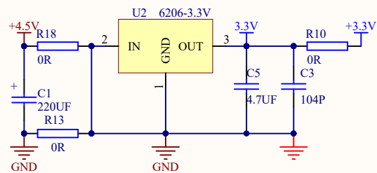
Voltage regulator circuit
