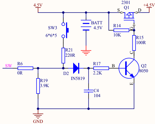
Switchgear circuit
