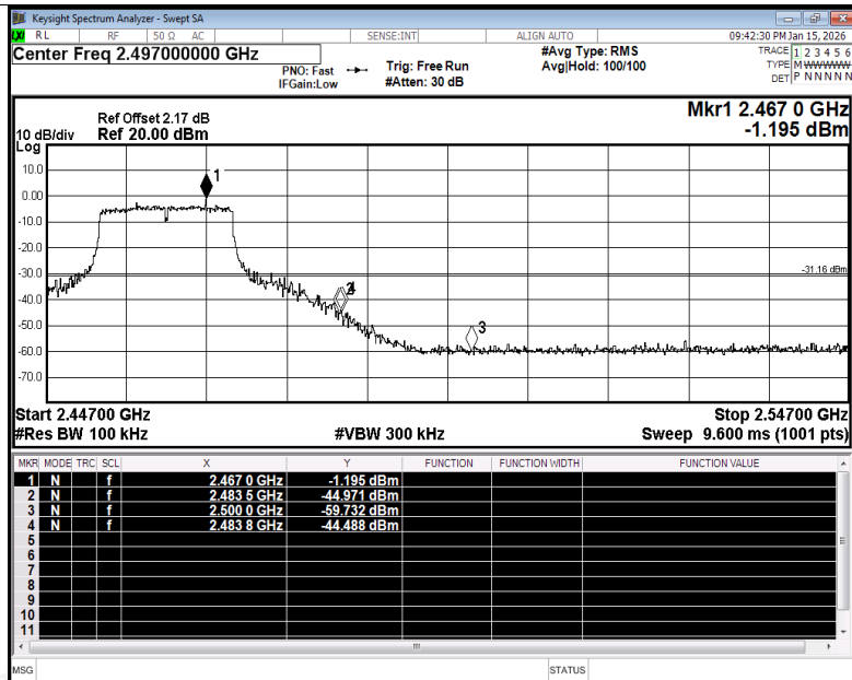
Band Edge NVNT g 2462MHz Ant1 Emission
