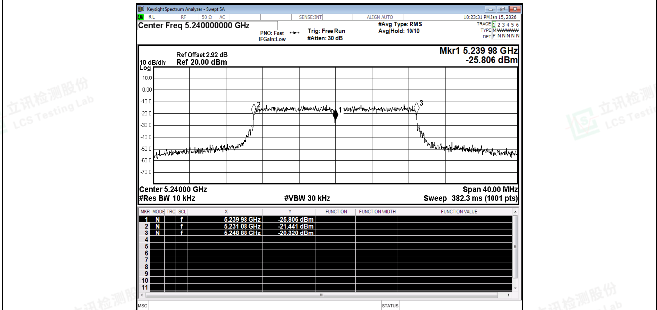
Freq. Stability NVNT n20 5240MHz Ant1
