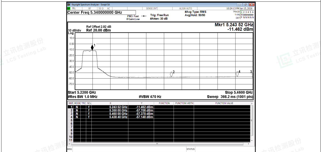
Restrict Band NVNT n20 5240MHz Ant1 Average
