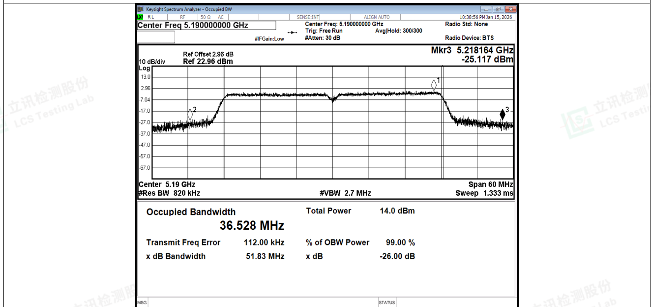
-26dB Bandwidth NVNT ac40 5190MHz Ant1
