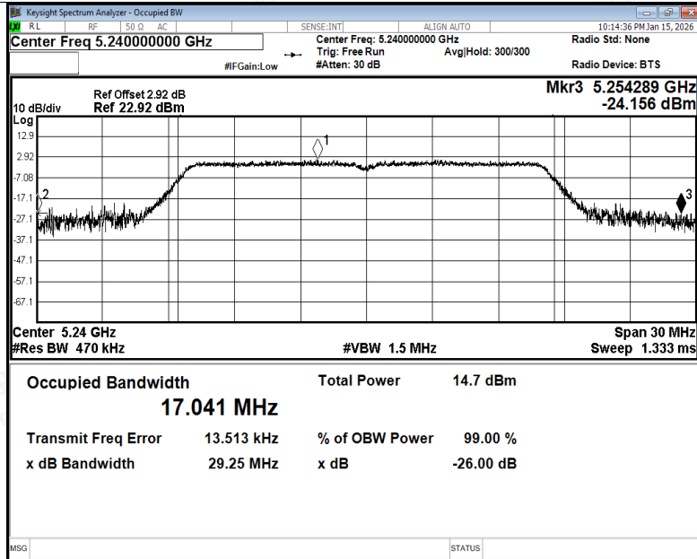
-26dB Bandwidth NVNT a 5240MHz Ant1
