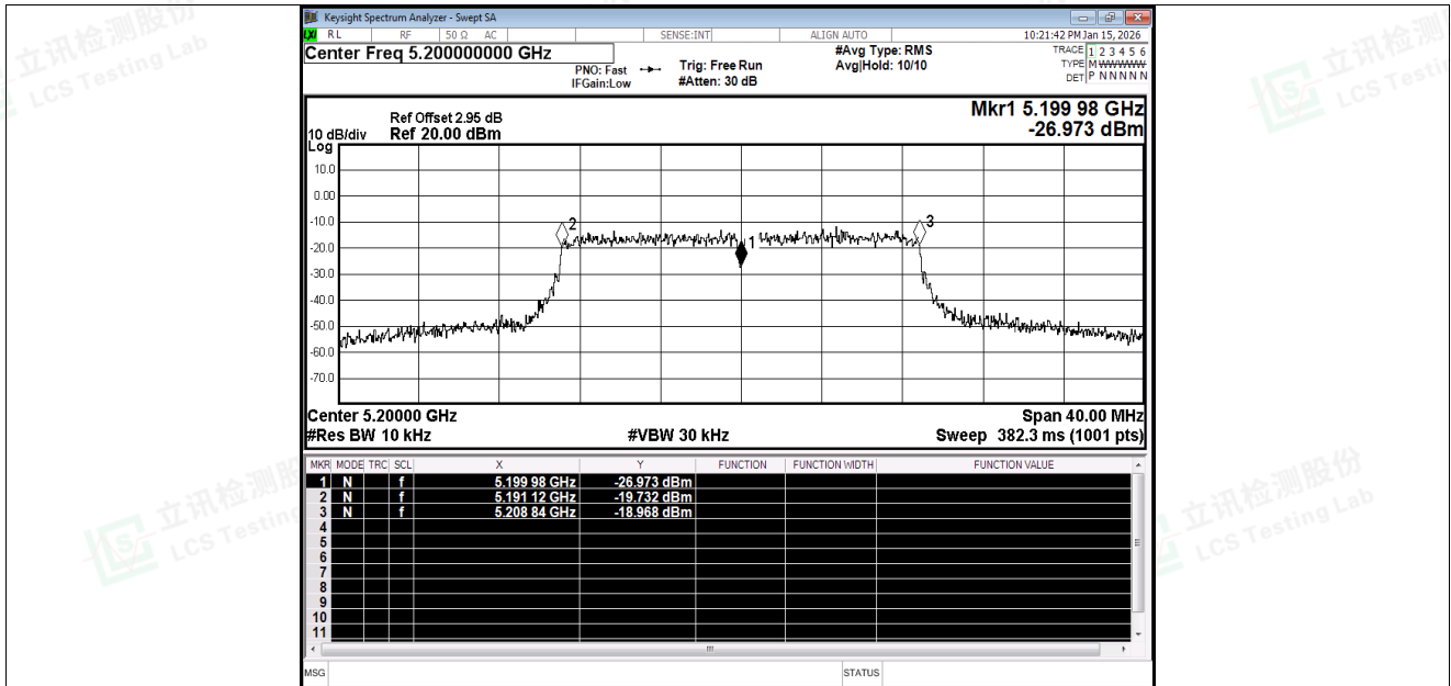
Freq. Stability NVNT n20 5200MHz Ant1
