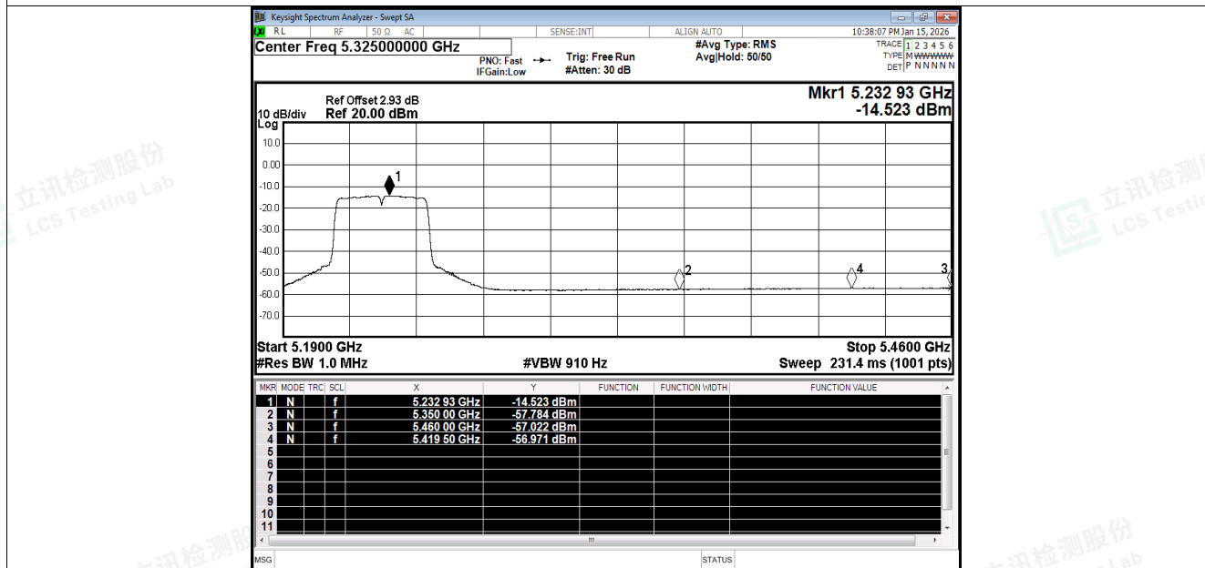
Restrict Band NVNT n40 5230MHz Ant1 Average
