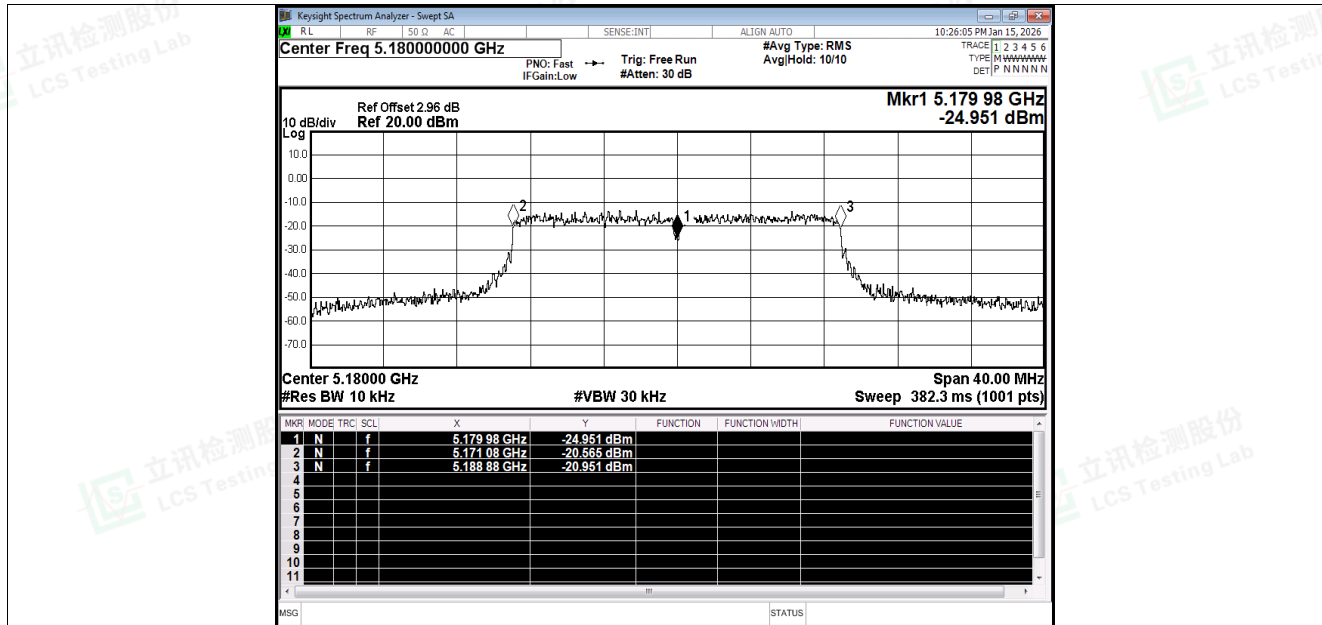
Freq. Stability NVNT ac20 5180MHz Ant1
