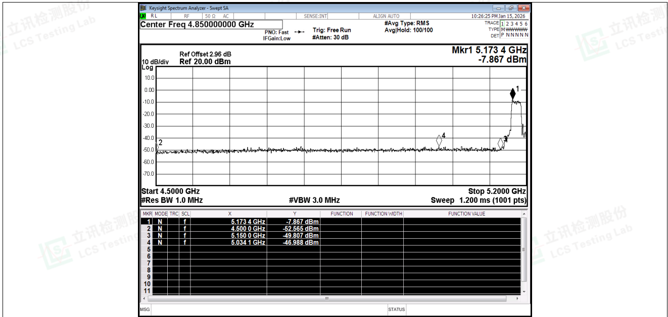
Restrict Band NVNT ac20 5180MHz Ant1 Peak
