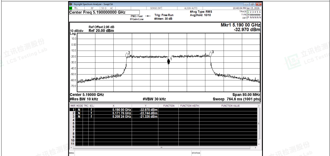
Freq. Stability NVNT ac40 5190MHz Ant1
