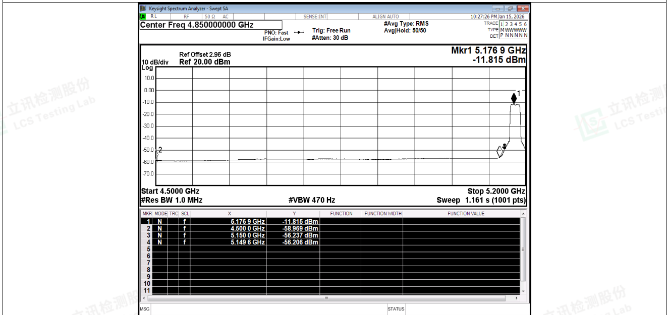
Restrict Band NVNT ac20 5180MHz Ant1 Average
