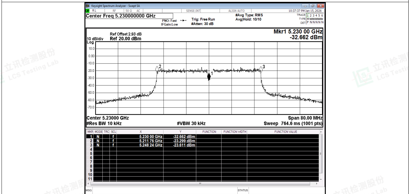
Freq. Stability NVNT n40 5230MHz Ant1
