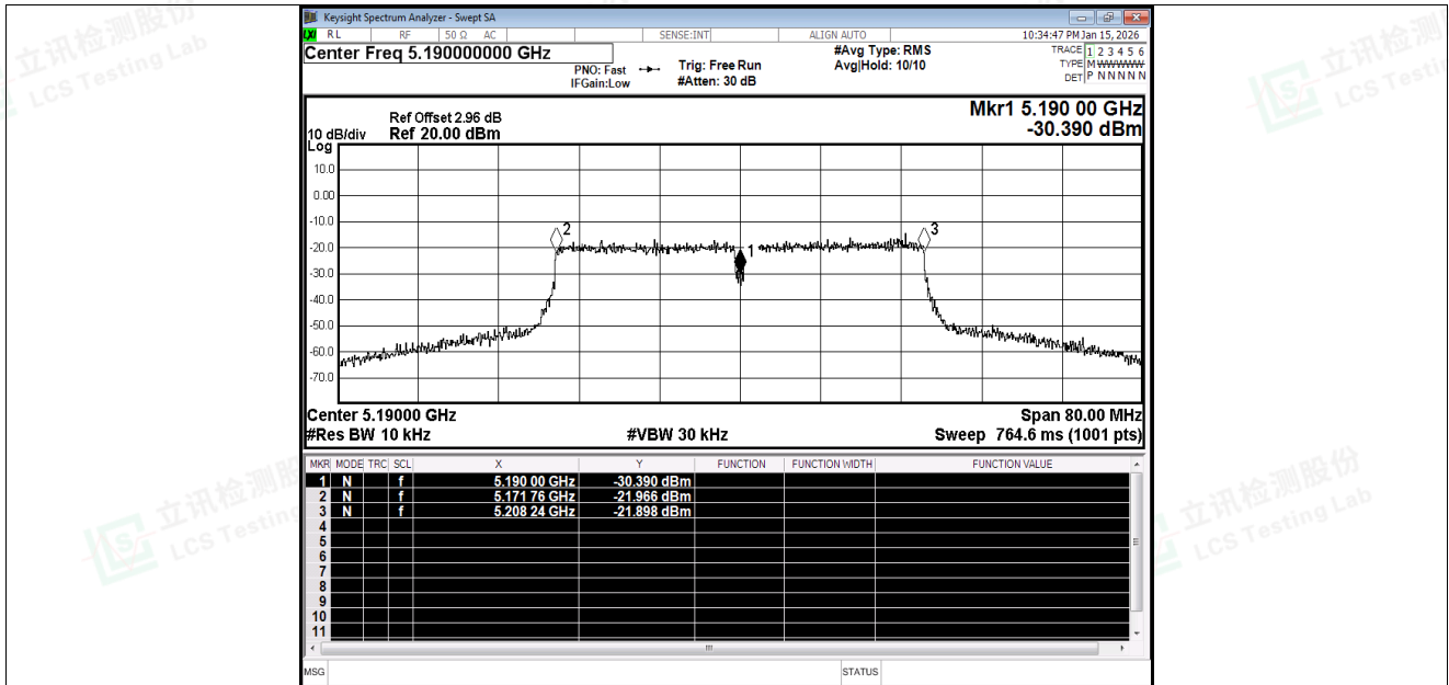
Freq. Stability NVNT n40 5190MHz Ant1
