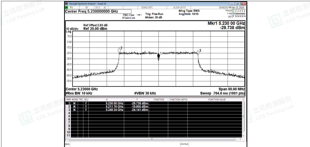
Freq. Stability NVNT ac40 5230MHz Ant1
