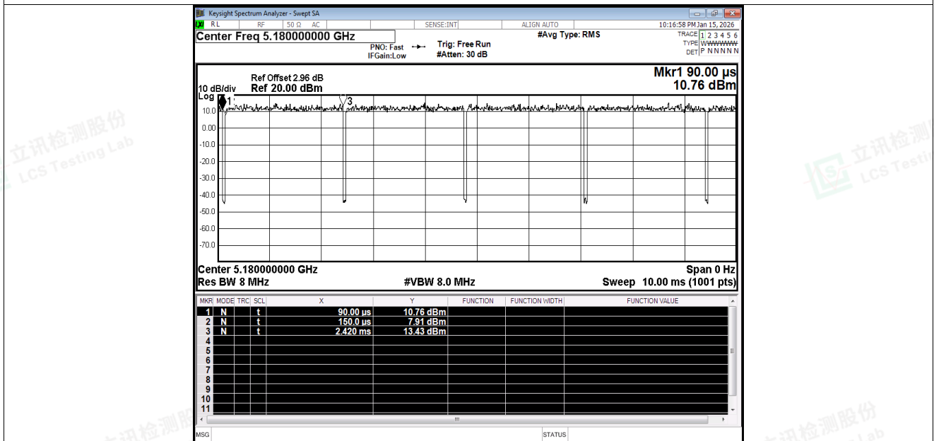
Duty Cycle NVNT n20 5180MHz Ant1
