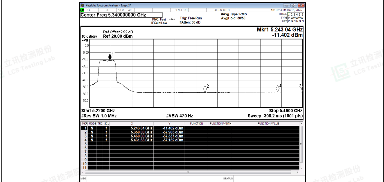
Restrict Band NVNT ac20 5240MHz Ant1 Average
