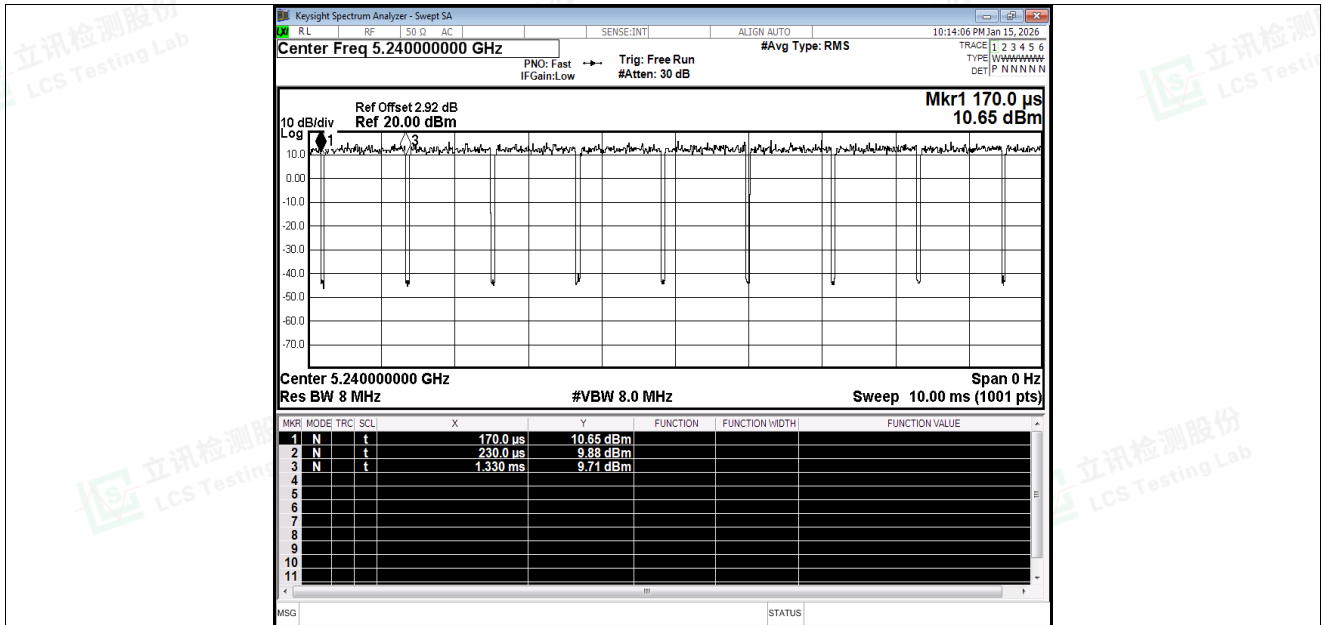
Duty Cycle NVNT a 5240MHz Ant1
