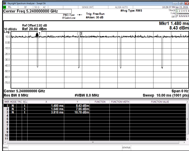
Duty Cycle NVNT ac20 5240MHz Ant1
