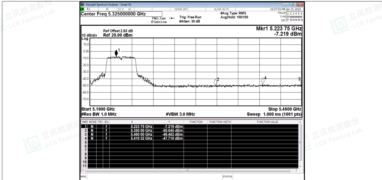
Restrict Band NVNT n40 5230MHz Ant1 Peak
