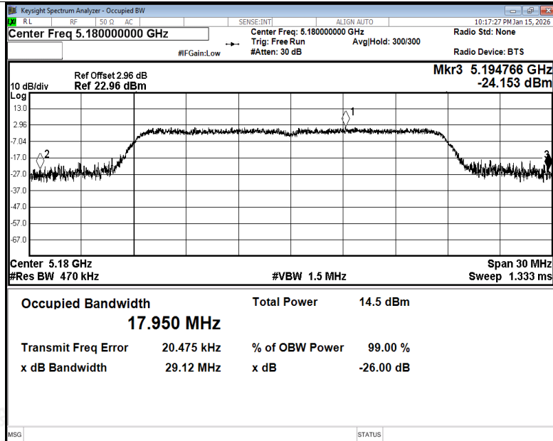
-26dB Bandwidth NVNT n20 5180MHz Ant1
