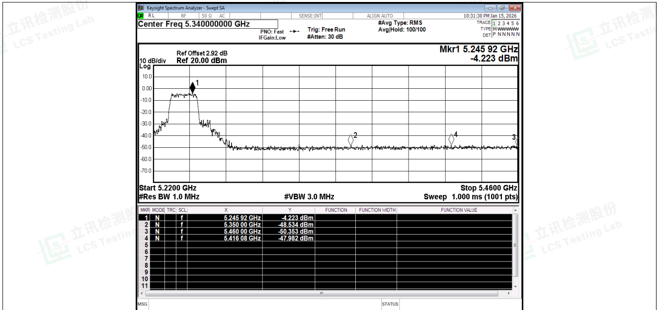
Restrict Band NVNT ac20 5240MHz Ant1 Peak
