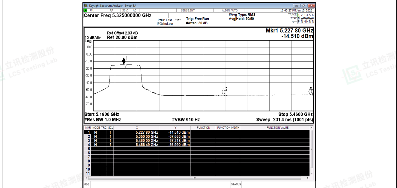
Restrict Band NVNT ac40 5230MHz Ant1 Average
