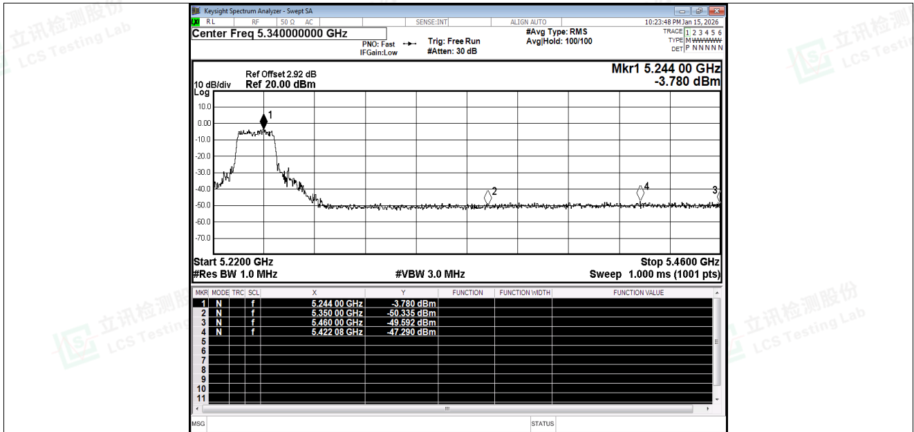
Restrict Band NVNT n20 5240MHz Ant1 Peak
