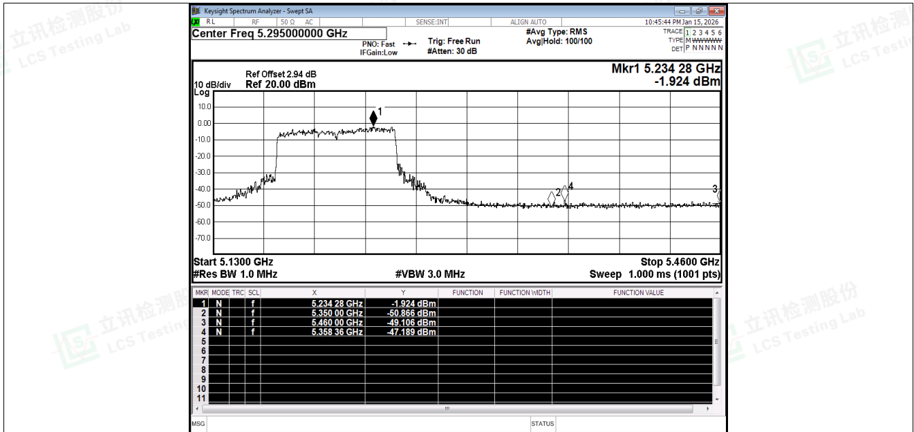
Restrict Band NVNT ac80 5210MHz Ant1 Peak
