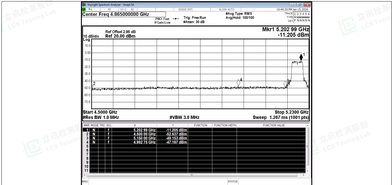
Restrict Band NVNT ac40 5190MHz Ant1 Peak
