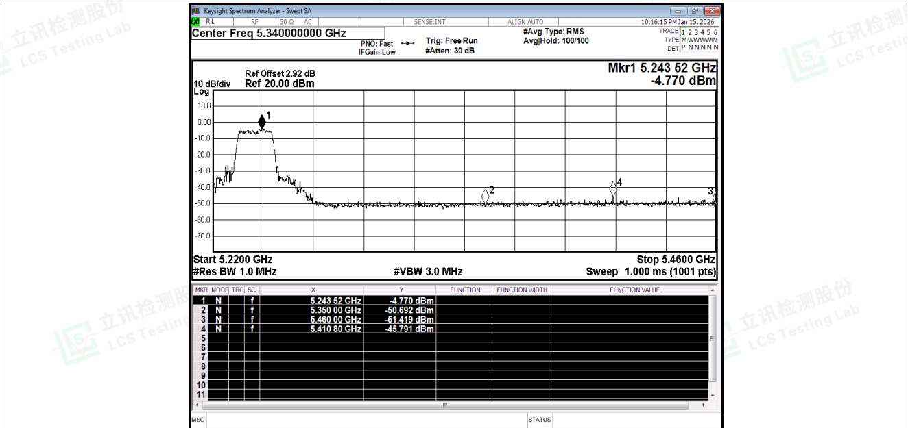
Restrict Band NVNT a 5240MHz Ant1 Peak
