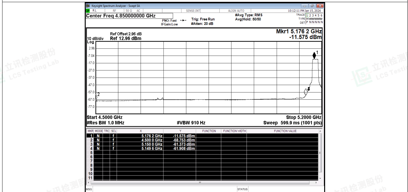
Restrict Band NVNT a 5180MHz Ant1 Average
