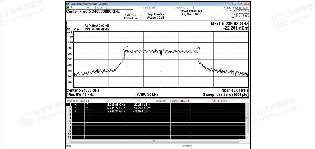
Freq. Stability NVNT a 5240MHz Ant1
