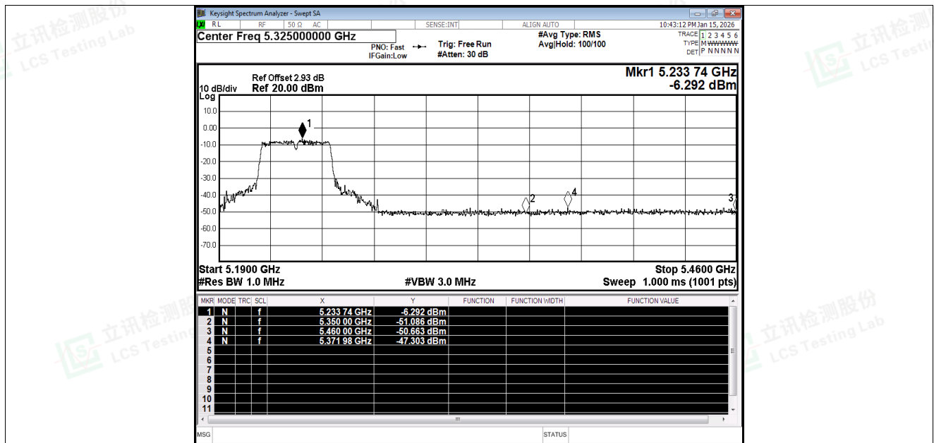
Restrict Band NVNT ac40 5230MHz Ant1 Peak
