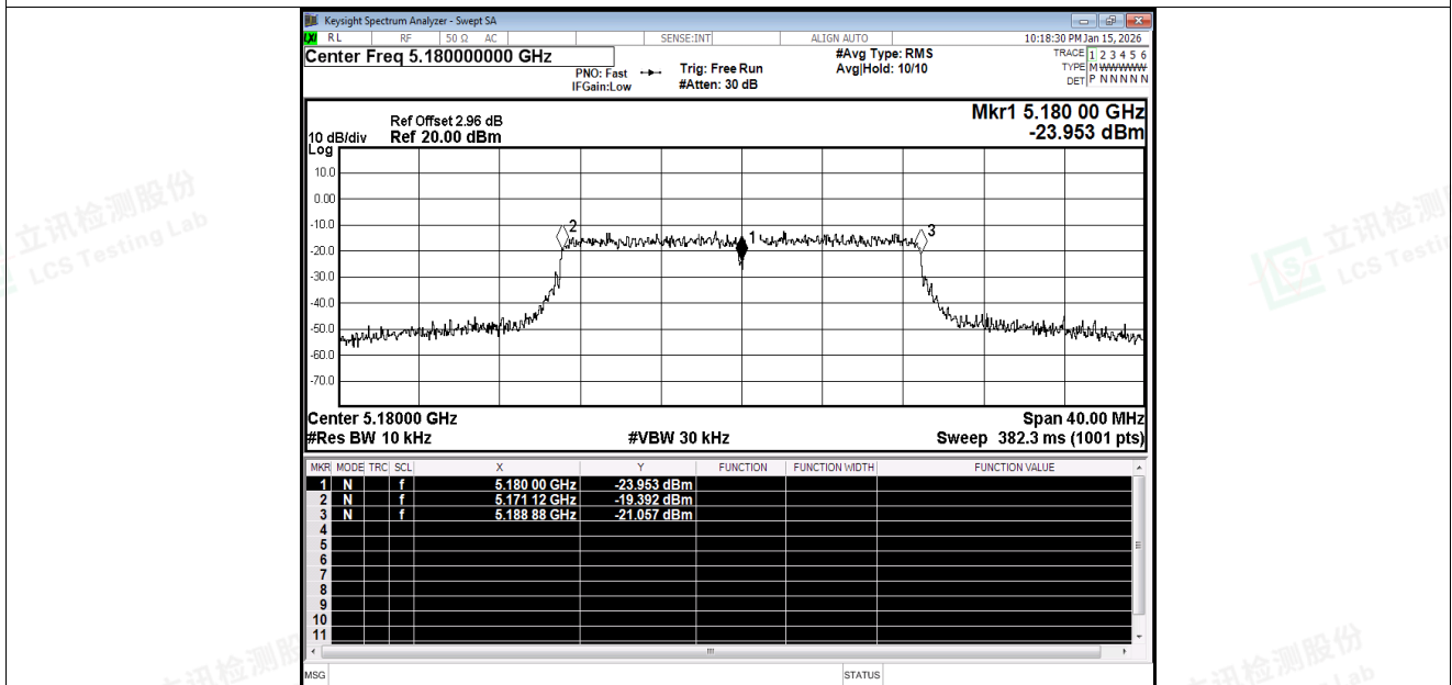
Freq. Stability NVNT n20 5180MHz Ant1
