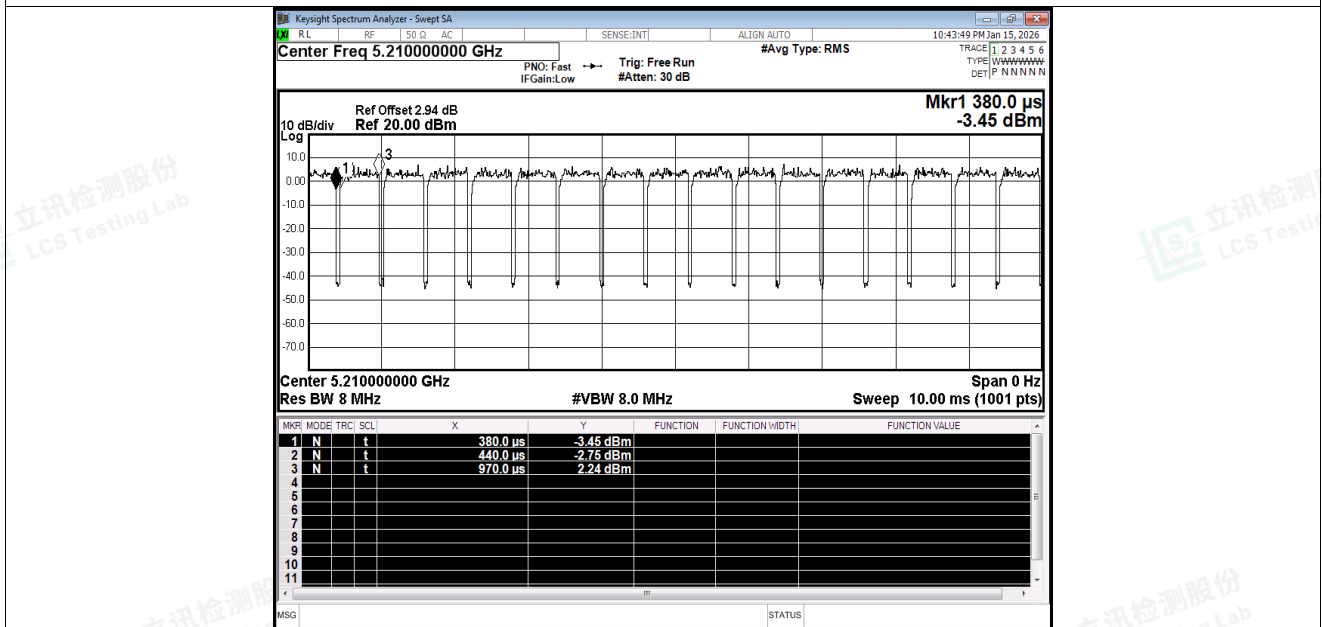
Duty Cycle NVNT ac80 5210MHz Ant1
