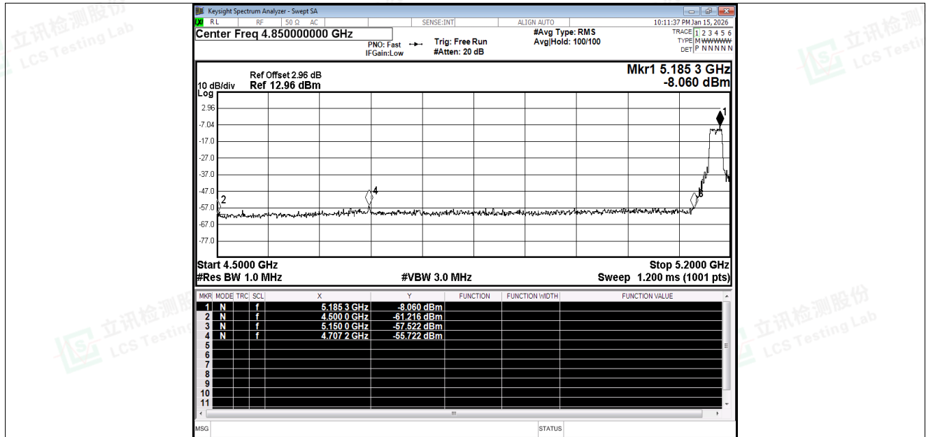
Restrict Band NVNT a 5180MHz Ant1 Peak
