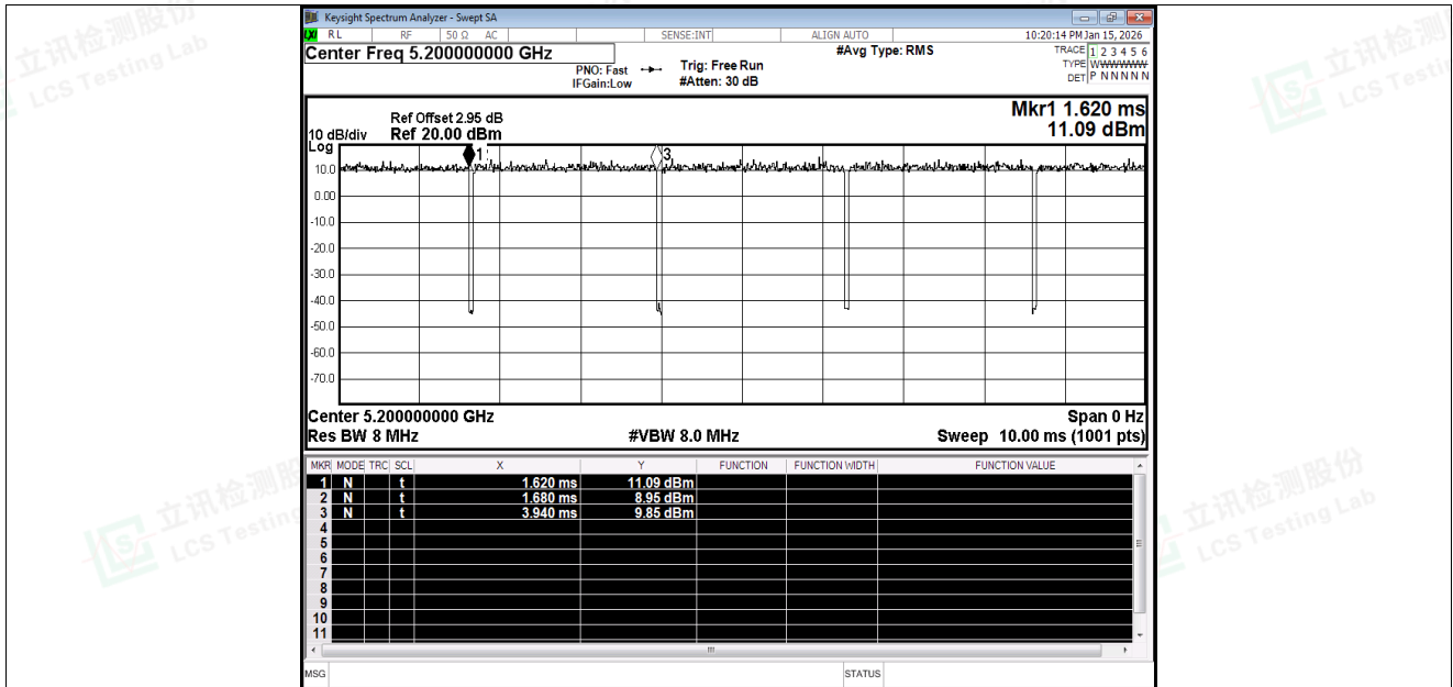
Duty Cycle NVNT n20 5200MHz Ant1
