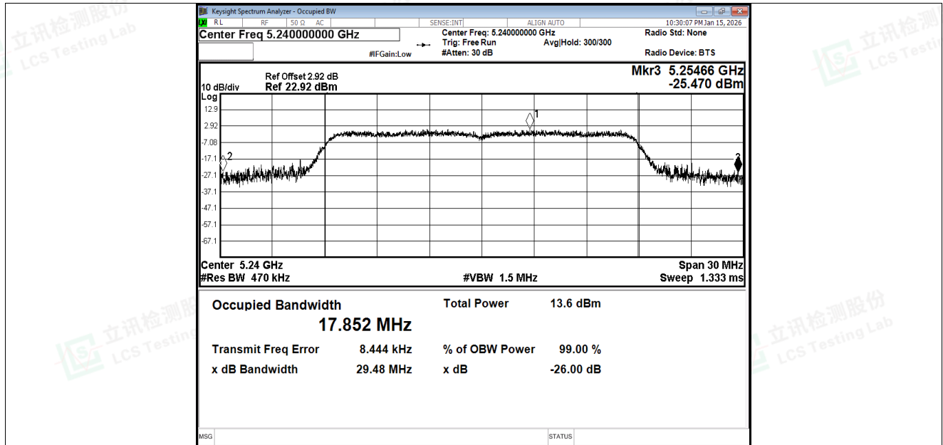
-26dB Bandwidth NVNT ac20 5240MHz Ant1
