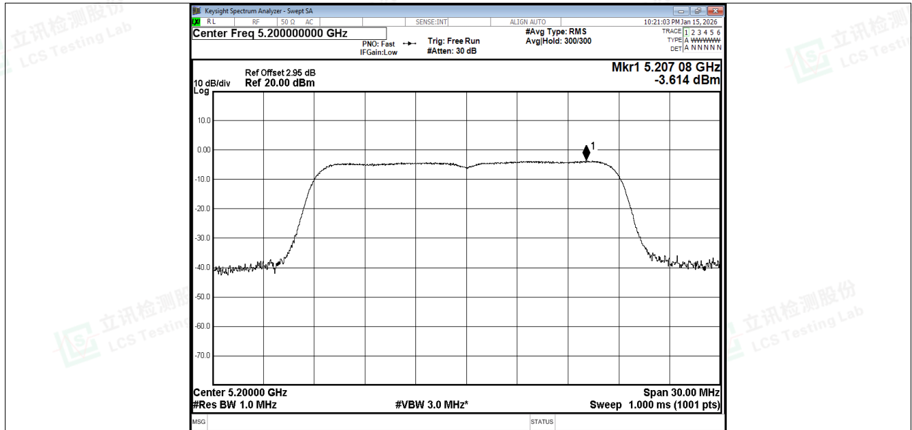
PSD NVNT n20 5200MHz Ant1
