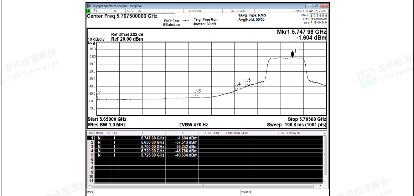
Restrict Band NVNT n20 5745MHz Ant1 Average
