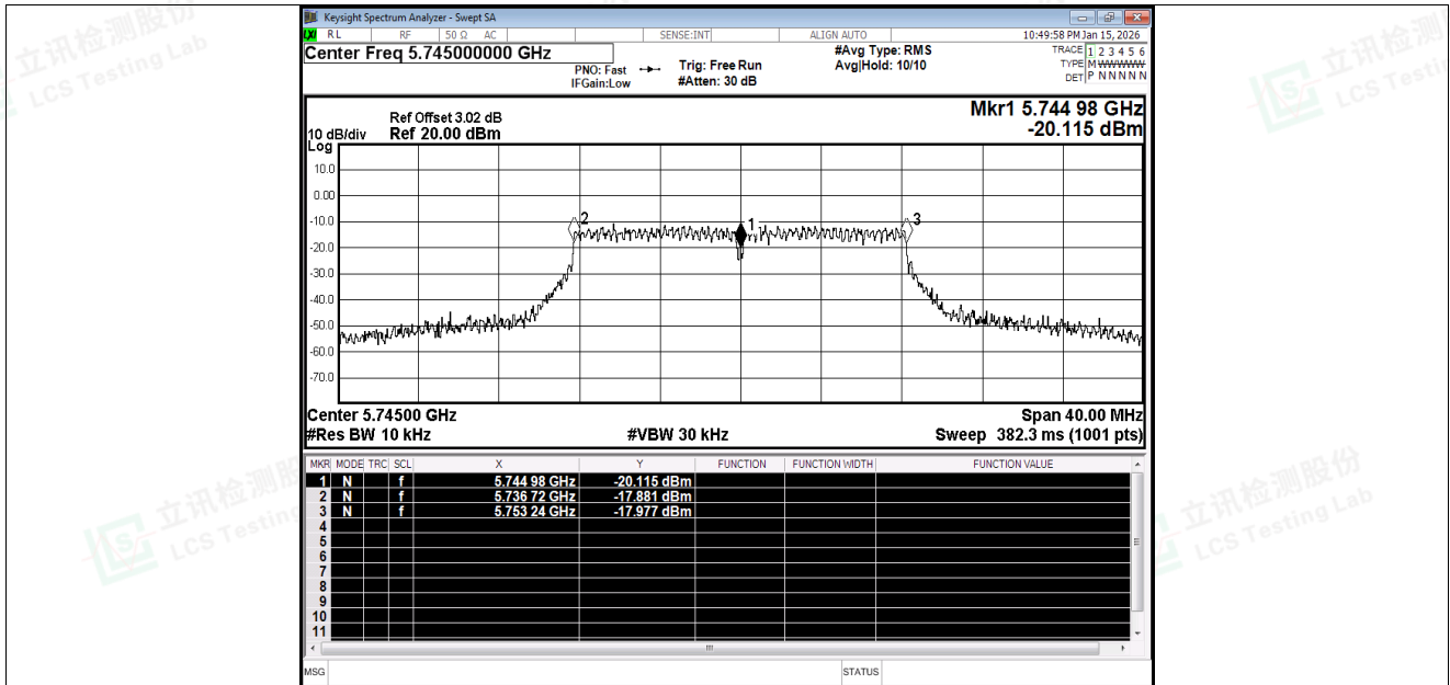
Freq. Stability NVNT a 5745MHz Ant1
