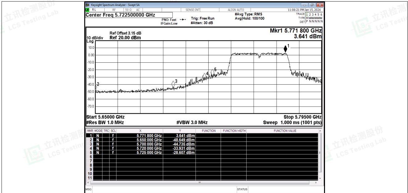
Restrict Band NVNT n40 5755MHz Ant1 Peak
