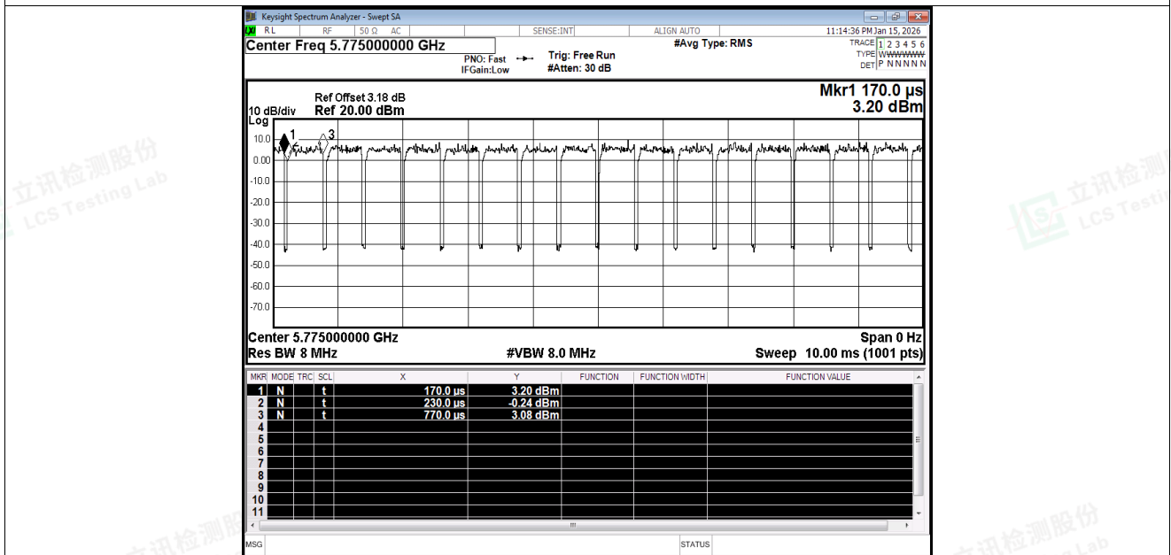
Duty Cycle NVNT ac80 5775MHz Ant1
