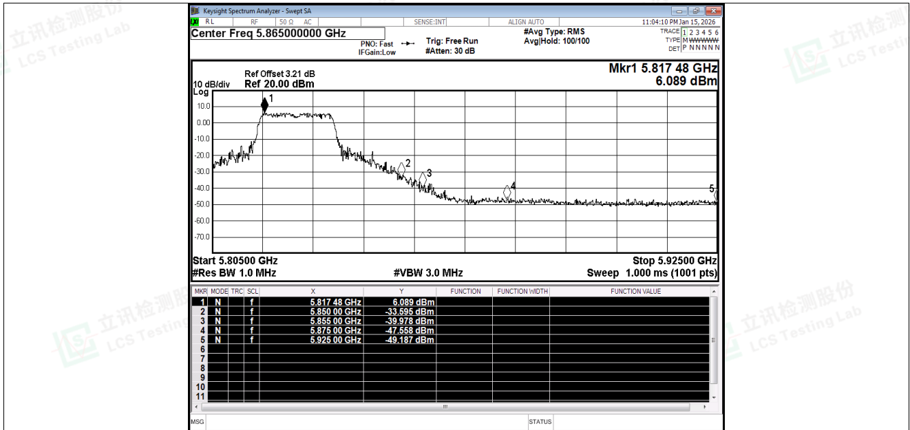
Restrict Band NVNT ac20 5825MHz Ant1 Peak
