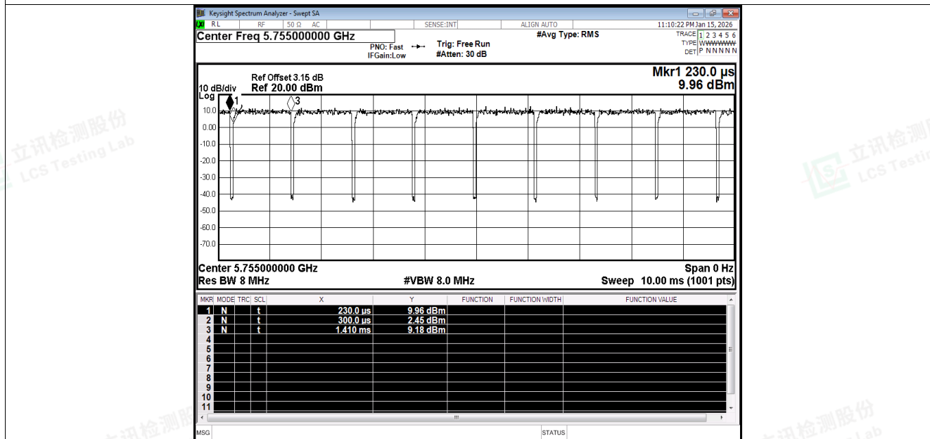
Duty Cycle NVNT ac40 5755MHz Ant1
