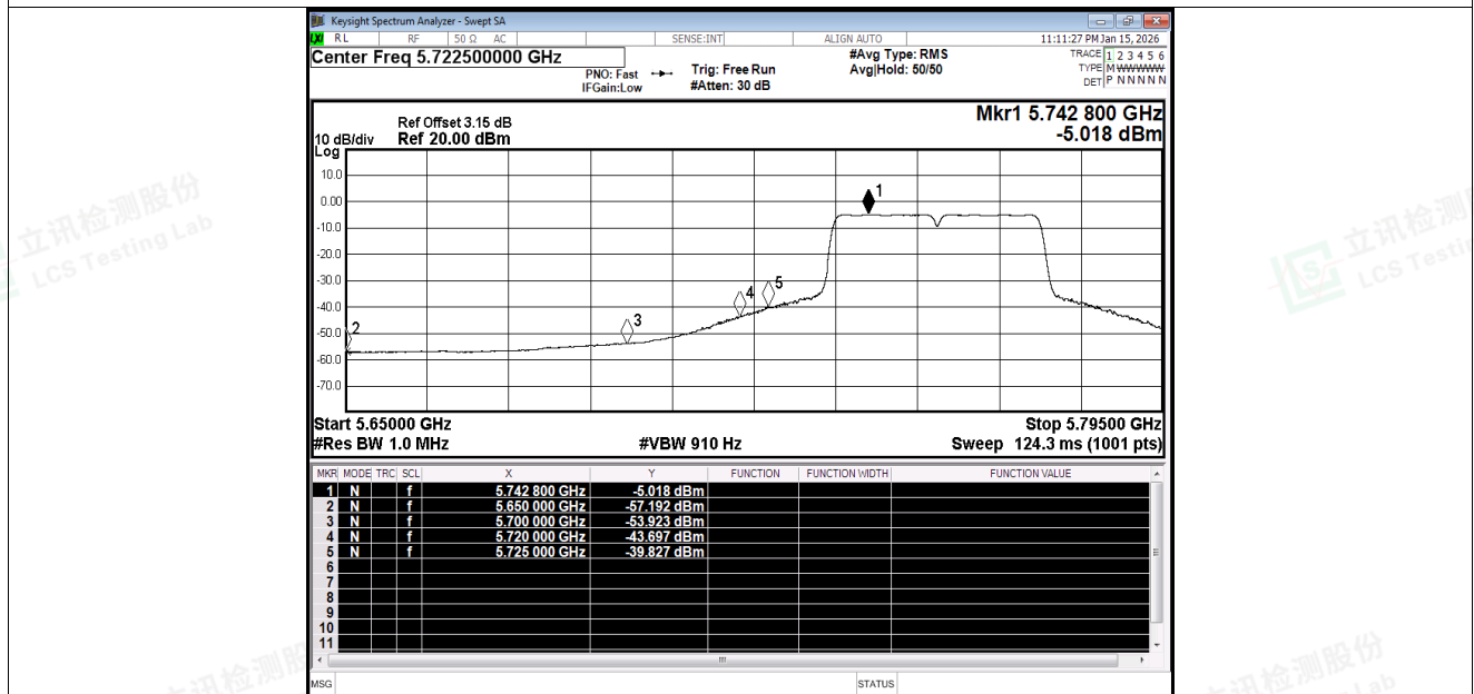
Restrict Band NVNT ac40 5755MHz Ant1 Average
