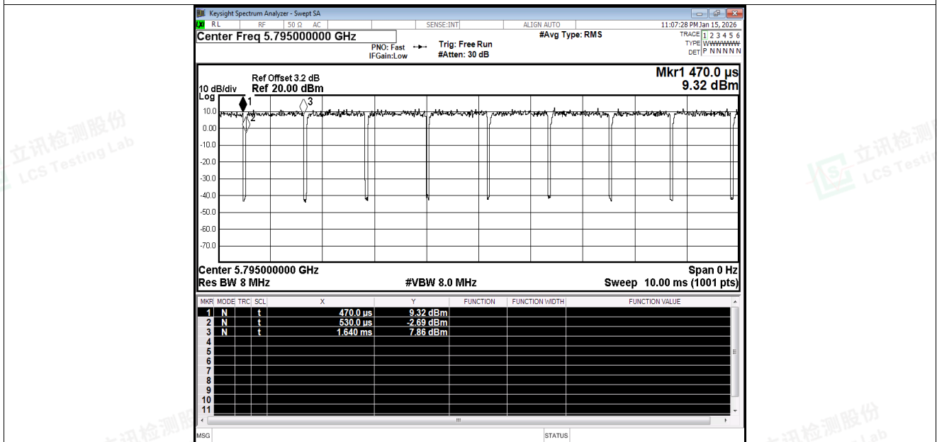
Duty Cycle NVNT n40 5795MHz Ant1
