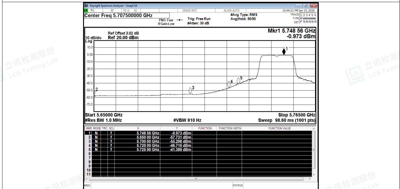
Restrict Band NVNT a 5745MHz Ant1 Average
