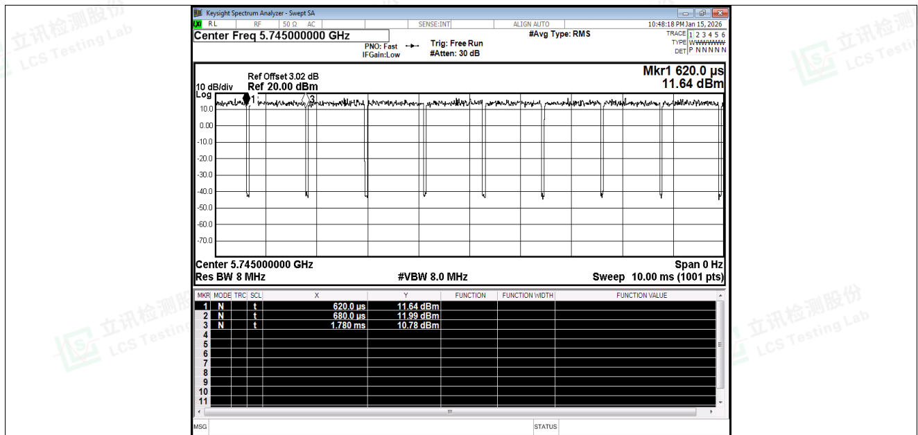
Duty Cycle NVNT a 5745MHz Ant1
