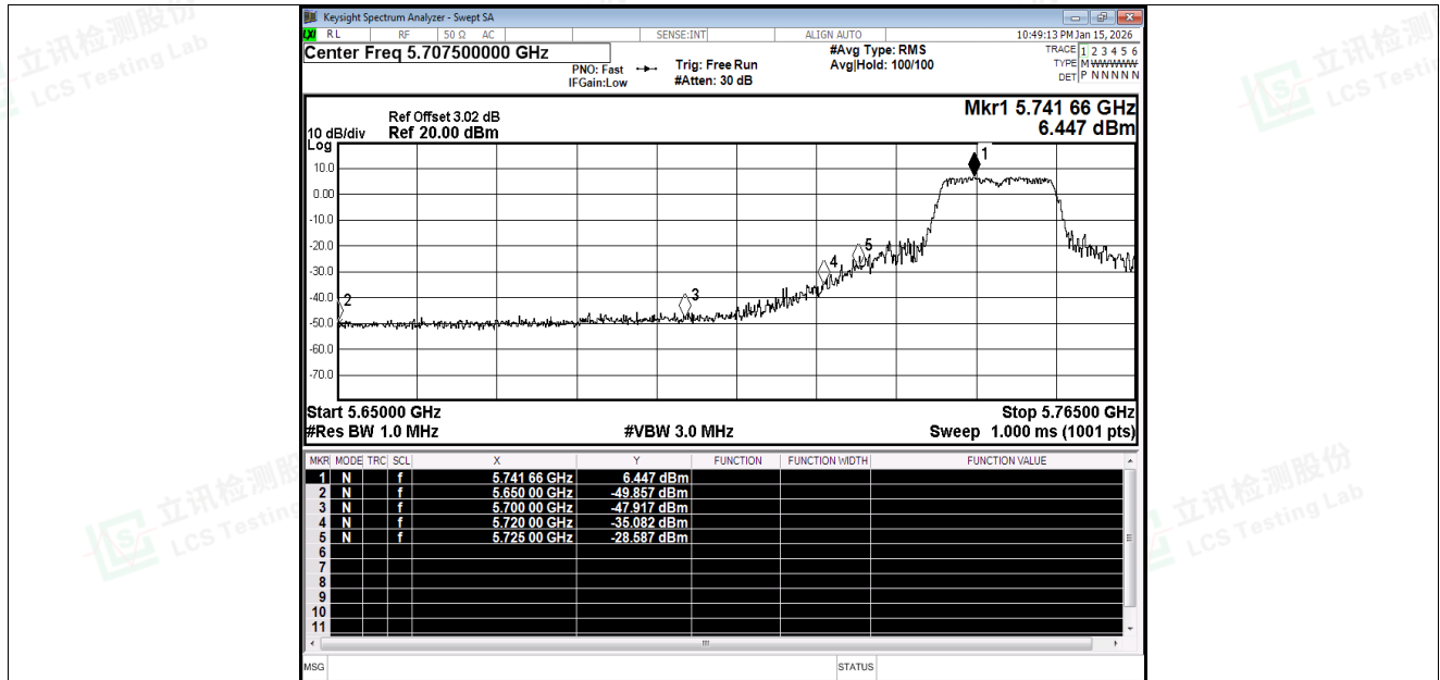
Restrict Band NVNT a 5745MHz Ant1 Peak
