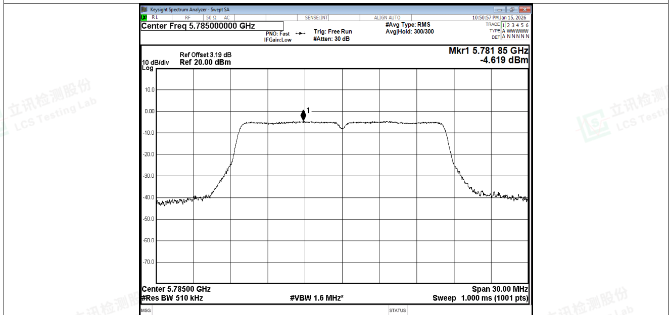
PSD NVNT a 5785MHz Ant1
