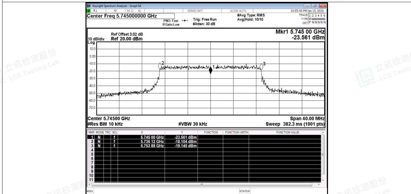
Freq. Stability NVNT n20 5745MHz Ant1
