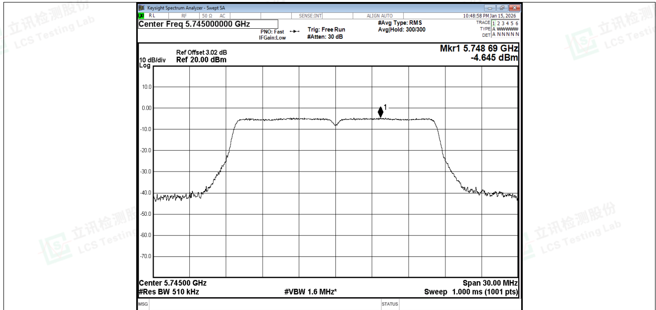
PSD NVNT a 5745MHz Ant1
