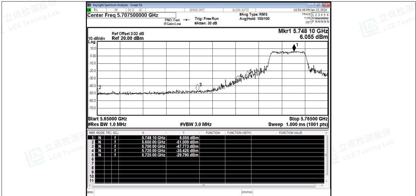
Restrict Band NVNT n20 5745MHz Ant1 Peak
