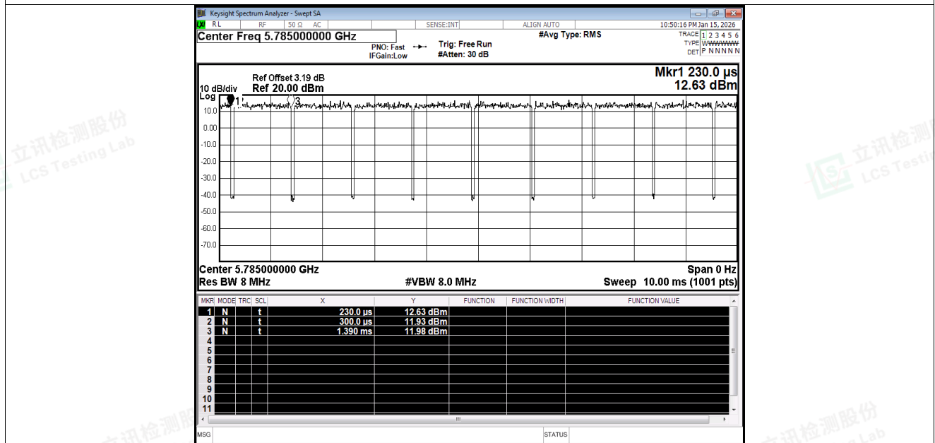
Duty Cycle NVNT a 5785MHz Ant1
