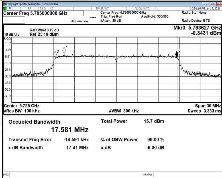
-6dB Bandwidth NVNT n20 5785MHz Ant1
