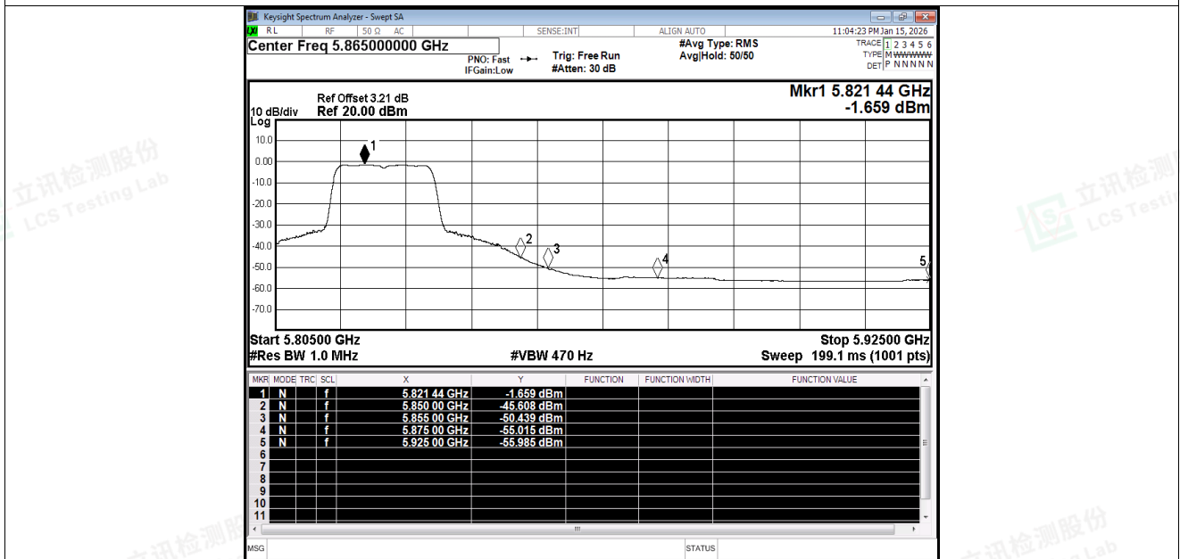
Restrict Band NVNT ac20 5825MHz Ant1 Average
