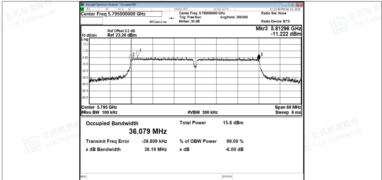
-6dB Bandwidth NVNT ac40 5795MHz Ant1
