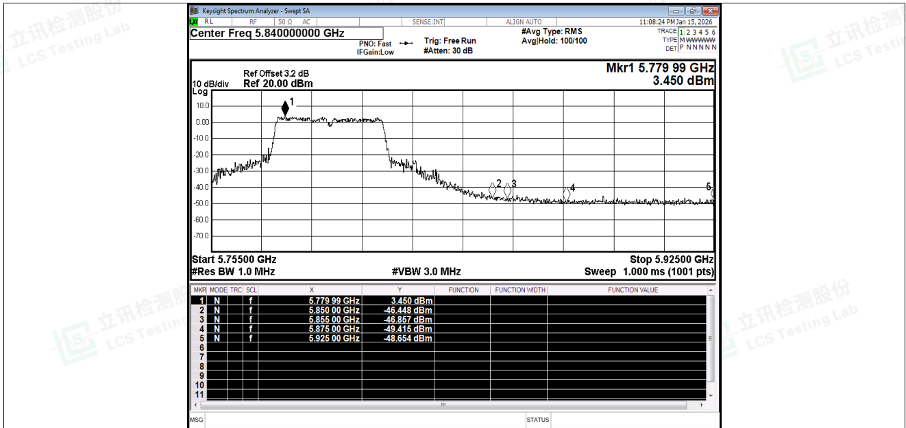
Restrict Band NVNT n40 5795MHz Ant1 Peak
