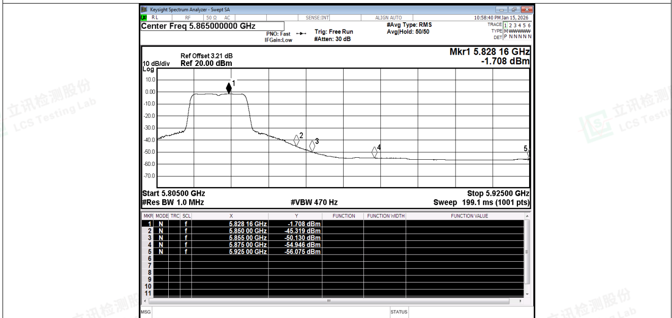
Restrict Band NVNT n20 5825MHz Ant1 Average
