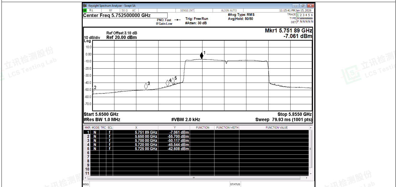
Restrict Band NVNT ac80 5775MHz Ant1 Average
