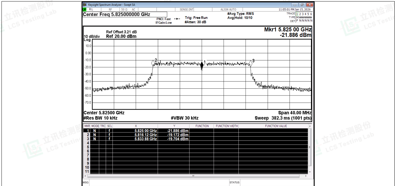
Freq. Stability NVNT ac20 5825MHz Ant1
