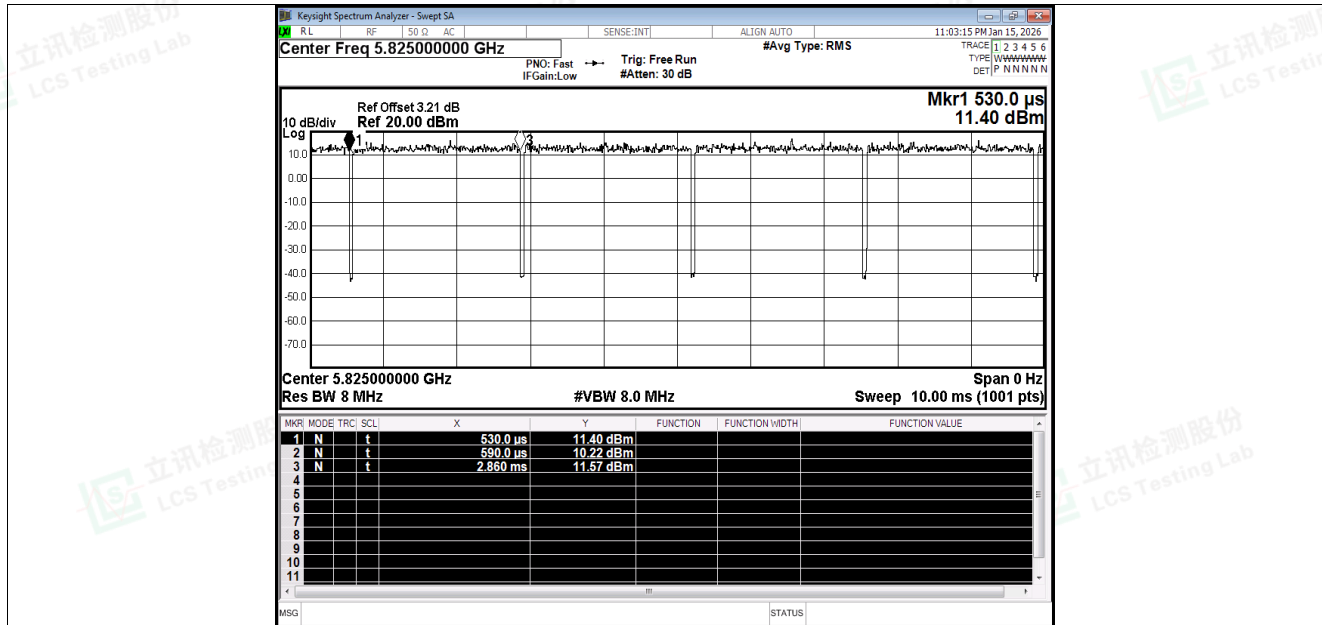
Duty Cycle NVNT ac20 5825MHz Ant1
