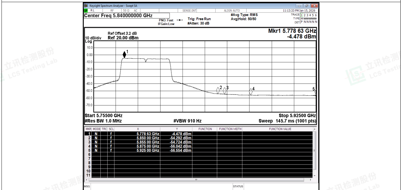
Restrict Band NVNT ac40 5795MHz Ant1 Average
