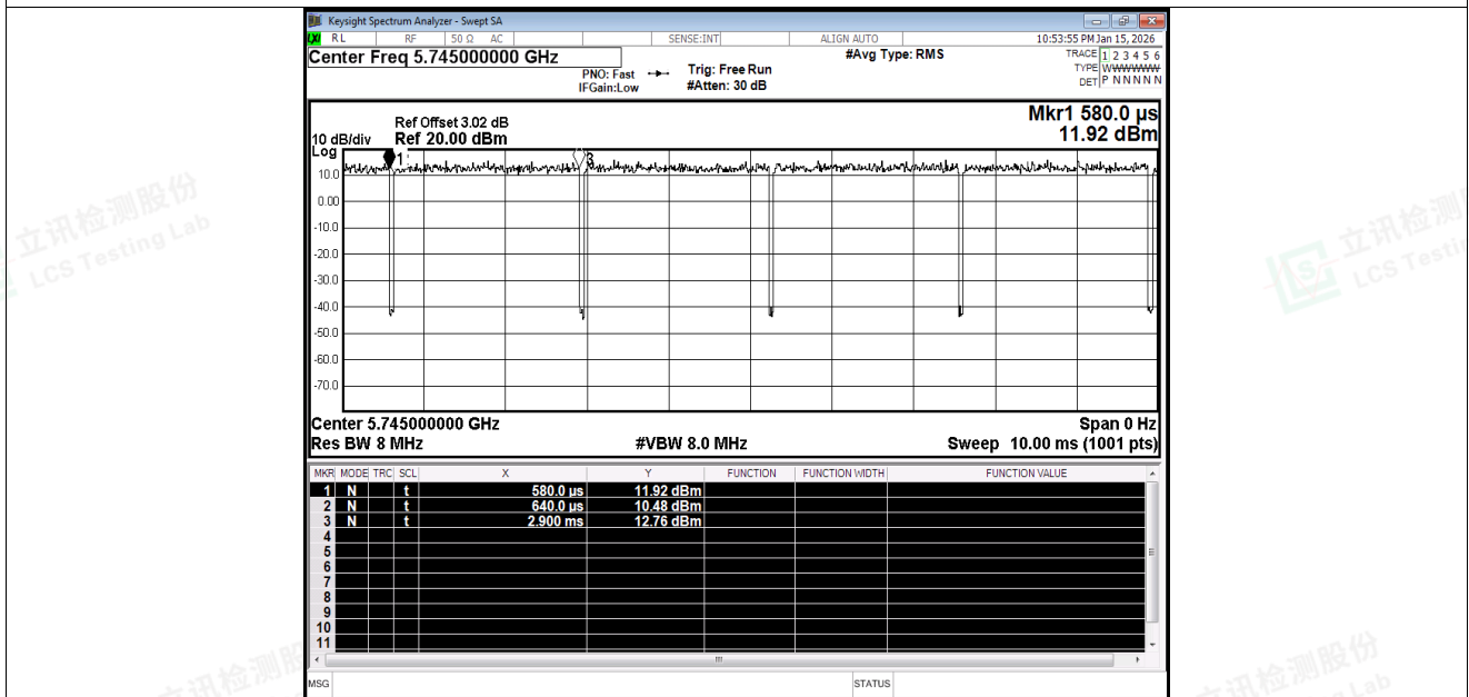
Duty Cycle NVNT n20 5745MHz Ant1
