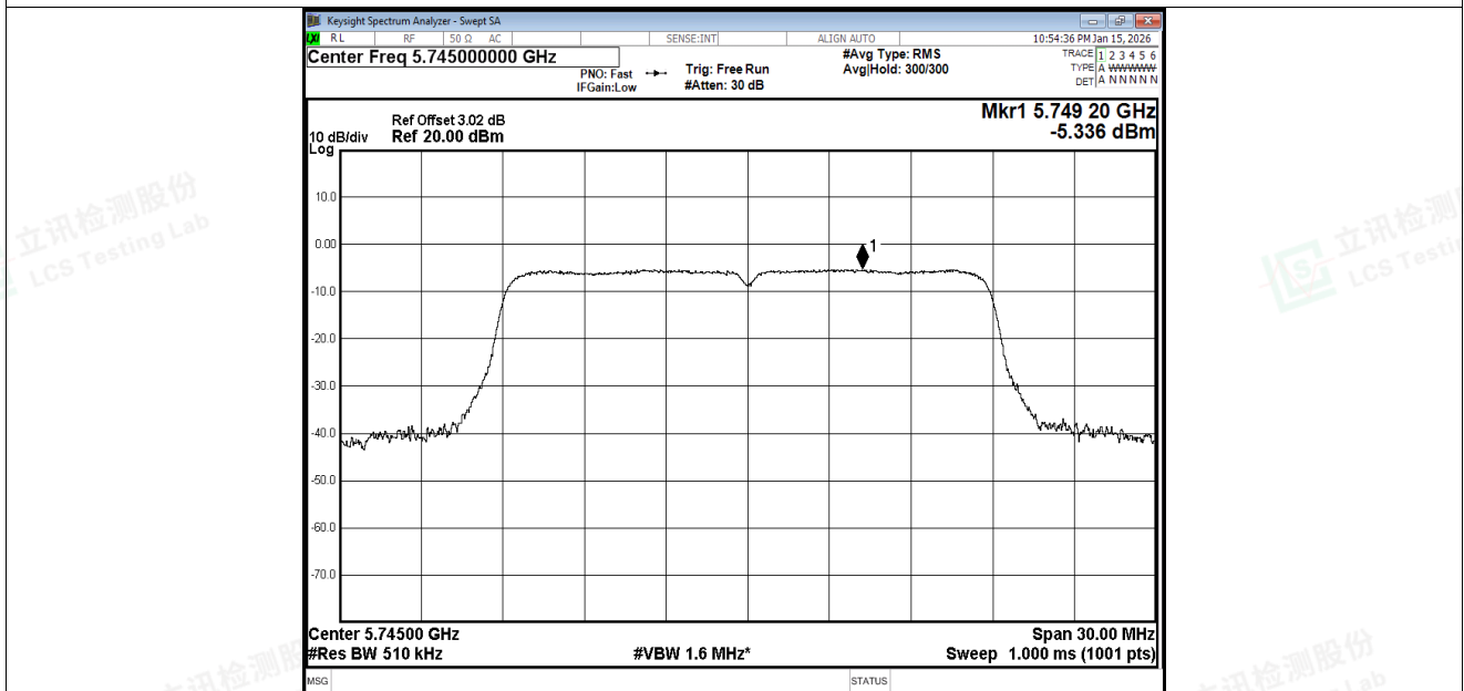
PSD NVNT n20 5745MHz Ant1
