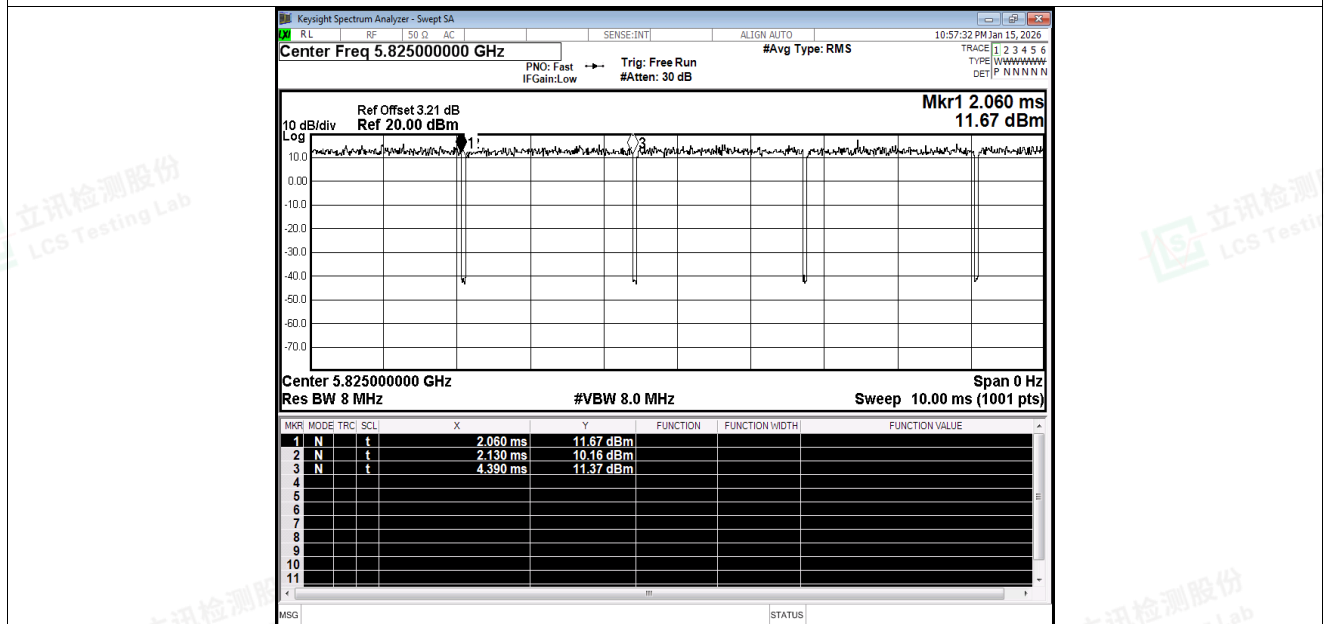
Duty Cycle NVNT n20 5825MHz Ant1
