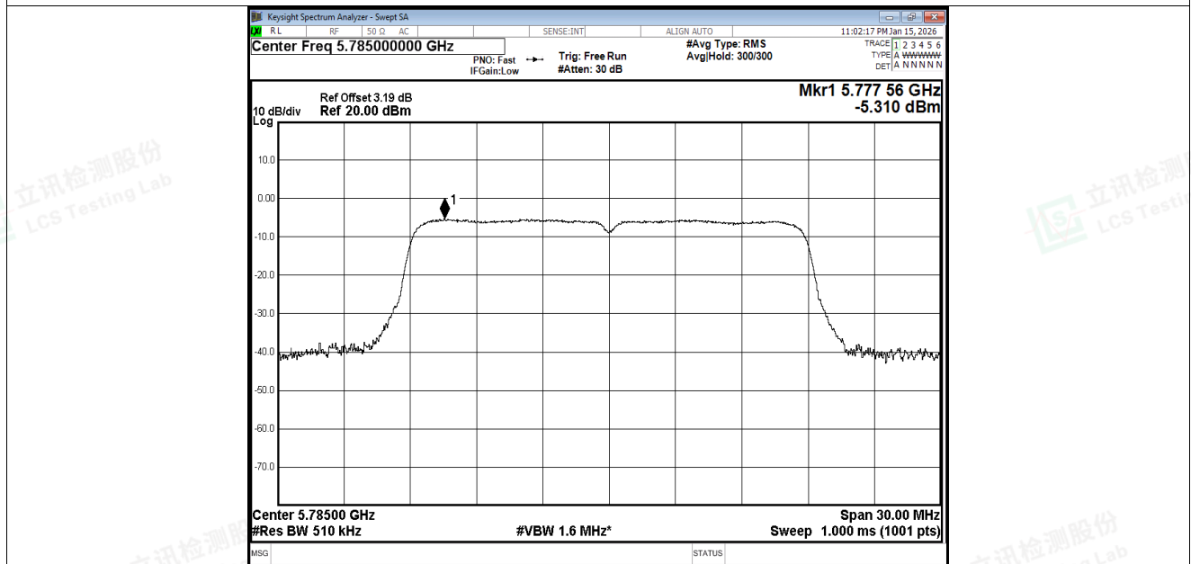
PSD NVNT ac20 5785MHz Ant1
