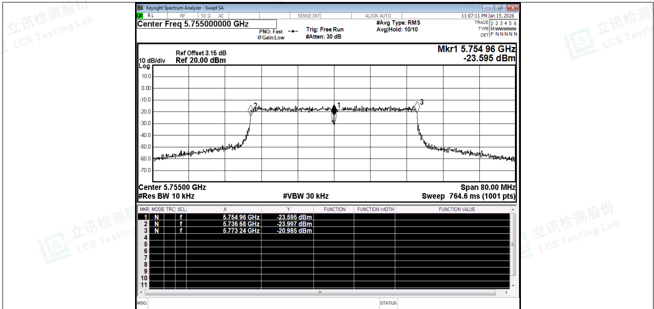
Freq. Stability NVNT n40 5755MHz Ant1
