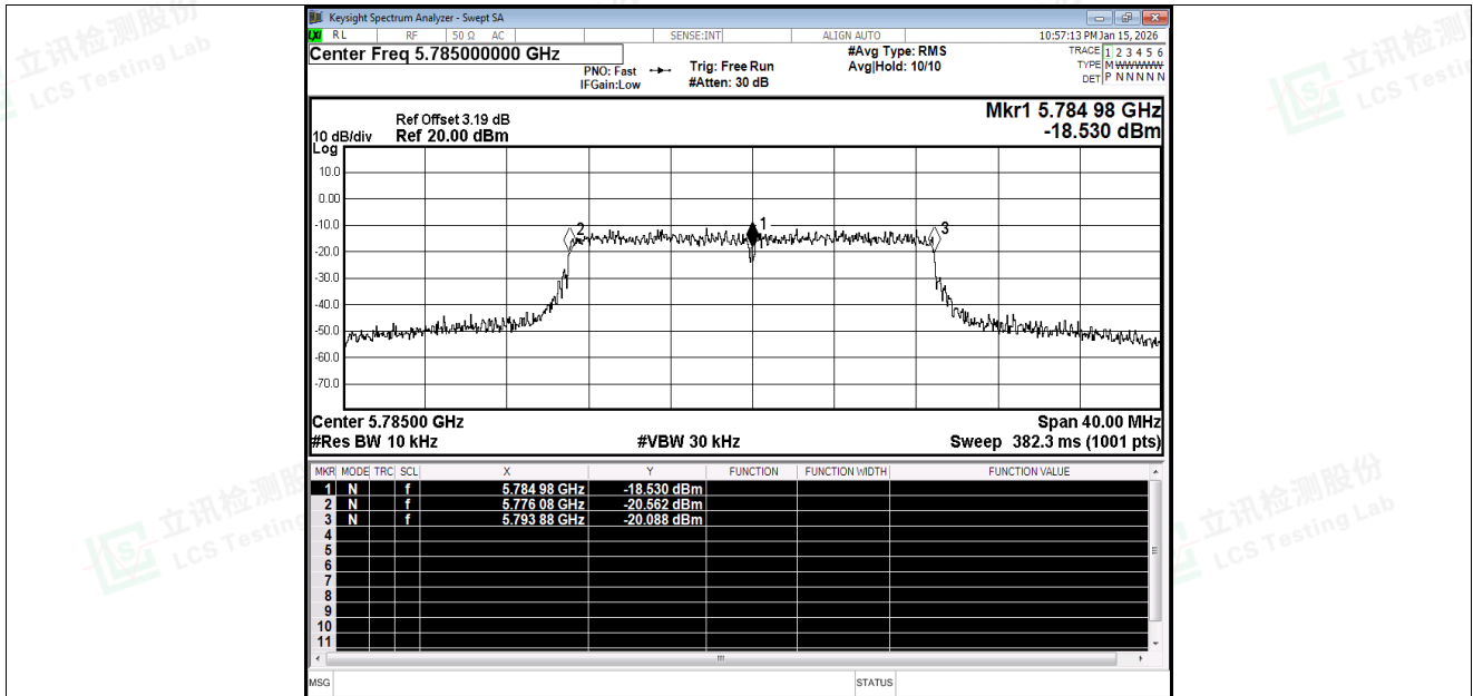
Freq. Stability NVNT n20 5785MHz Ant1
