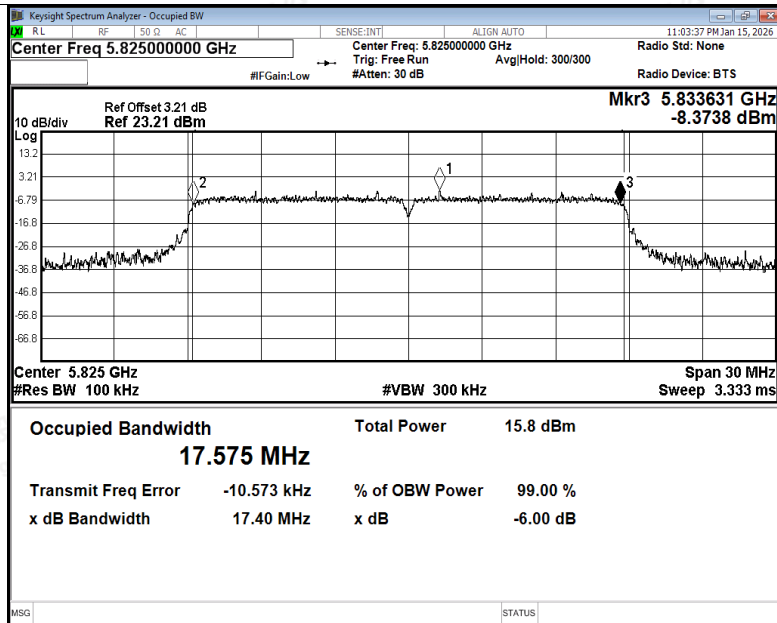
-6dB Bandwidth NVNT ac20 5825MHz Ant1
