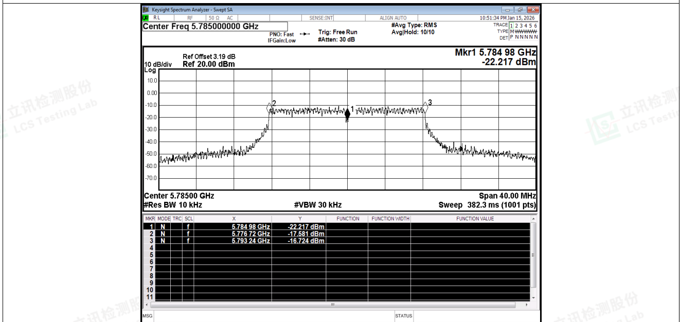
Freq. Stability NVNT a 5785MHz Ant1
