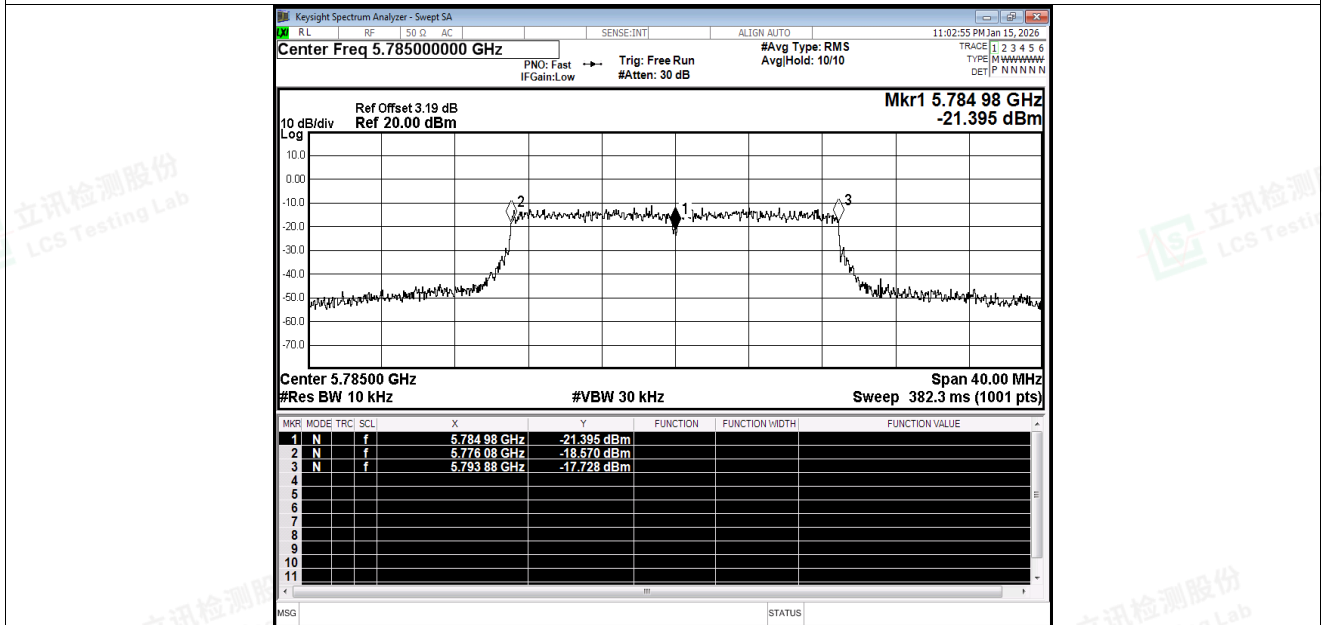
Freq. Stability NVNT ac20 5785MHz Ant1
