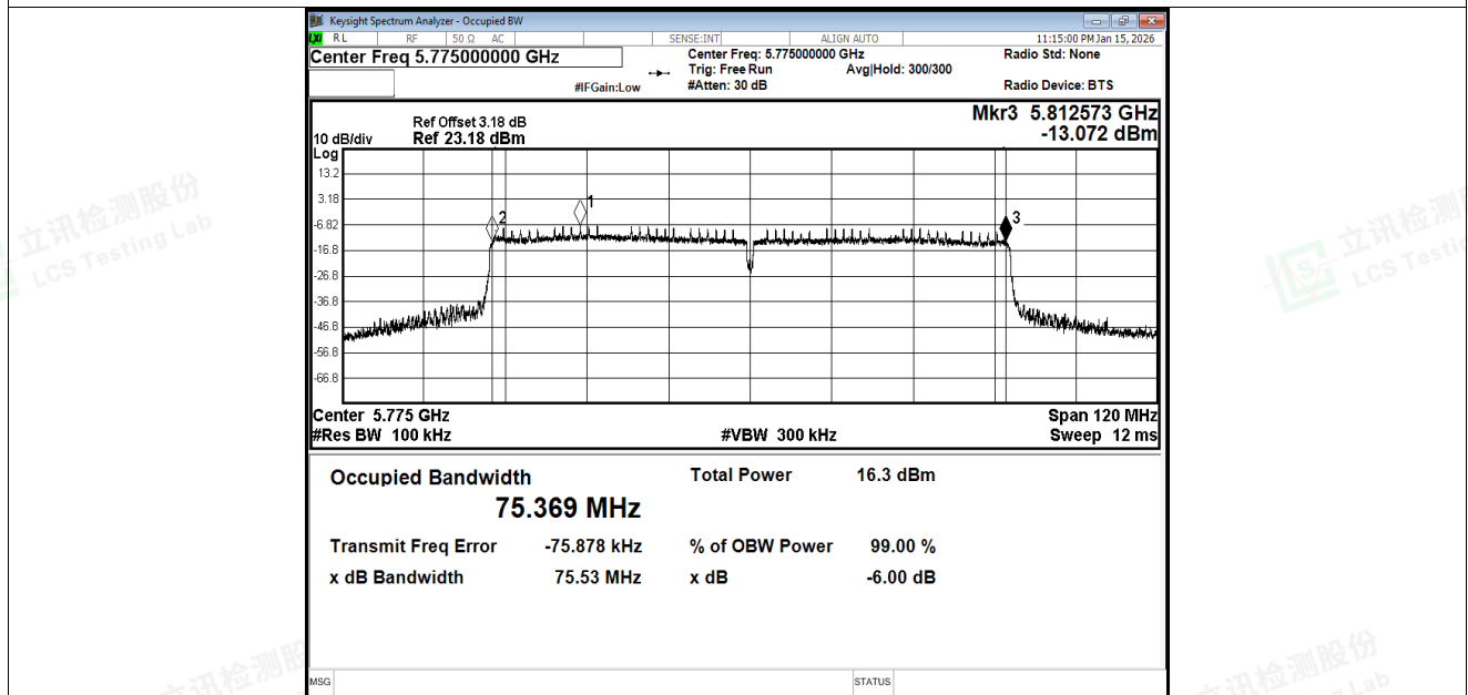
-6dB Bandwidth NVNT ac80 5775MHz Ant1
