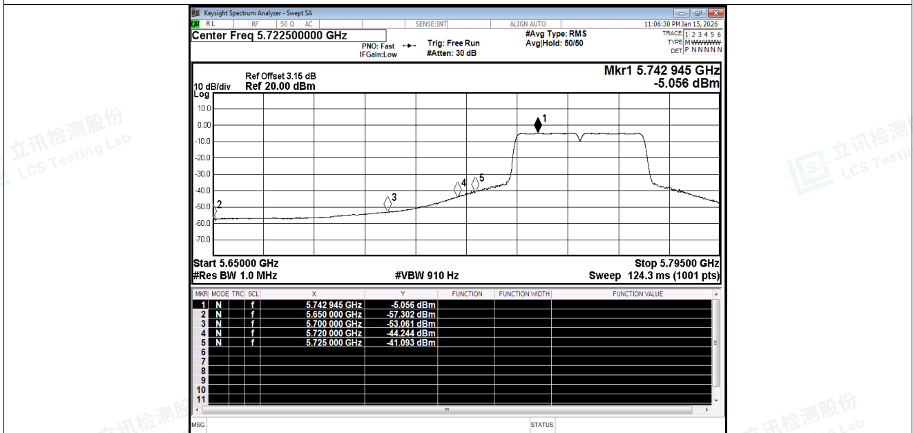
Restrict Band NVNT n40 5755MHz Ant1 Average
