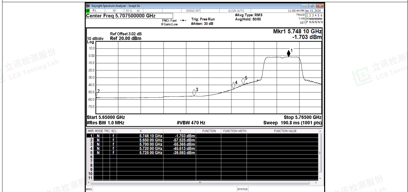
Restrict Band NVNT ac20 5745MHz Ant1 Average
