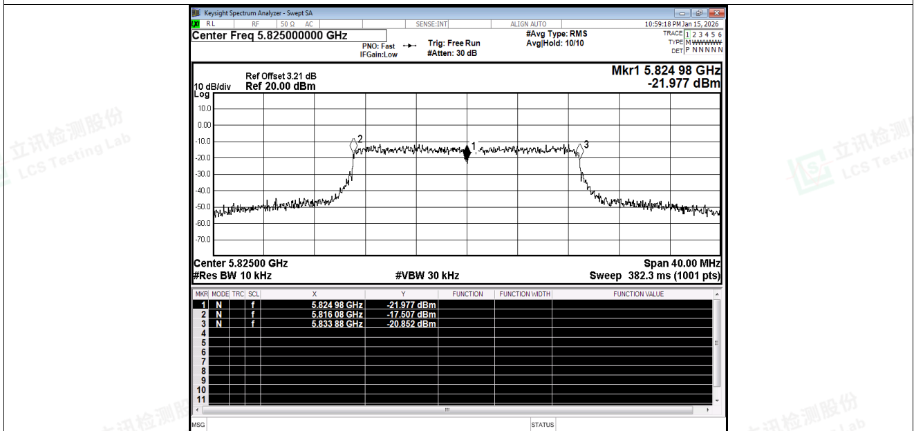
Freq. Stability NVNT n20 5825MHz Ant1
