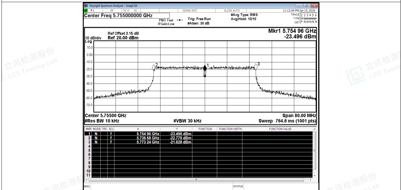
Freq. Stability NVNT ac40 5755MHz Ant1
