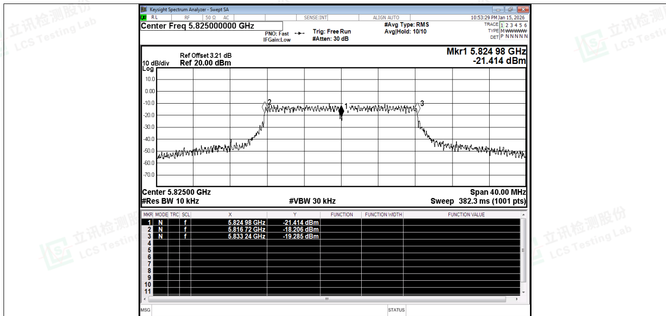
Freq. Stability NVNT a 5825MHz Ant1
