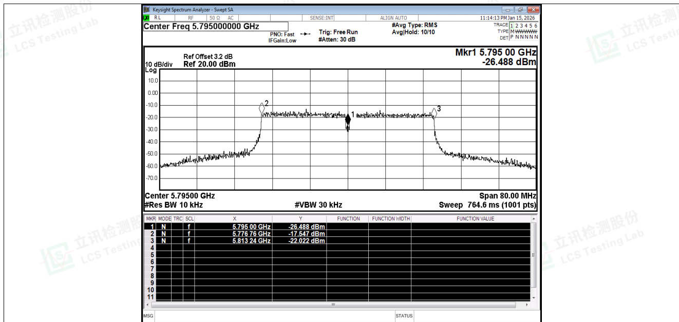
Freq. Stability NVNT ac40 5795MHz Ant1
