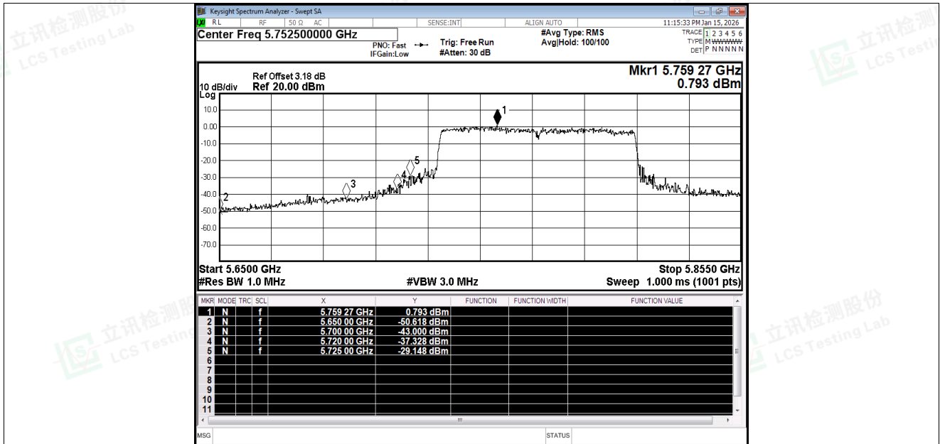
Restrict Band NVNT ac80 5775MHz Ant1 Peak
