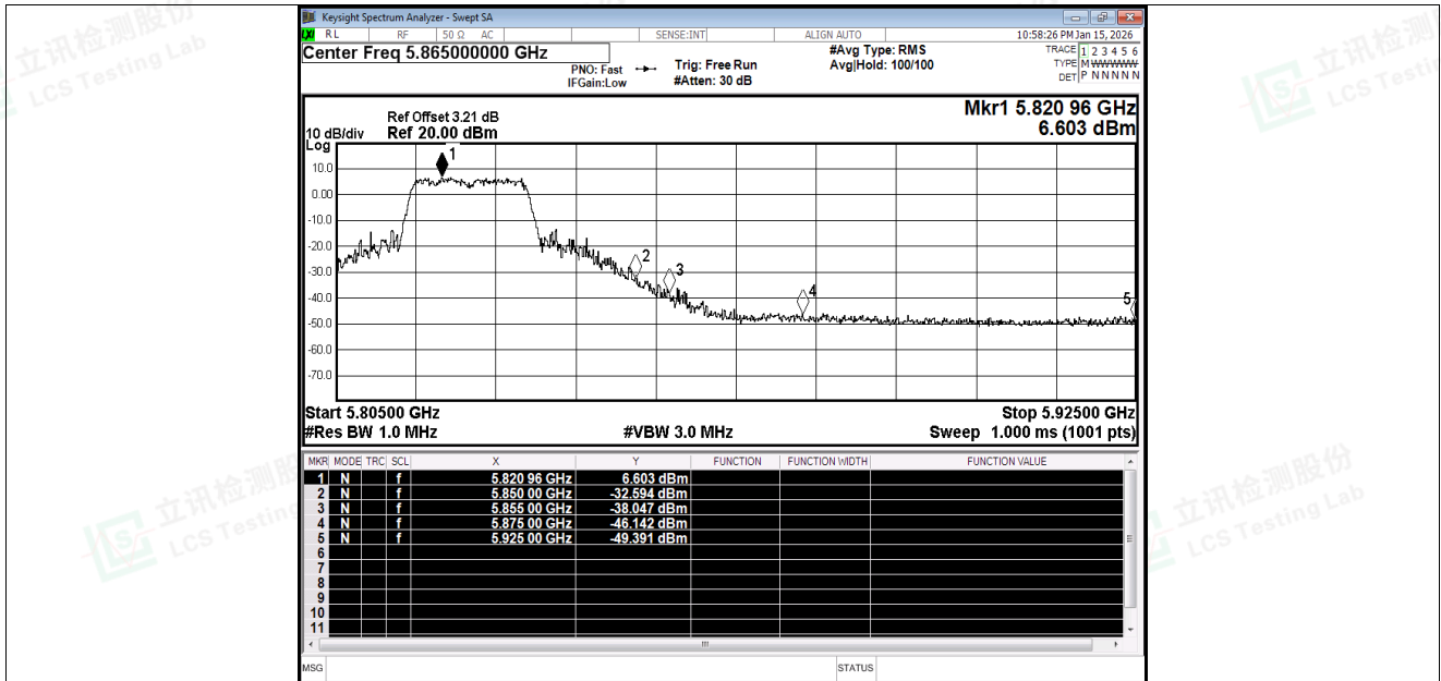
Restrict Band NVNT n20 5825MHz Ant1 Peak
