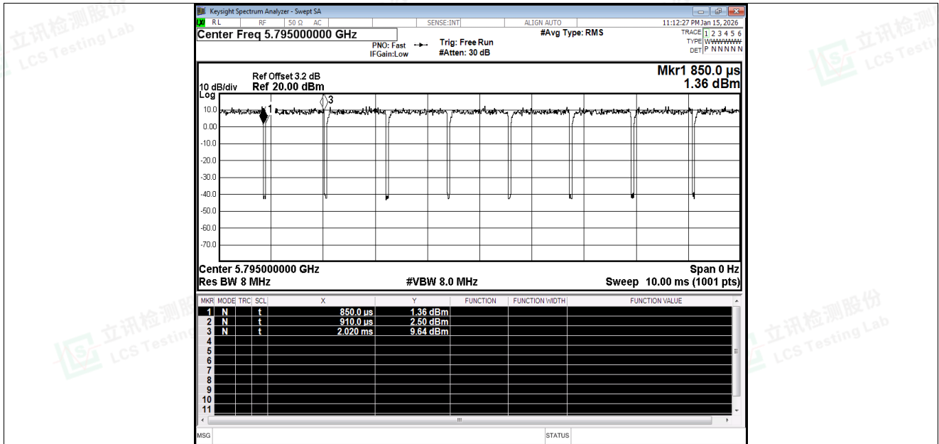
Duty Cycle NVNT ac40 5795MHz Ant1
