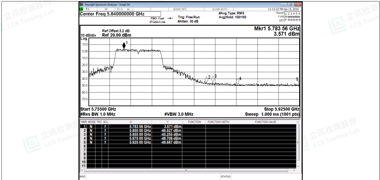
Restrict Band NVNT ac40 5795MHz Ant1 Peak
