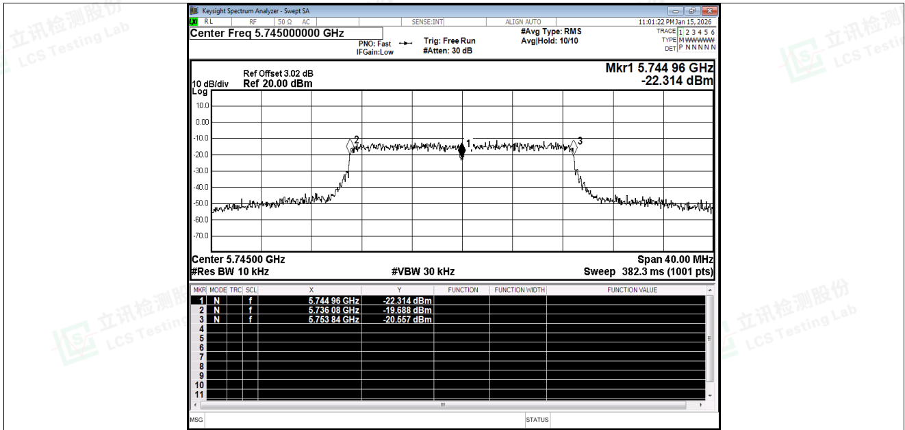
Freq. Stability NVNT ac20 5745MHz Ant1
