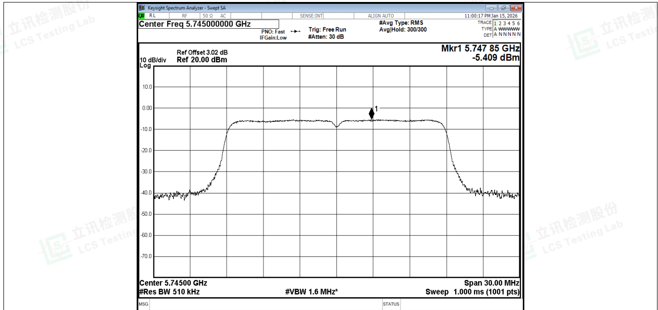
PSD NVNT ac20 5745MHz Ant1
