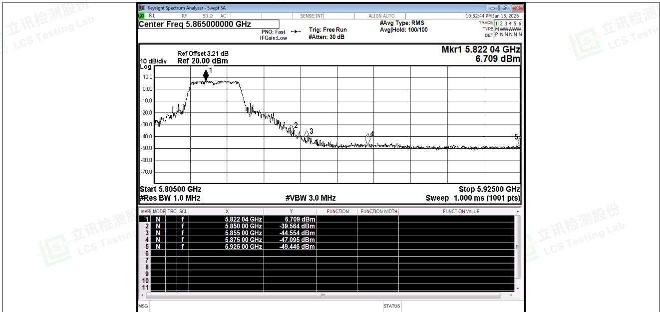
Restrict Band NVNT a 5825MHz Ant1 Peak
