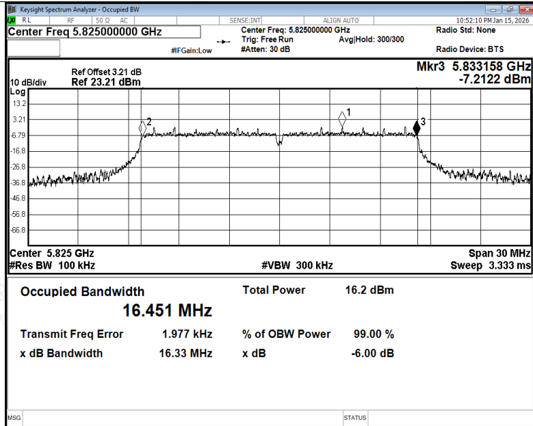
-6dB Bandwidth NVNT a 5825MHz Ant1
