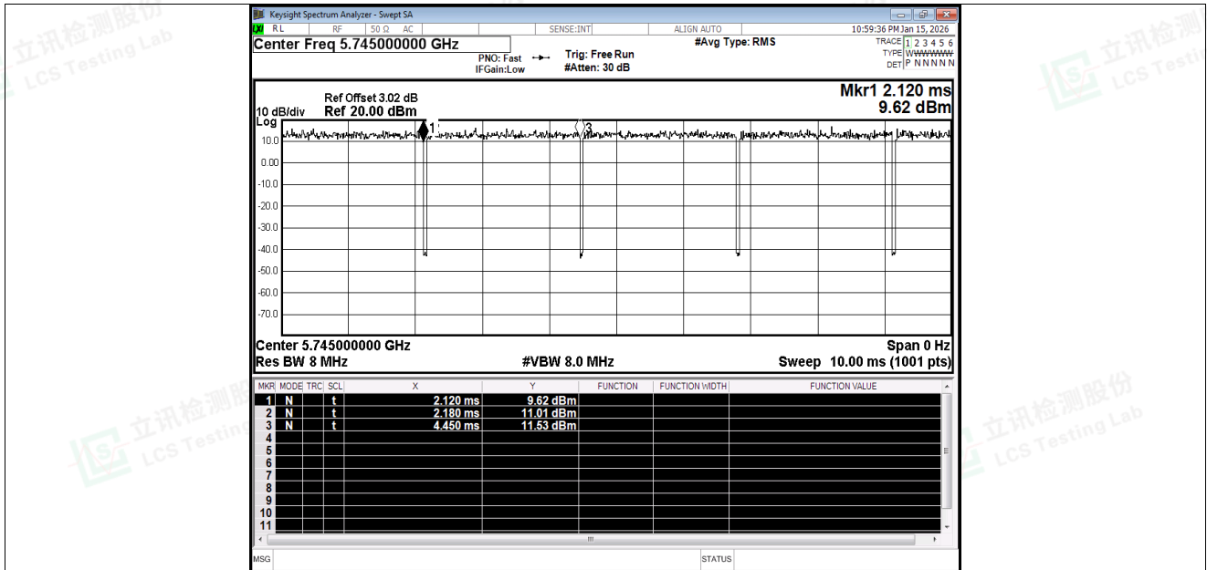
Duty Cycle NVNT ac20 5745MHz Ant1
