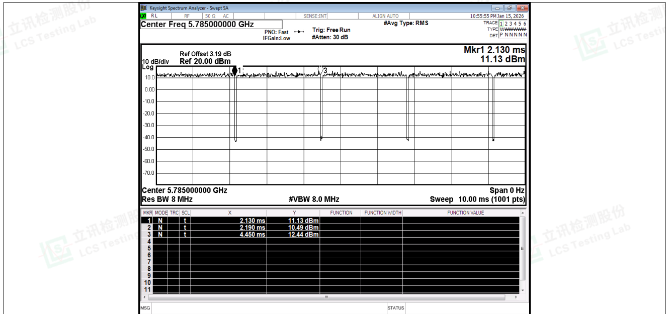
Duty Cycle NVNT n20 5785MHz Ant1
