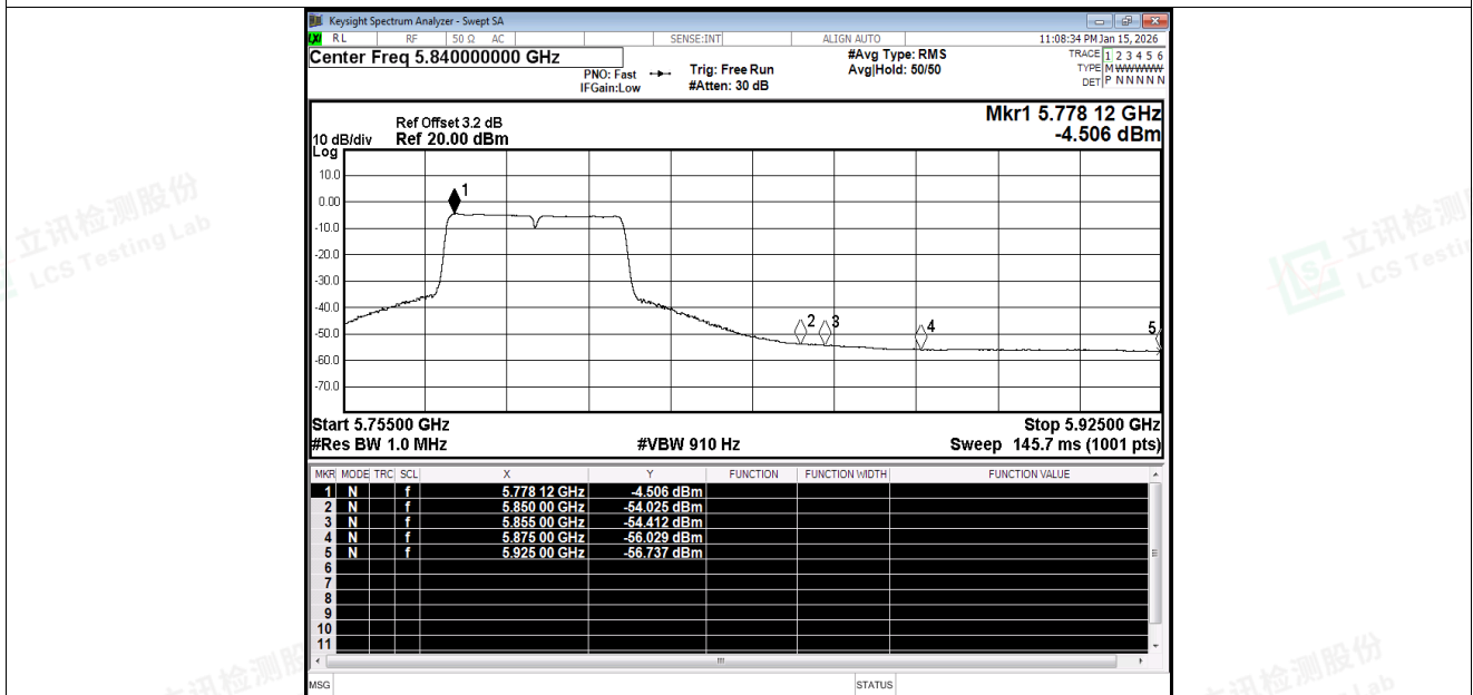
Restrict Band NVNT n40 5795MHz Ant1 Average
