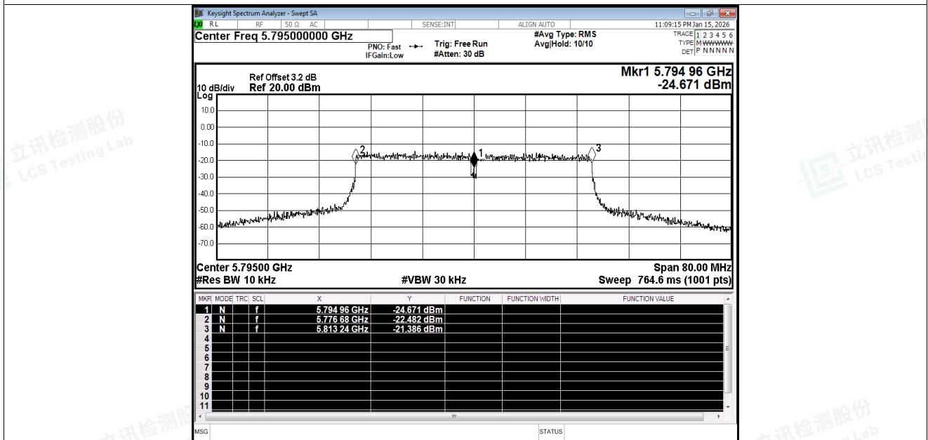
Freq. Stability NVNT n40 5795MHz Ant1
