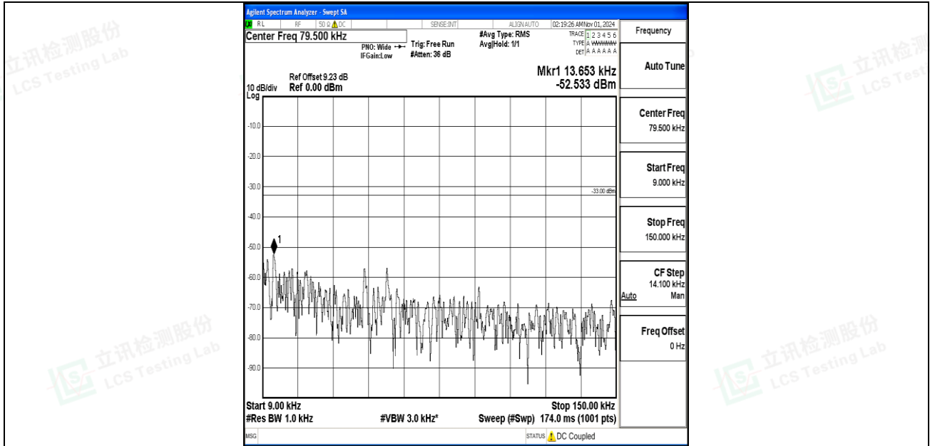
Band5-3MHz-QPSK-20415-1RB#0-0.009~0.15-PASS
