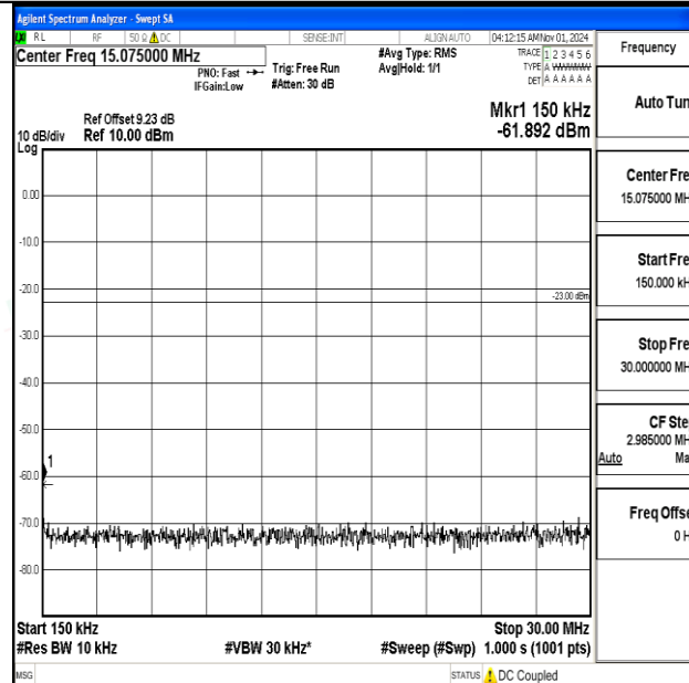
Band12-3MHz-QPSK-23025-1RB#0-0.15~30-PASS
