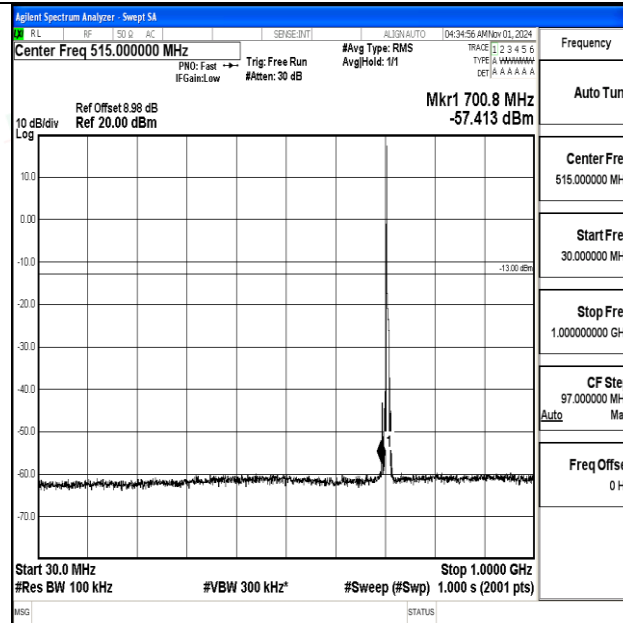
Band12-5MHz-QPSK-23155-1RB#0-30~1000-PASS
