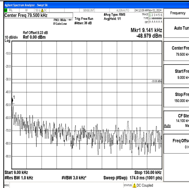
Band12-3MHz-QPSK-23025-1RB#0-0.009~0.15-PASS
