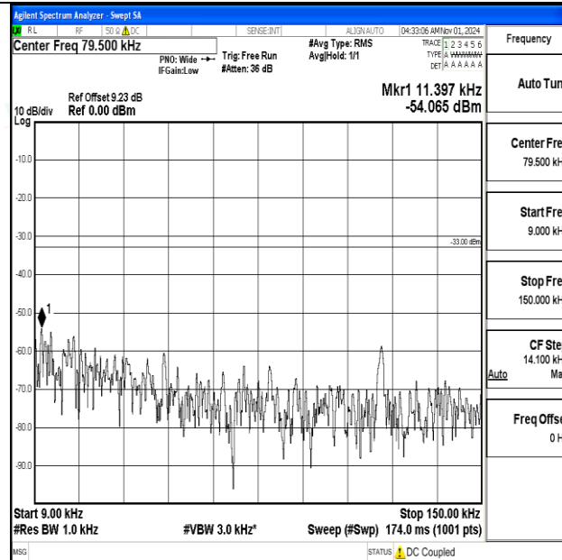
Band12-5MHz-QPSK-23095-1RB#0-0.009~0.15-PASS
