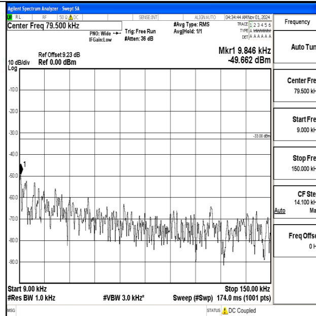
Band12-5MHz-QPSK-23155-1RB#0-0.009~0.15-PASS
