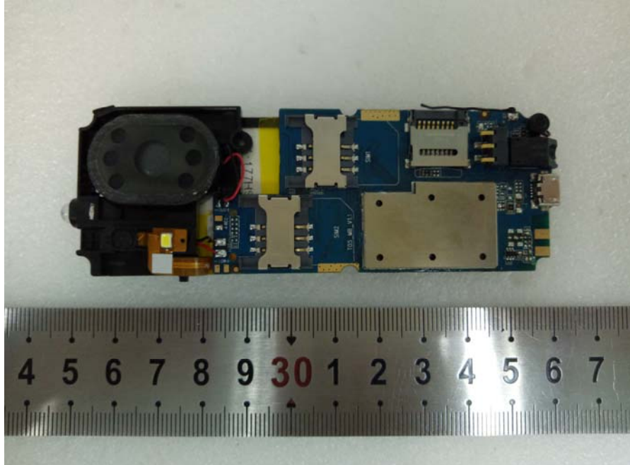
EUT –Main Board Rear View
