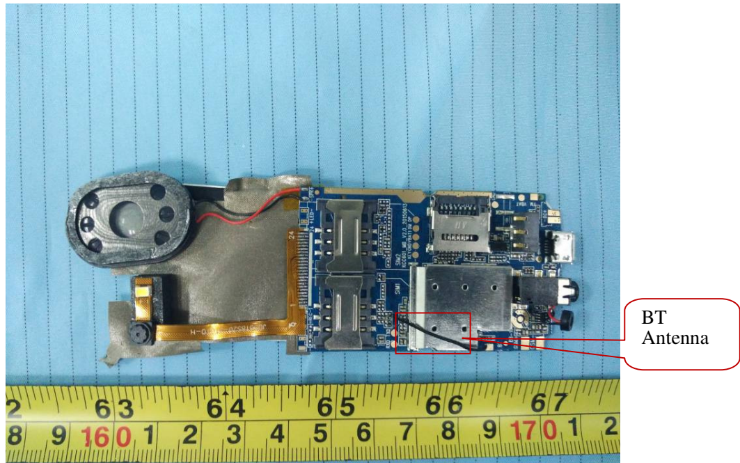
EUT – Main Board Bottom View 1
