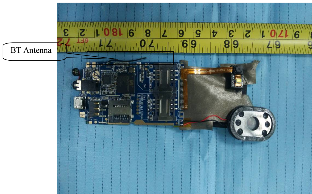
EUT – Main Board Bottom Shielding off View
