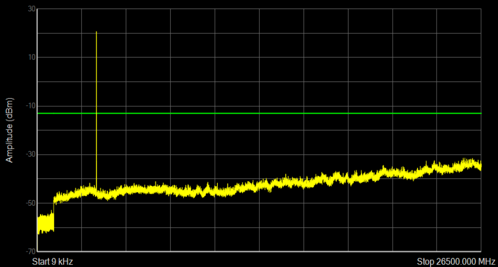
Band42 QAM16 BW=5MHz Channel=43065 RB Size=25 Position=#0
