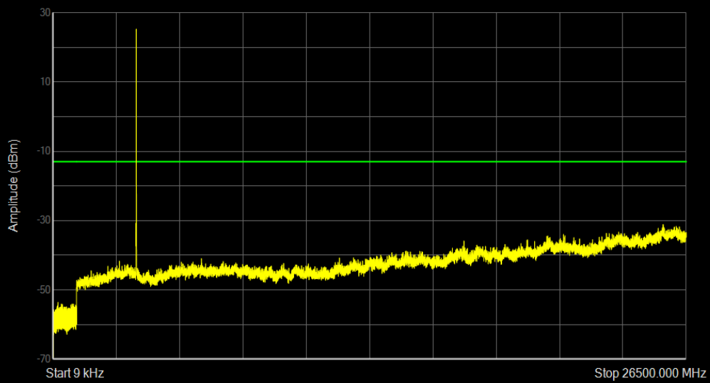
Band42 QAM16 BW=5MHz Channel=42590 RB Size=1 Position=#0
