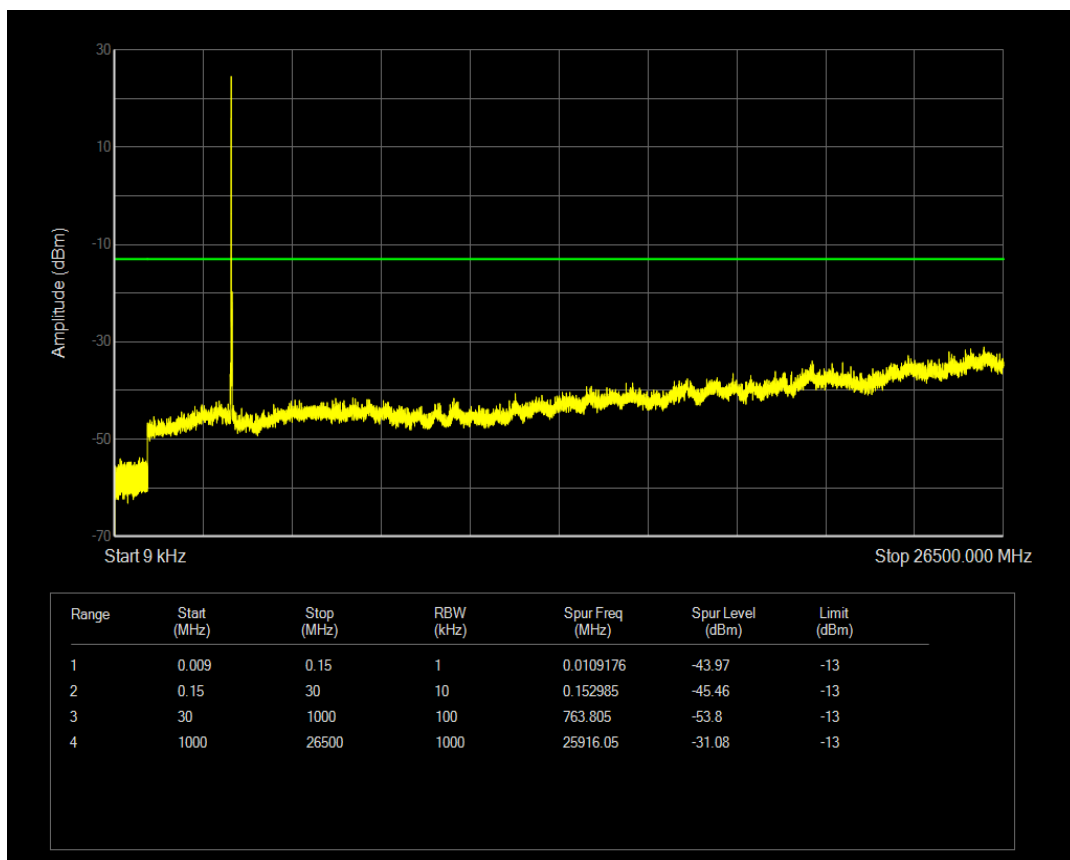
Band42 QAM16 BW=15MHz Channel=42590 RB Size=1 Position=#0
