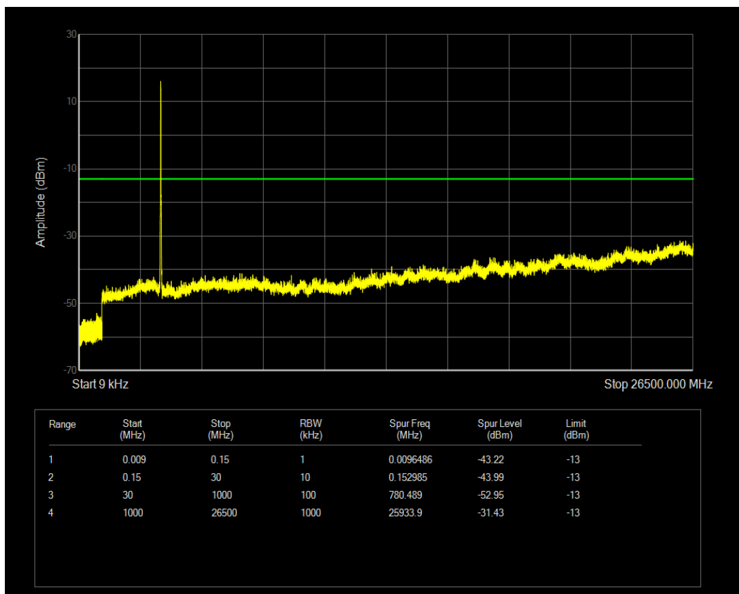
Band42 QAM16 BW=20MHz Channel=42990 RB Size=1 Position=#0
