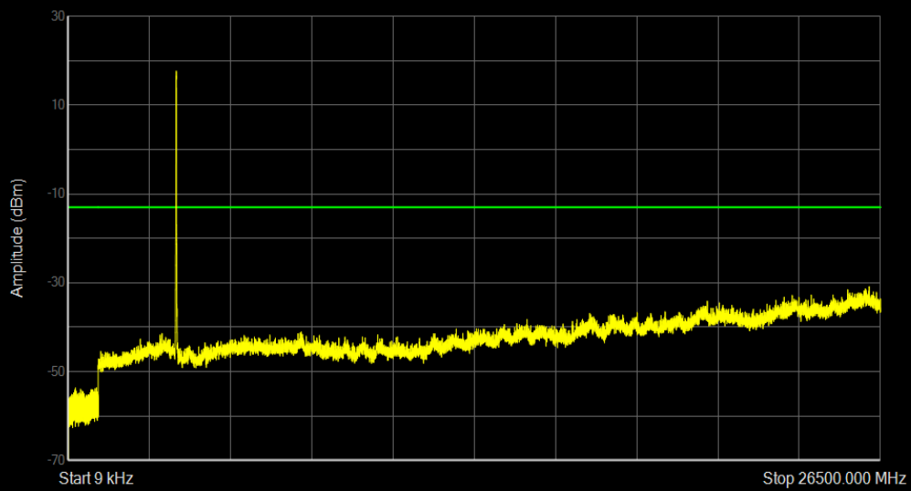
Band42 QAM16 BW=15MHz Channel=43015 RB Size=75 Position=#0
