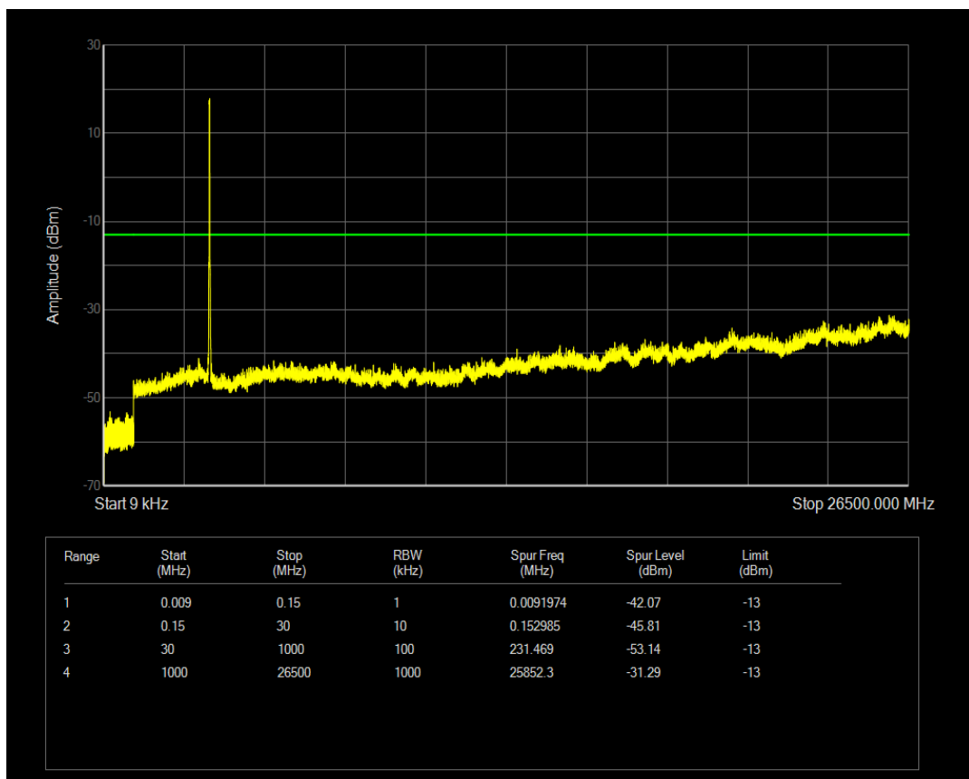
Band42 QAM16 BW=20MHz Channel=42590 RB Size=1 Position=#0
