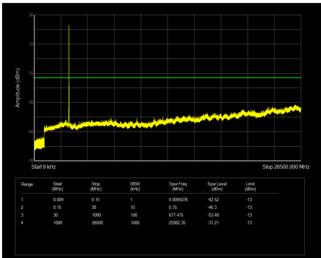
Band42 QAM16 BW=10MHz Channel=42140 RB Size=50 Position=#0
