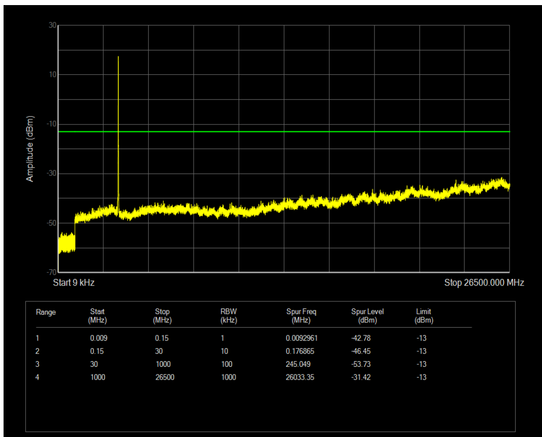
Band42 QAM16 BW=15MHz Channel=43015 RB Size=1 Position=#0
