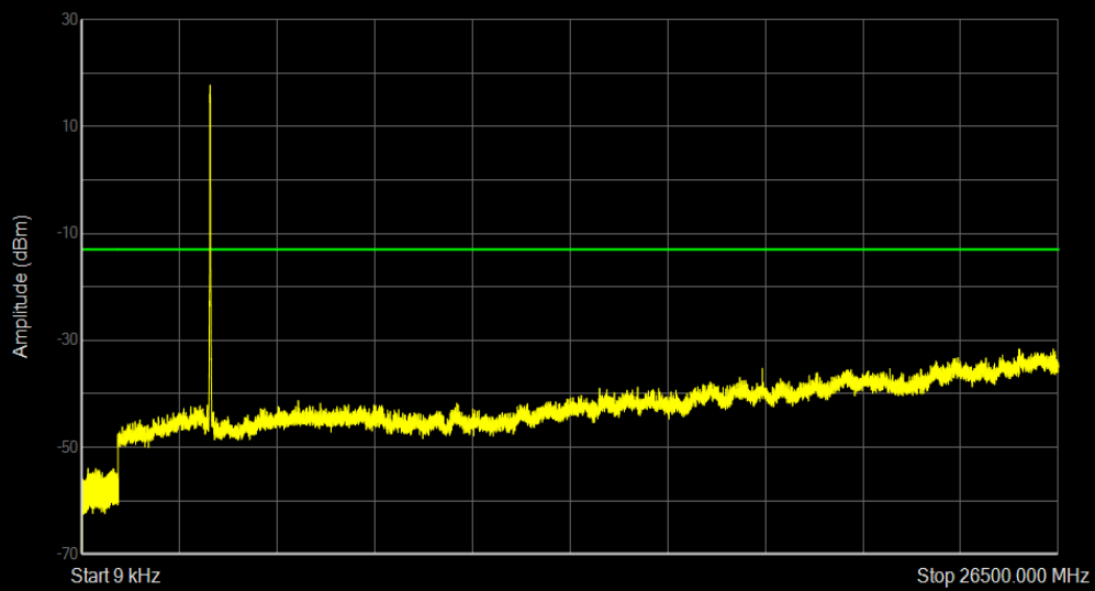
Band42 QAM16 BW=20MHz Channel=42590 RB Size=100 Position=#0
