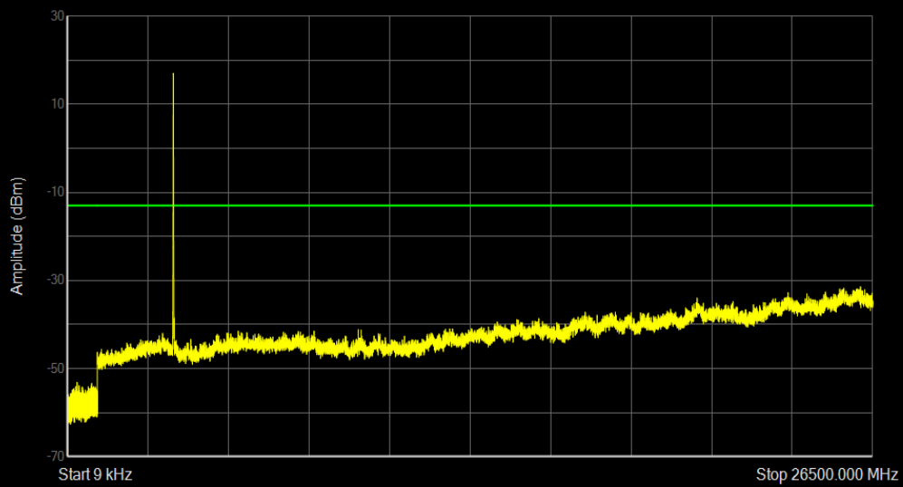
Band42 QAM16 BW=10MHz Channel=42590 RB Size=50 Position=#0
