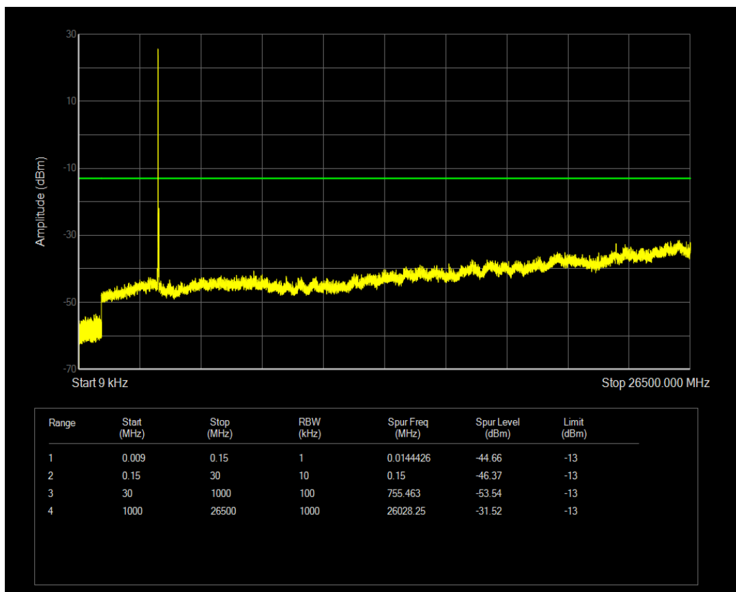
Band42 QAM16 BW=20MHz Channel=42190 RB Size=100 Position=#0
