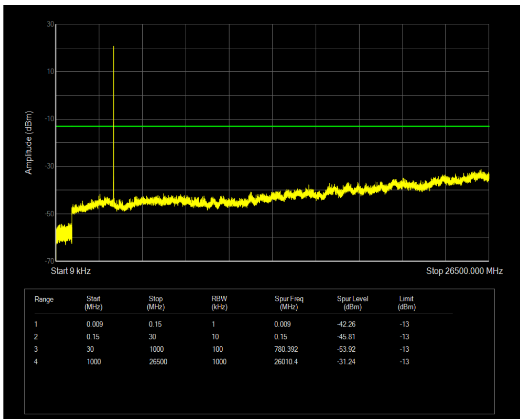
Band42 QAM16 BW=5MHz Channel=43065 RB Size=1 Position=#0
