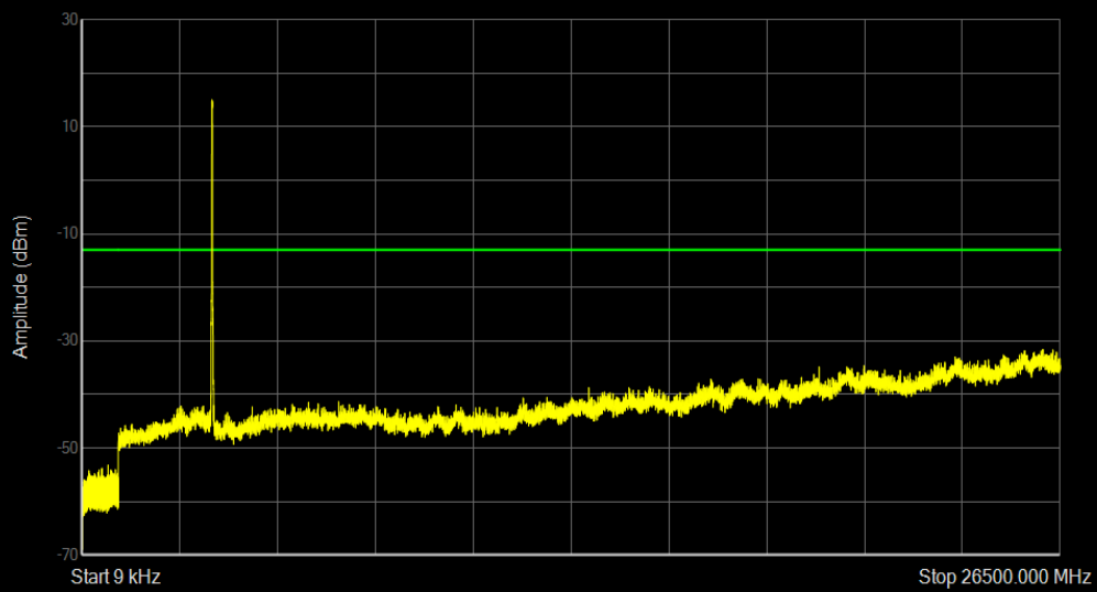
Band42 QAM16 BW=20MHz Channel=42990 RB Size=100 Position=#0
