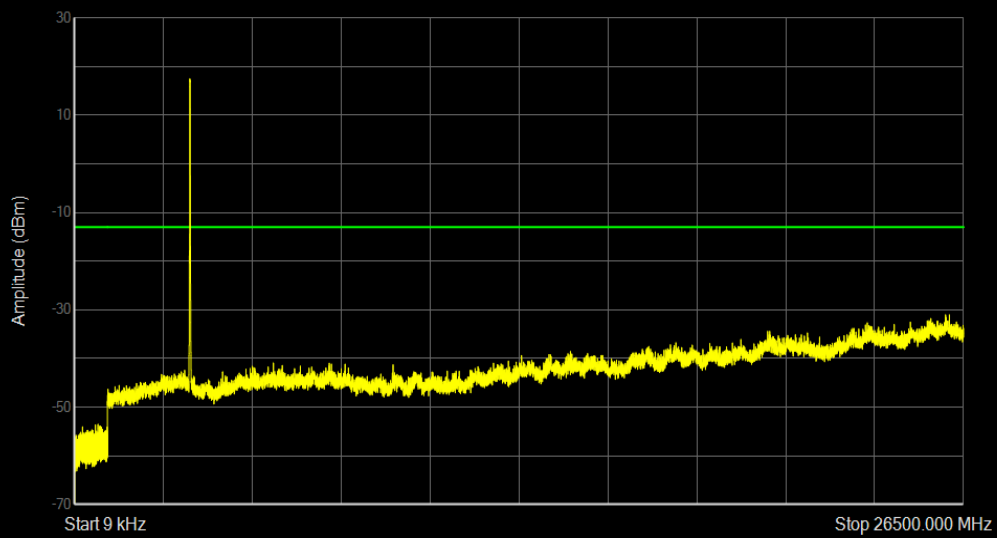
Band42 QPSK BW=15MHz Channel=42165 RB Size=75 Position=#0
