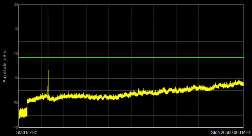
Band42 QPSK BW=20MHz Channel=42190 RB Size=1 Position=#0
