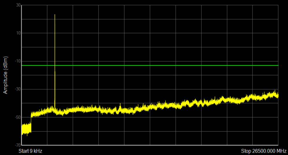
Band42 QPSK BW=10MHz Channel=42140 RB Size=1 Position=#0
