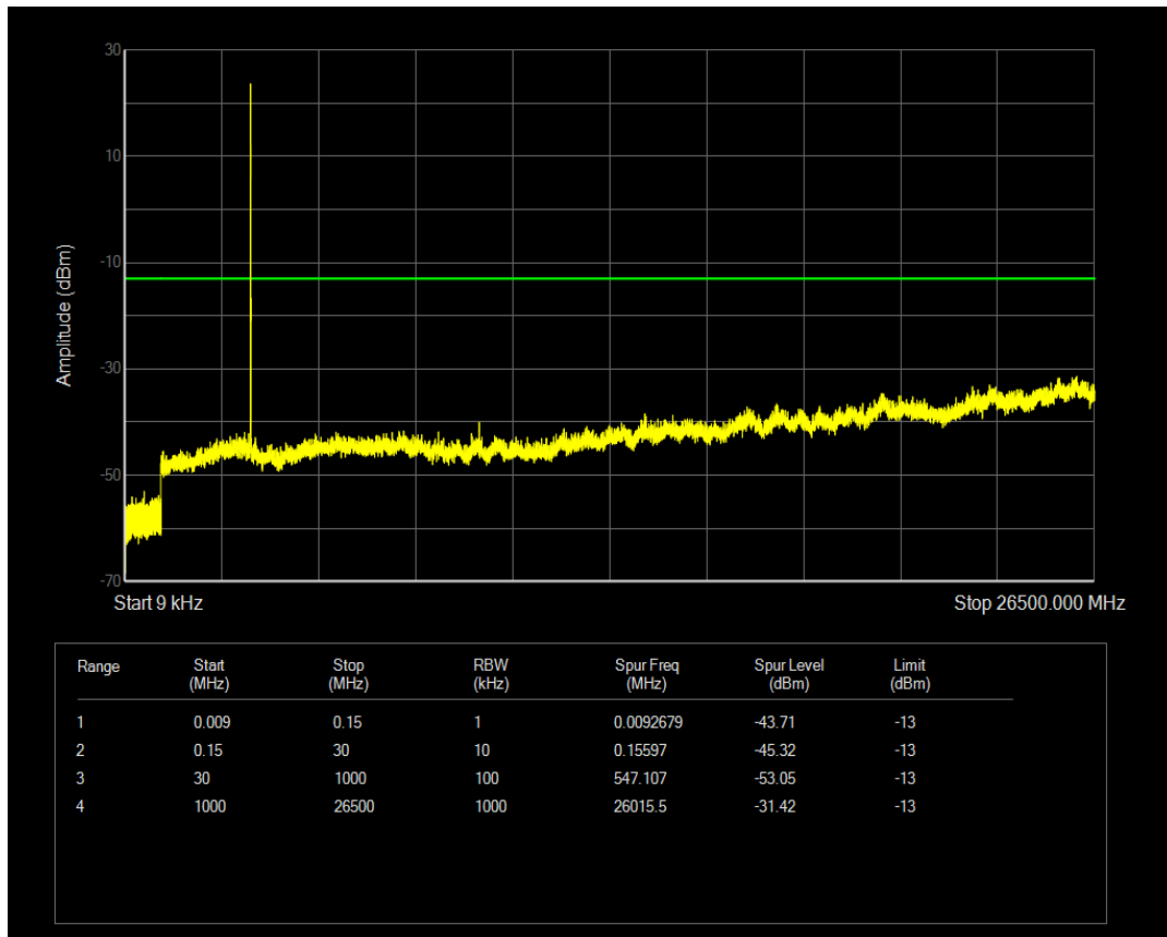
Band42 QAM16 BW=5MHz Channel=42115 RB Size=25 Position=#0
