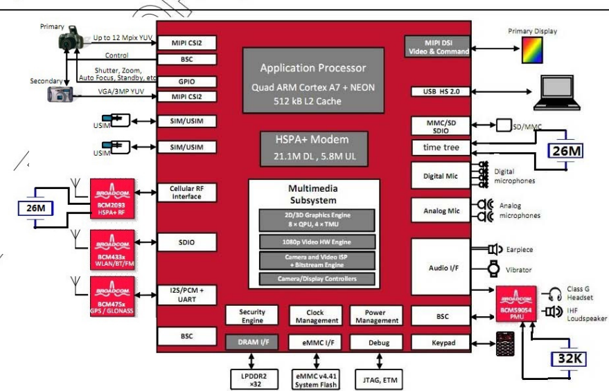
Figure 1: Functional Block Diagram of a BCM23550-Based 3G Platform Solution
