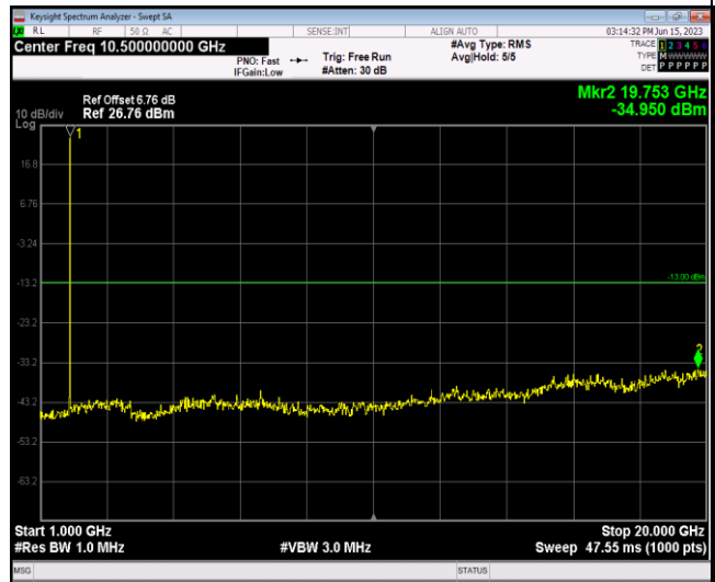
Band2-1.4MHz-QPSK-18900-1RB#0-Range2:1000~ 20000MHz
