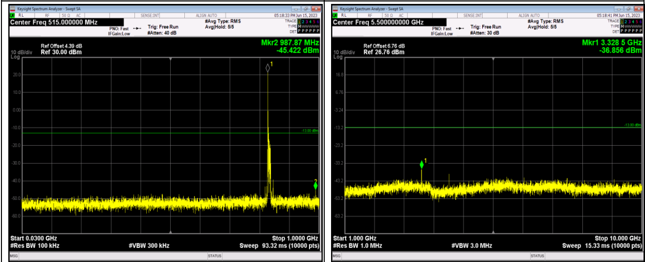
Band5-10MHz-16QAM-20525-1RB#0-Range1:30~1000MHz
