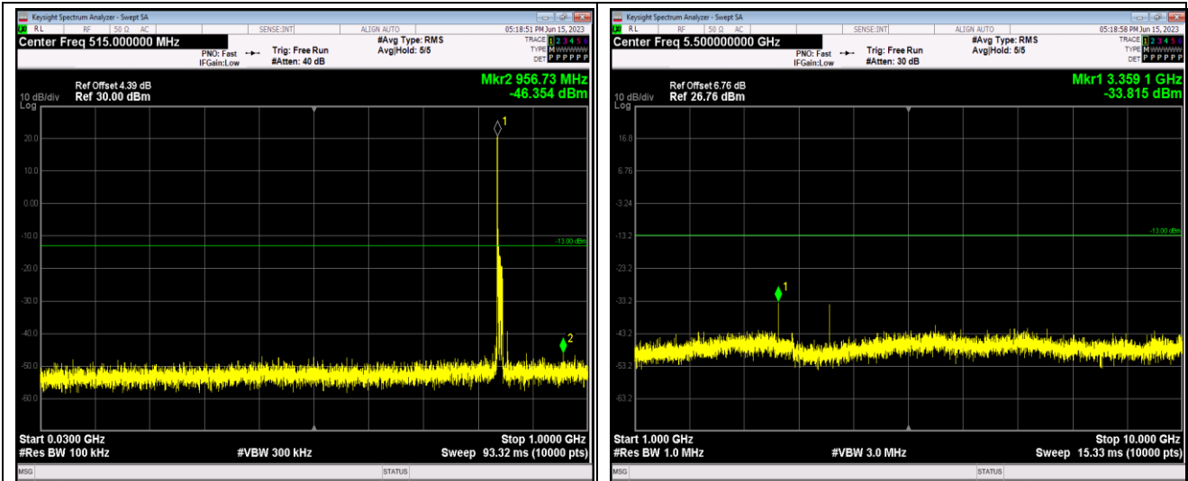
Band5-10MHz-16QAM-20450-1RB#0-Range1:30~1000MHz
