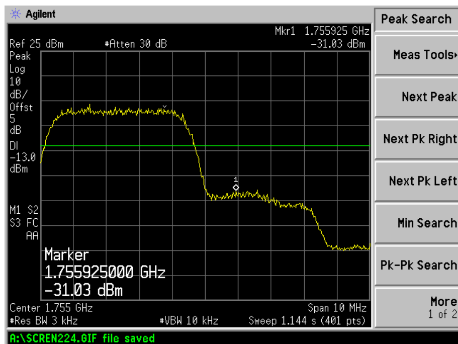
WCDMA High Band Spurious Emission
