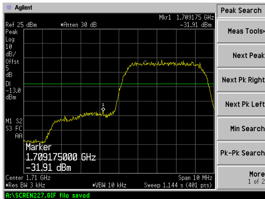
WCDMA Low Band Spurious Emission
