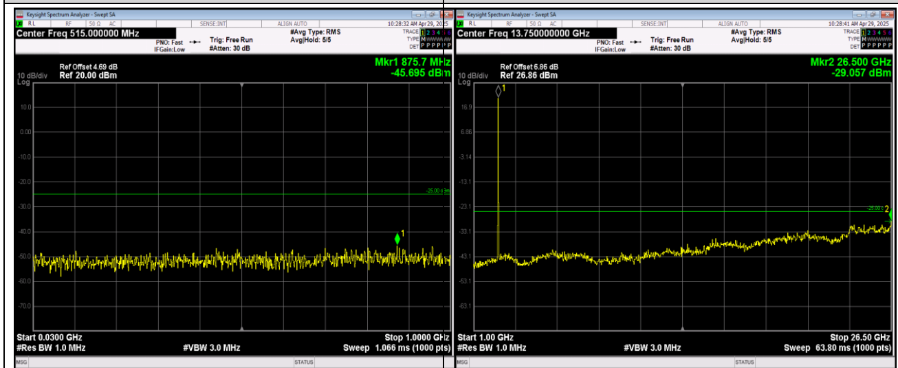
Band7-20MHz-QPSK-21100-1RB#0-Range1:30~1000MHz
