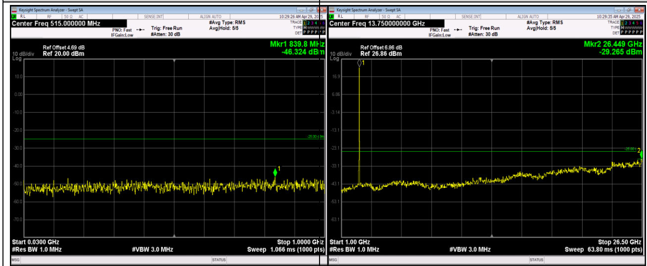
Band7-20MHz-QPSK-21100-1RB#0-Range1:30~1000MHz
