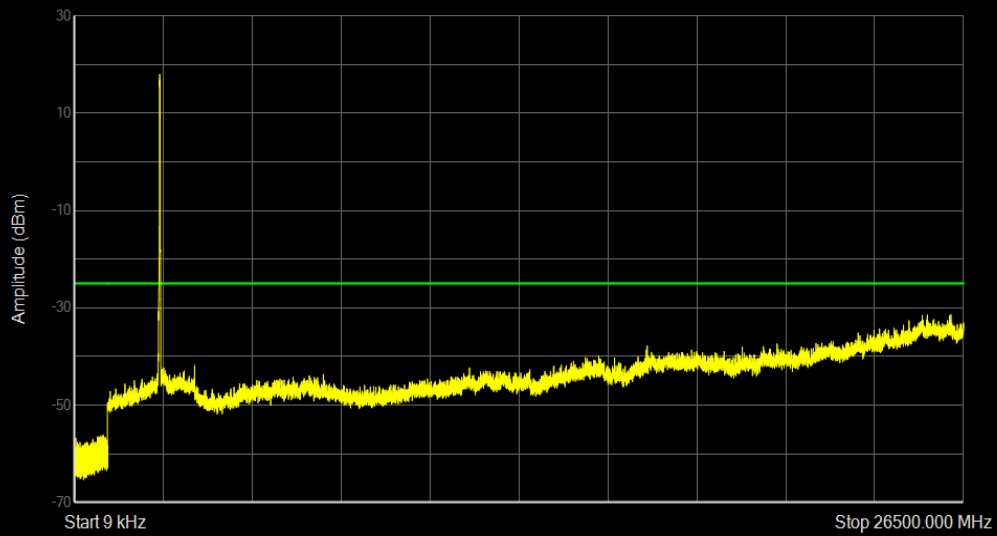
Band7 16QAM BW=20MHz Channel=21350 RB Size=100 Position=#0
