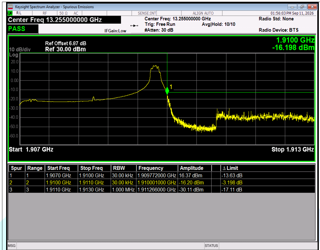
Band2 16QAM BW=3MHz Channel=19185 RB Size=1 Position=#Max NVNT
