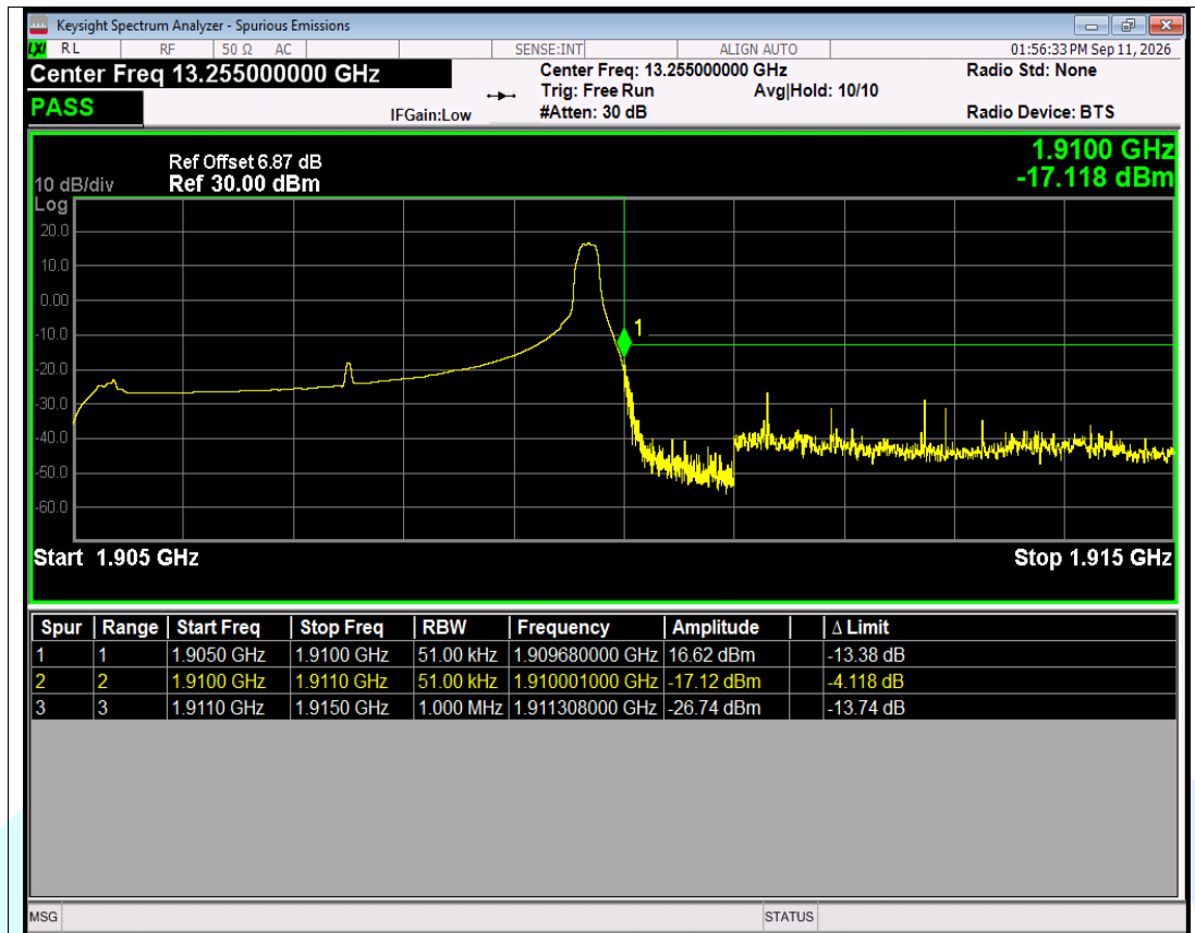
Band2 16QAM BW=5MHz Channel=19175 RB Size=1 Position=#Max NVNT
