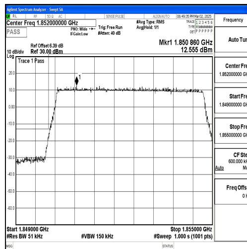
Band2_5MHz_QPSK_18625_25RB#0
