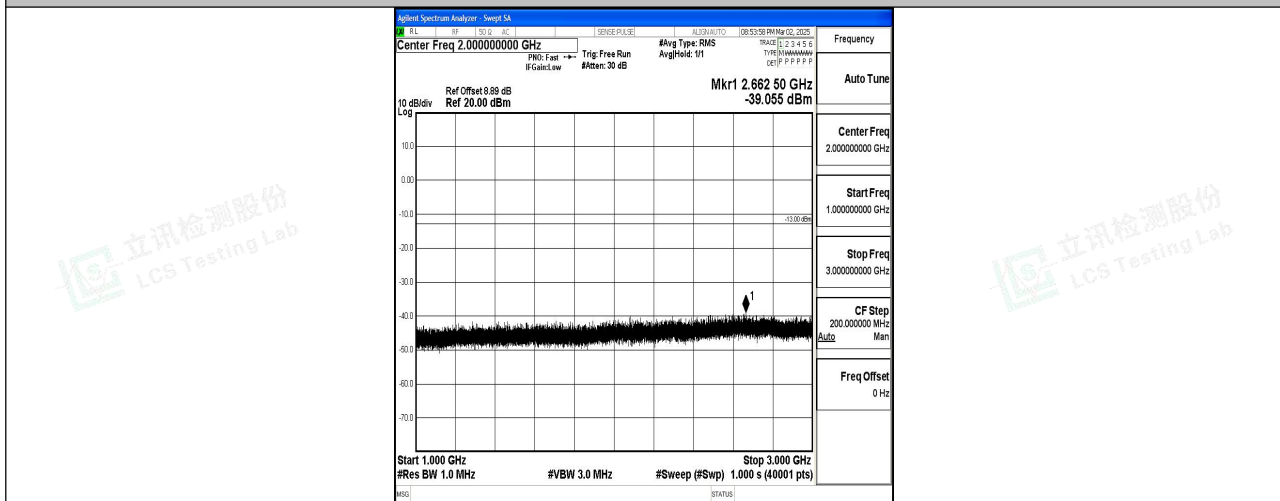
Band2_5MHz_QPSK_18625_1RB#0_1000~3000_1000~3000
