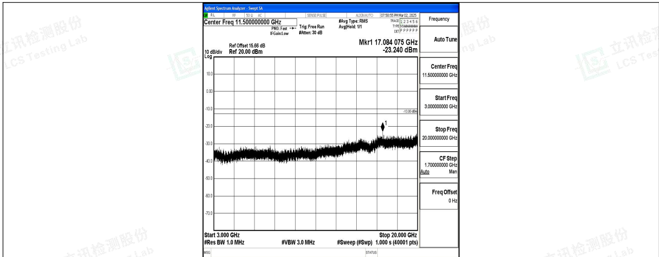
Band2_3MHz_16QAM_18900_1RB#0_3000~20000_3000~20000
