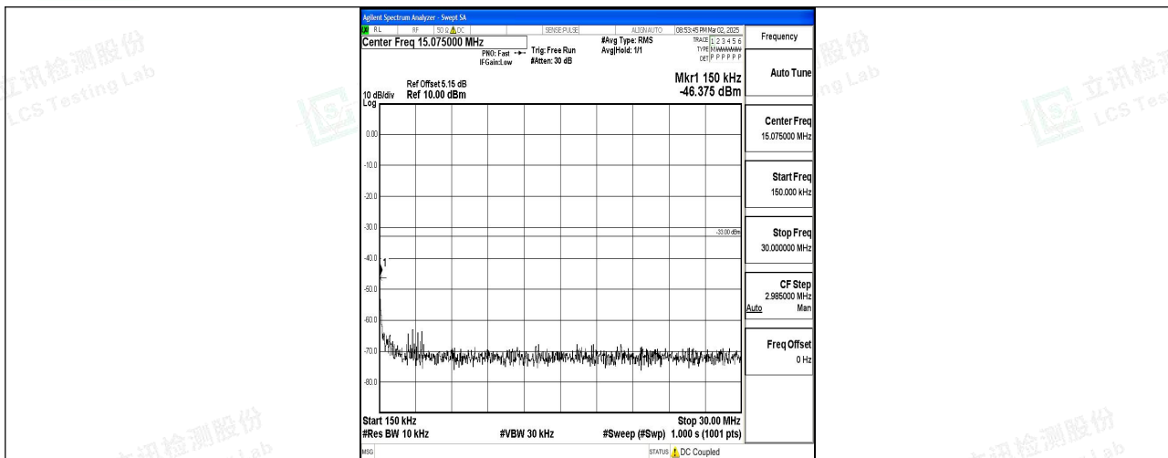
Band2_5MHz_QPSK_18625_1RB#0_0.15~30_0.15~30
