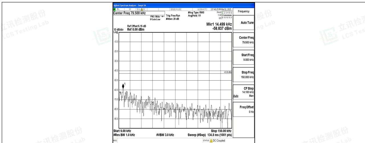
Band2_1.4MHz_16QAM_19193_1RB#0_0.009~0.15_0.009~0.15
