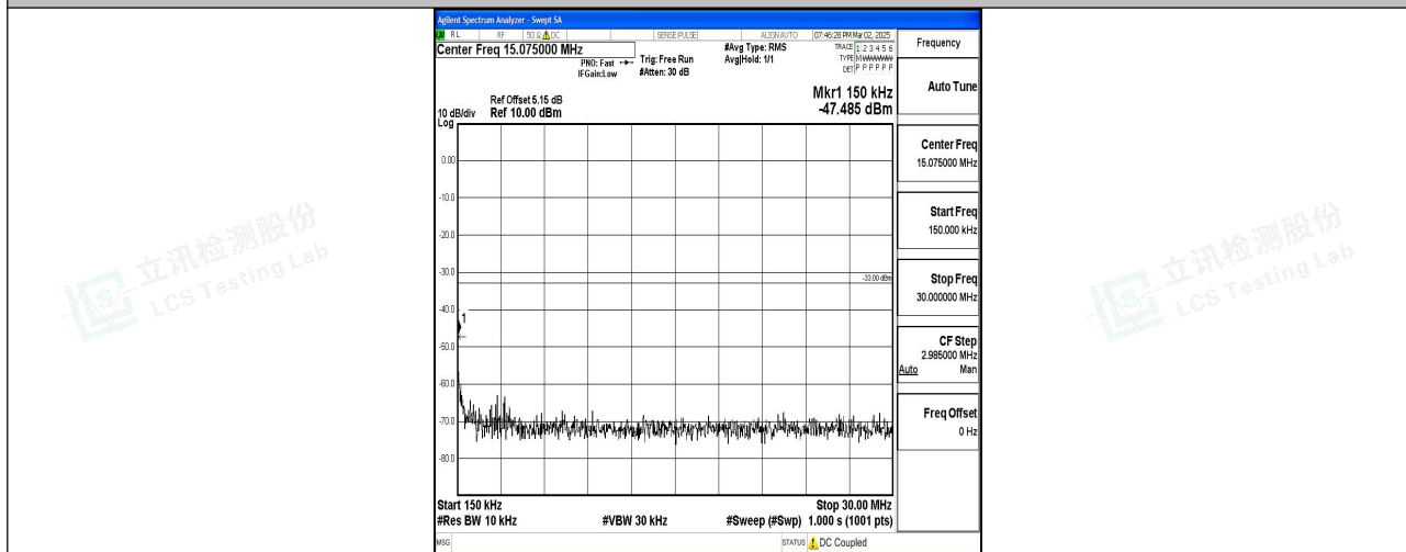
Band2_1.4MHz_QPSK_19193_1RB#0_0.15~30_0.15~30
