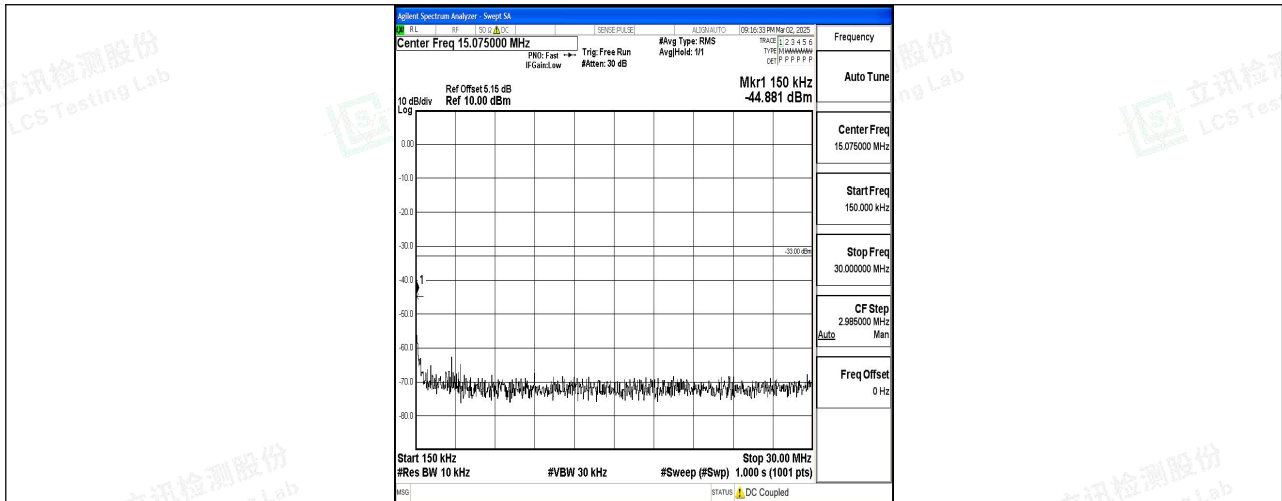
Band2_5MHz_16QAM_18900_1RB#0_0.15~30_0.15~30
