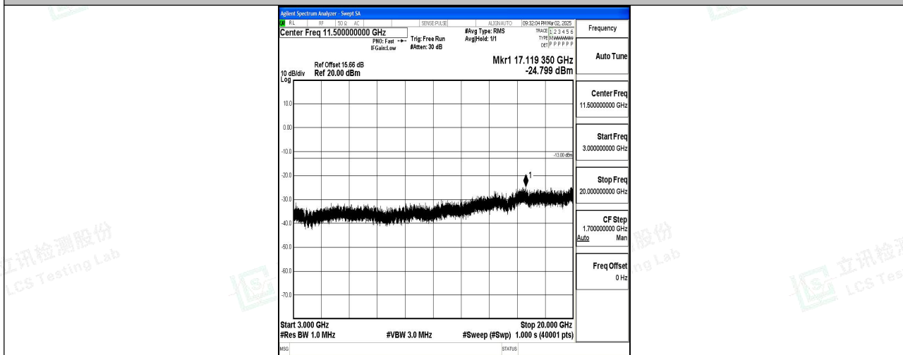
Band2_5MHz_16QAM_19175_1RB#0_3000~20000_3000~20000
