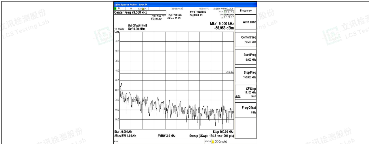
Band2_10MHz_QPSK_18900_1RB#0_0.009~0.15_0.009~0.15
