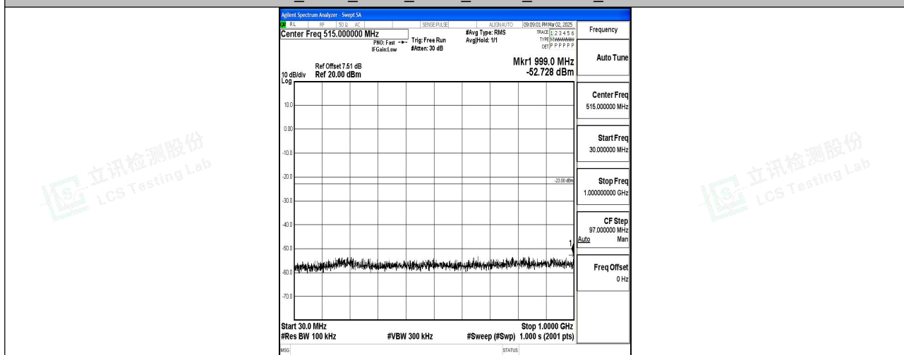
Band2_5MHz_QPSK_18900_1RB#0_30~1000_30~1000
