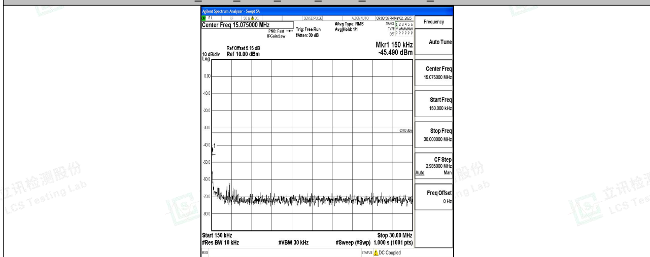
Band2_5MHz_QPSK_18900_1RB#0_0.15~30_0.15~30
