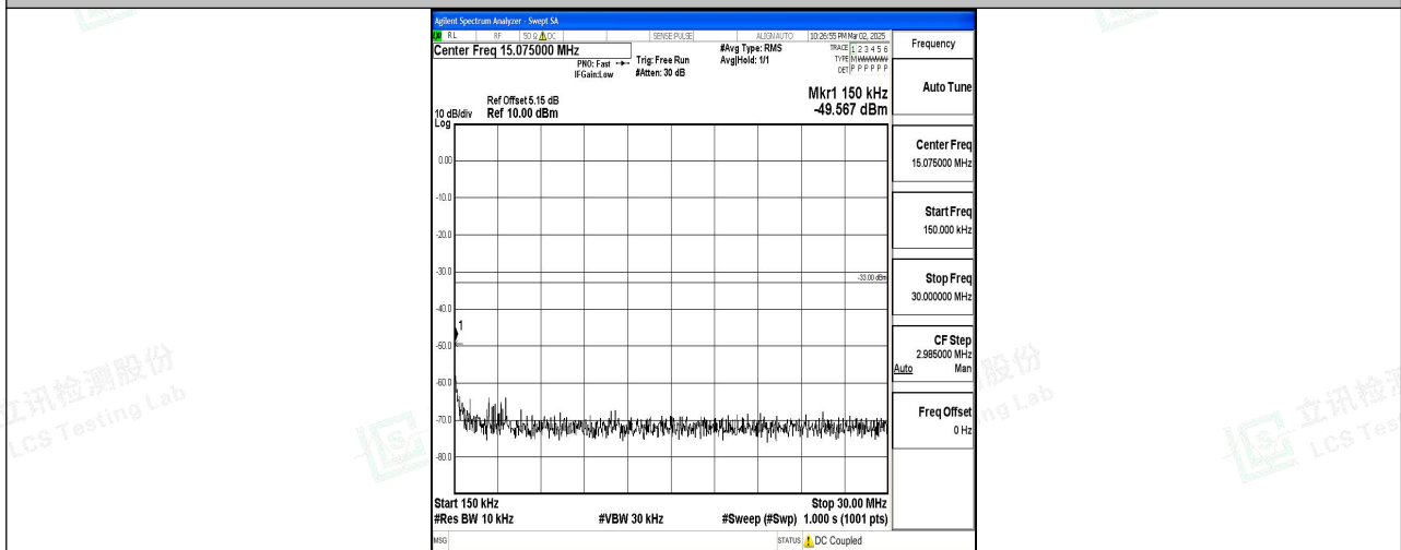
Band2_10MHz_QPSK_18900_1RB#0_0.15~30_0.15~30
