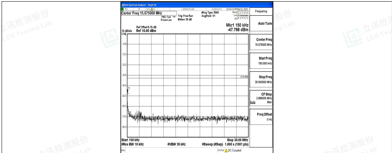
Band2_10MHz_16QAM_18900_1RB#0_0.15~30_0.15~30
