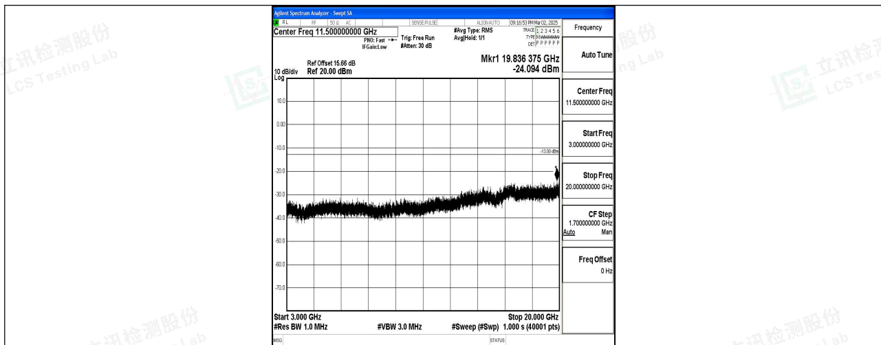
Band2_5MHz_16QAM_18900_1RB#0_3000~20000_3000~20000
