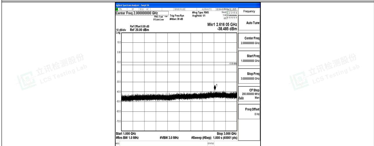
Band2_10MHz_16QAM_18900_1RB#0_1000~3000_1000~3000
