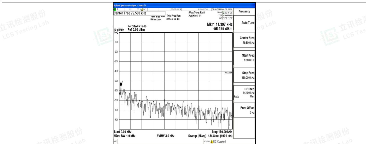
Band2_5MHz_QPSK_18900_1RB#0_0.009~0.15_0.009~0.15
