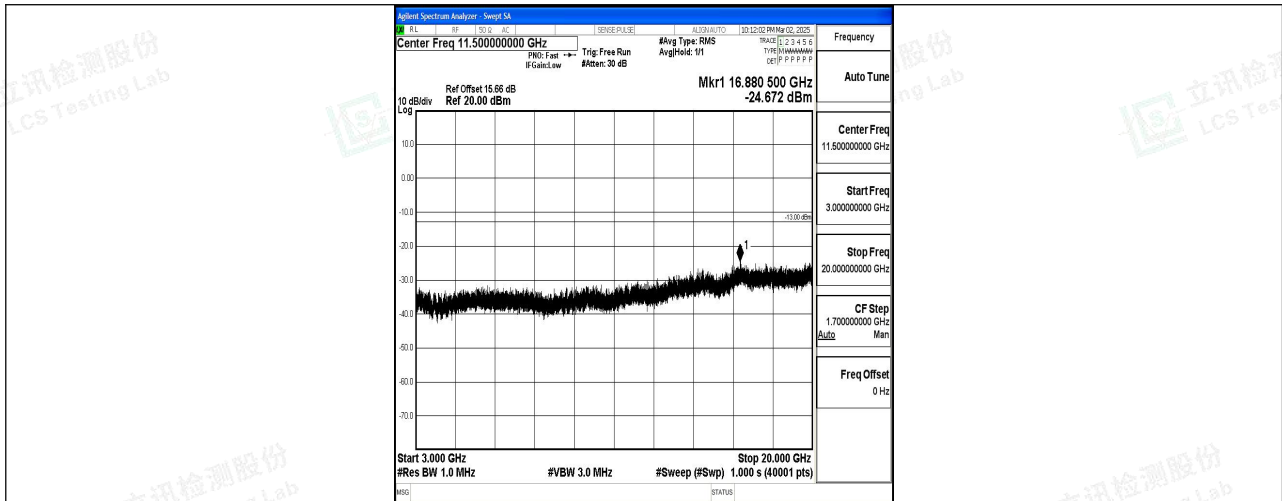
Band2_10MHz_QPSK_18650_1RB#0_3000~20000_3000~20000
