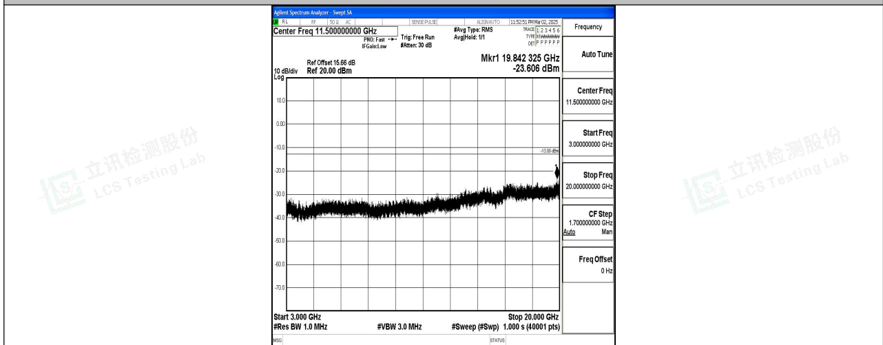
Band2_15MHz_QPSK_19125_1RB#0_3000~20000_3000~20000
