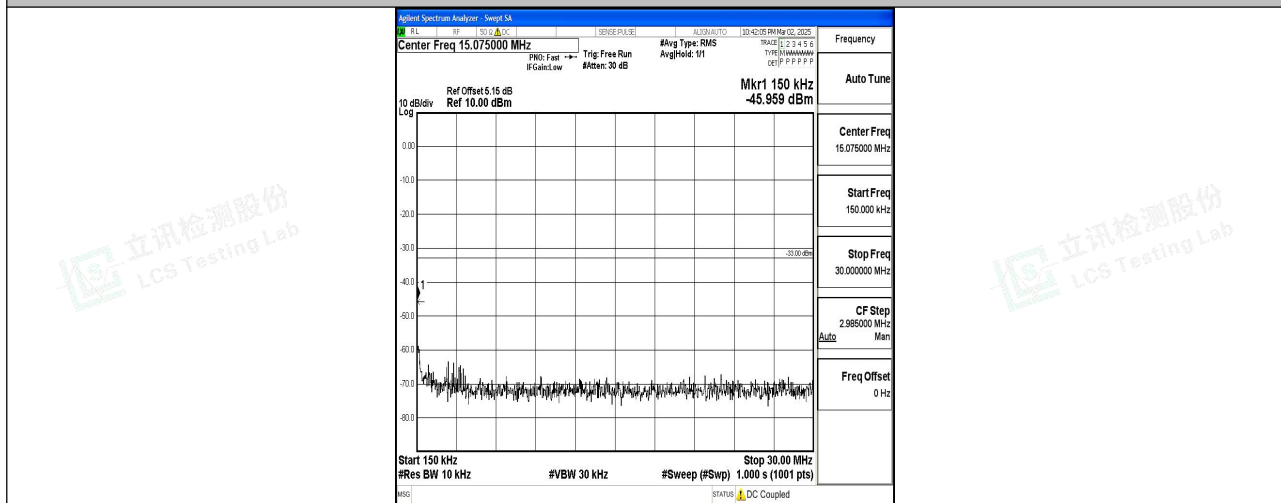
Band2_10MHz_QPSK_19150_1RB#0_0.15~30_0.15~30
