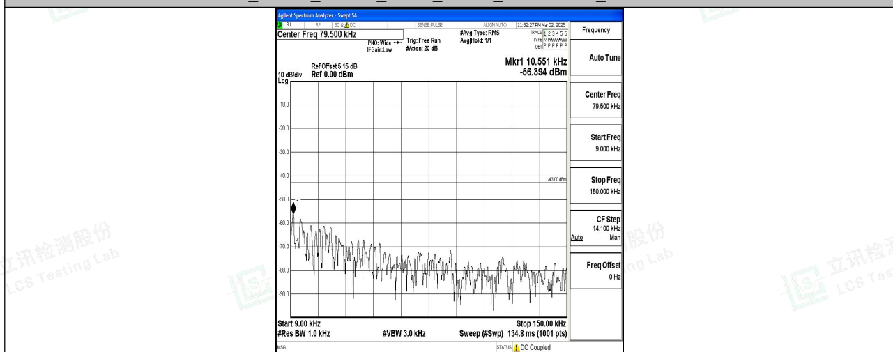
Band2_15MHz_QPSK_19125_1RB#0_0.009~0.15_0.009~0.15
