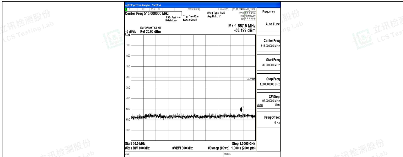
Band2_15MHz_16QAM_18675_1RB#0_30~1000_30~1000
