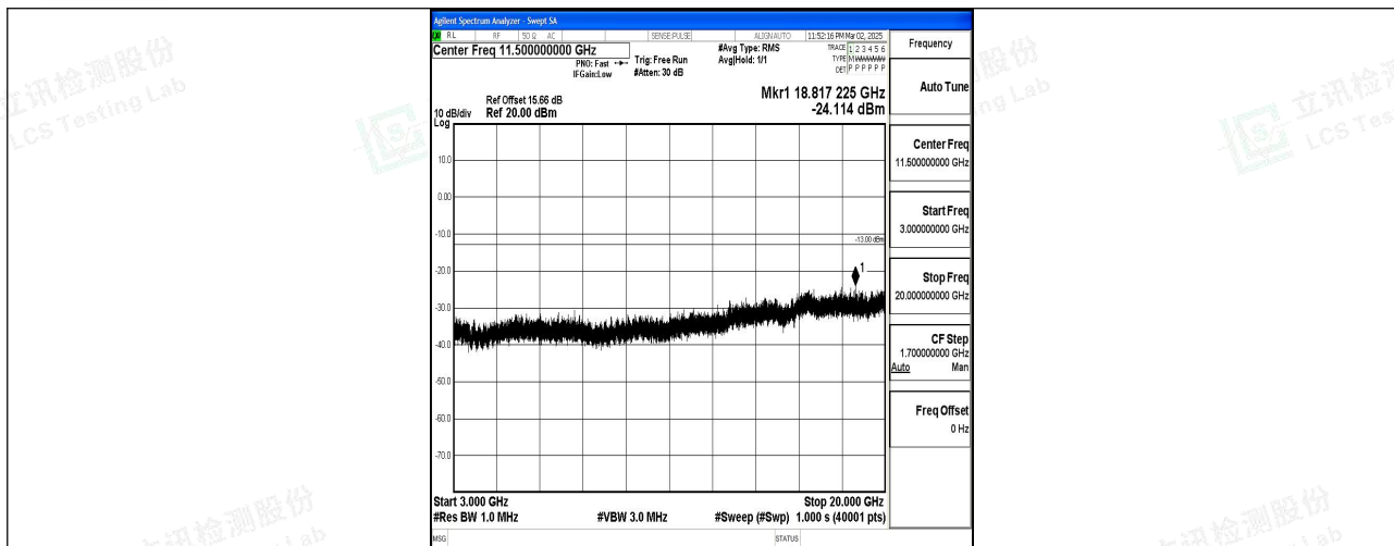
Band2_15MHz_16QAM_18900_1RB#0_3000~20000_3000~20000
