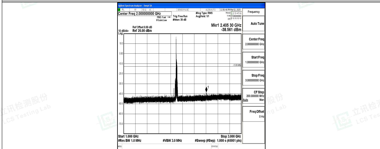
Band2_20MHz_QPSK_19100_1RB#0_1000~3000_1000~3000
