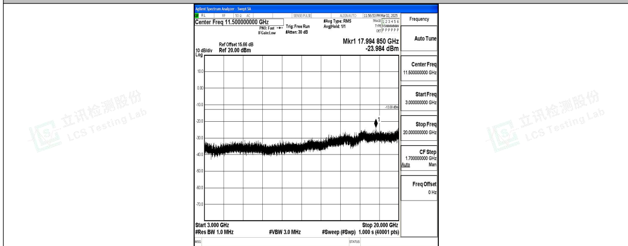
Band2_20MHz_QPSK_19100_1RB#0_3000~20000_3000~20000
