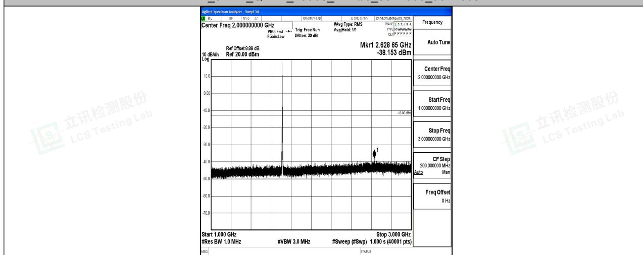
Band4_3MHz_QPSK_19965_1RB#0_1000~3000_1000~3000
