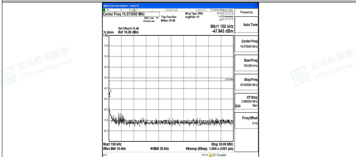
Band4_20MHz_QPSK_20300_1RB#0_0.15~30_0.15~30
