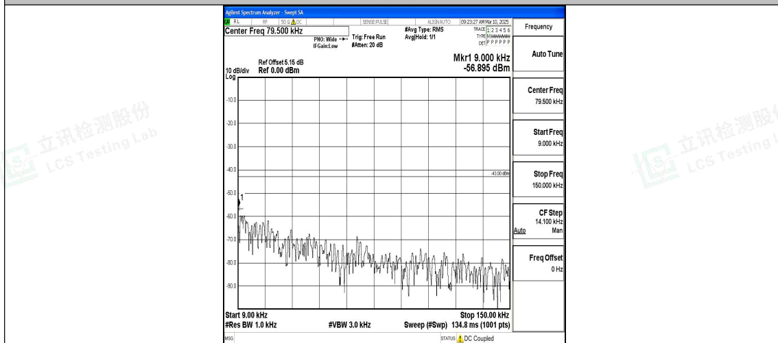
Band66_15MHz_16QAM_132322_1RB#0_0.009~0.15_0.009~0.15
