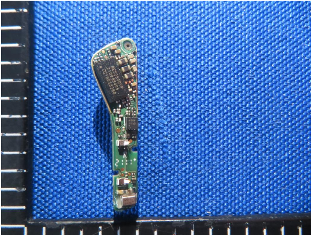
(9) EUT Photo (Right Earbud)
