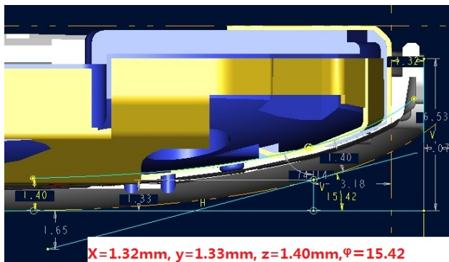
The device exterior radius dimension
