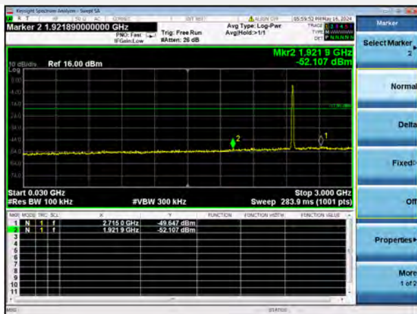
802.11b 11 CHANNEL, SPURIOUS 30 MHz ~ 3 GHz
