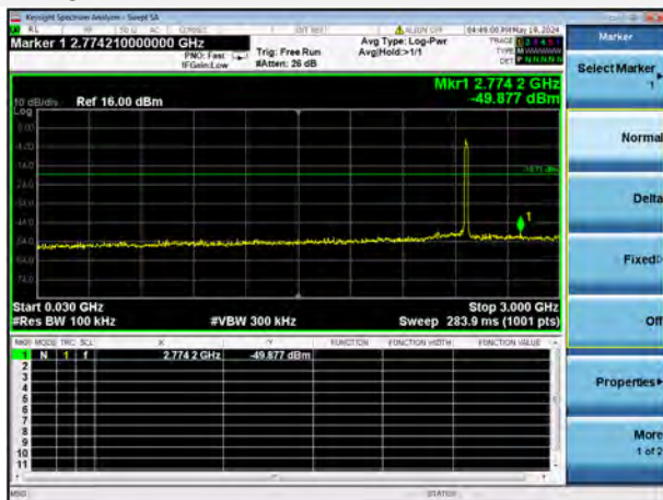
802.11g 12 CHANNEL, SPURIOUS 30 MHz ~ 3 GHz
