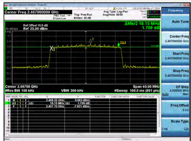
802.11ax-20 MHz(SU) 12 CHANNEL
