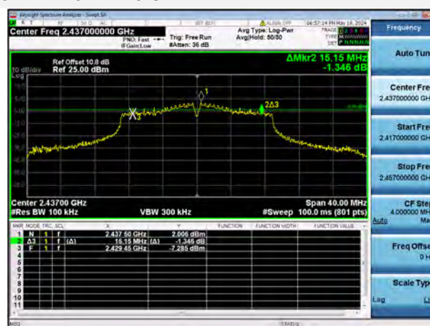
802.11n-20 MHz 6 CHANNEL
