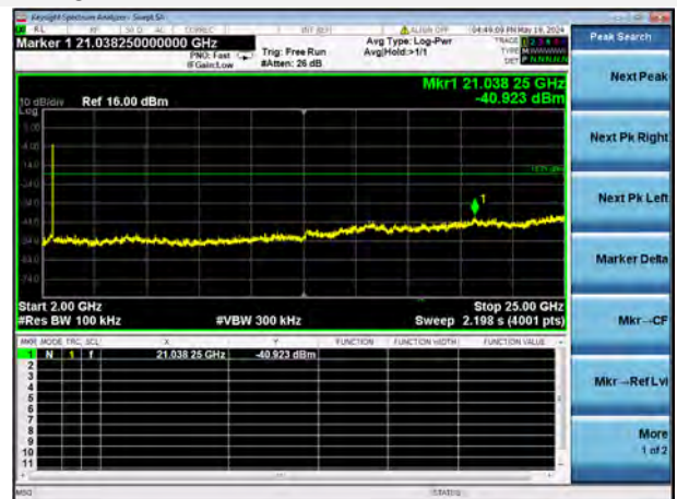
802.11g 12 CHANNEL, SPURIOUS 2 GHz ~ 25 GHz
