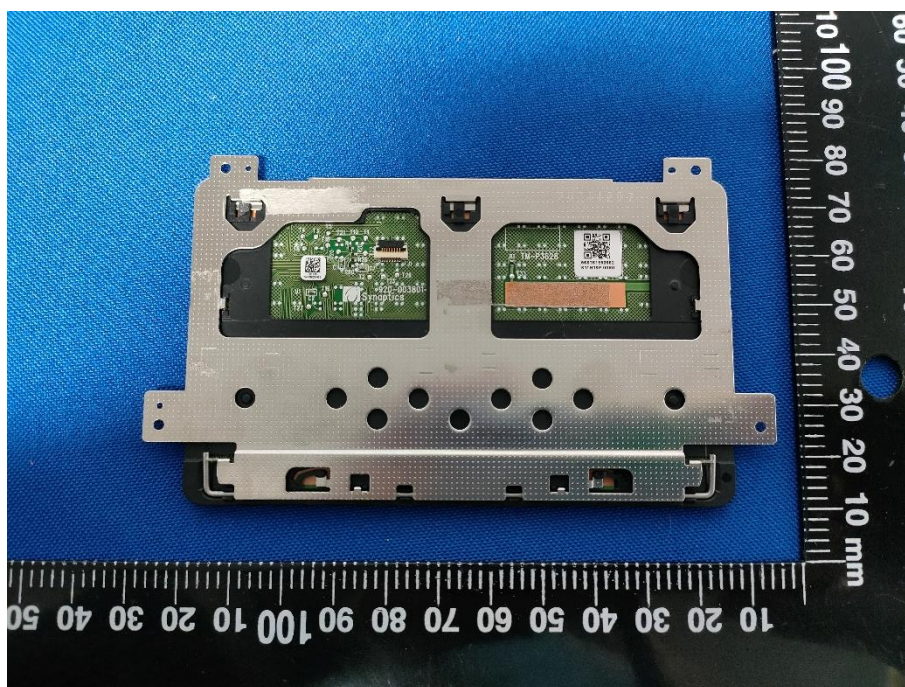
Touch Tablet REAR VIEW
