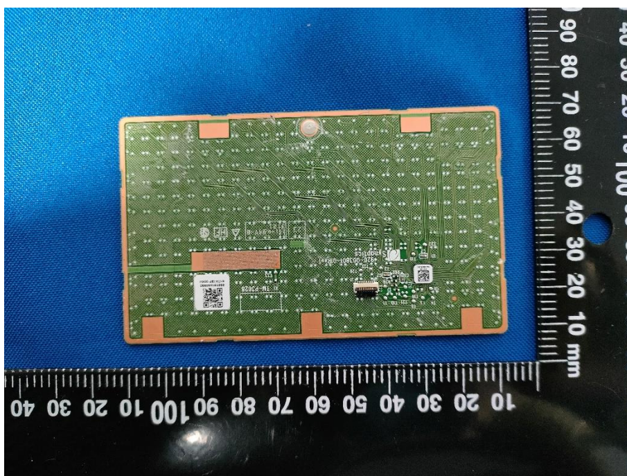
BOARD 1 REAR VIEW
