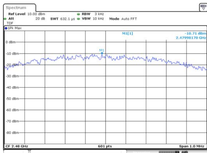
GFSK (BLE) HIGH CHANNEL
