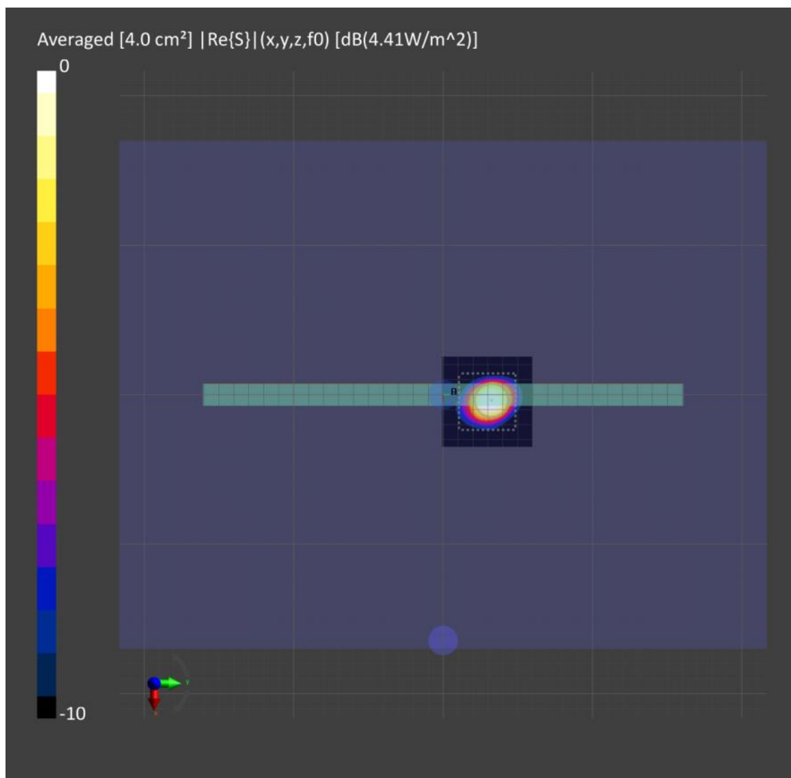
Figure 8-3: 4cm2-averaged power density distribution measured at input.power.limit of 9.5 dBm on the back surface for n260 beam 2
