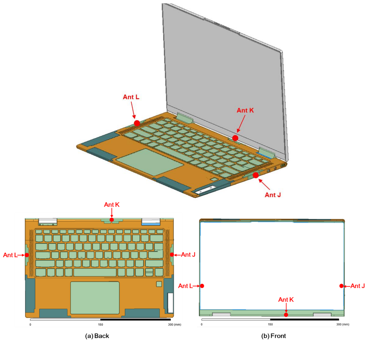
Figure 3 Simulation model which is mounted three mmWave antenna modules.
