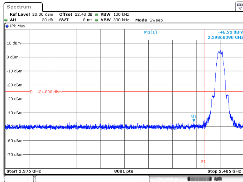
Low Band Edge Plot on Channel 00_1Mbps
