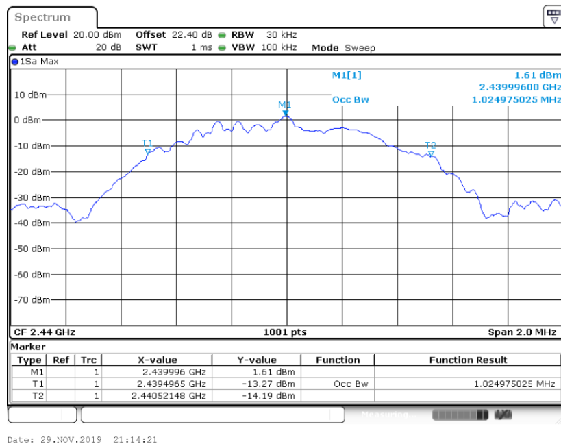
99% Occupied Bandwidth Plot on Channel 19_1Mbps
