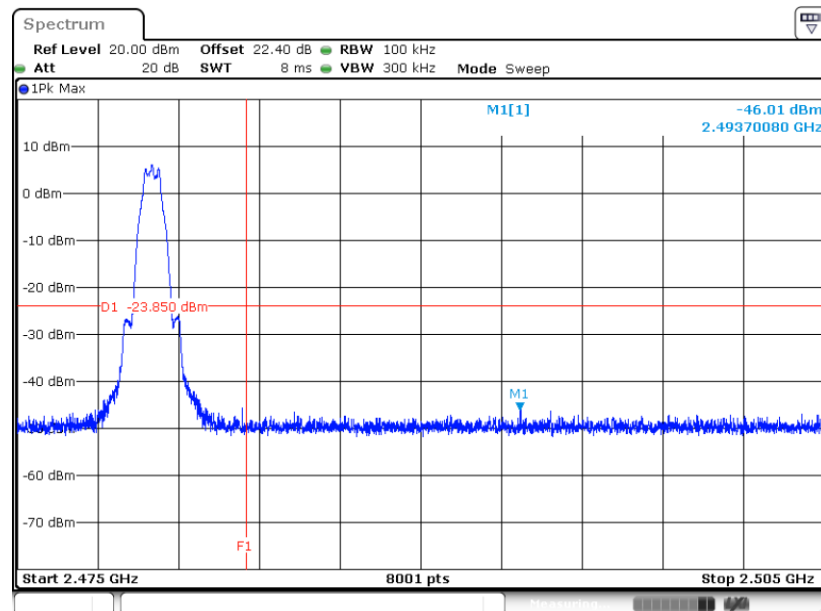
High Band Edge Plot on Channel 39_1Mbps
