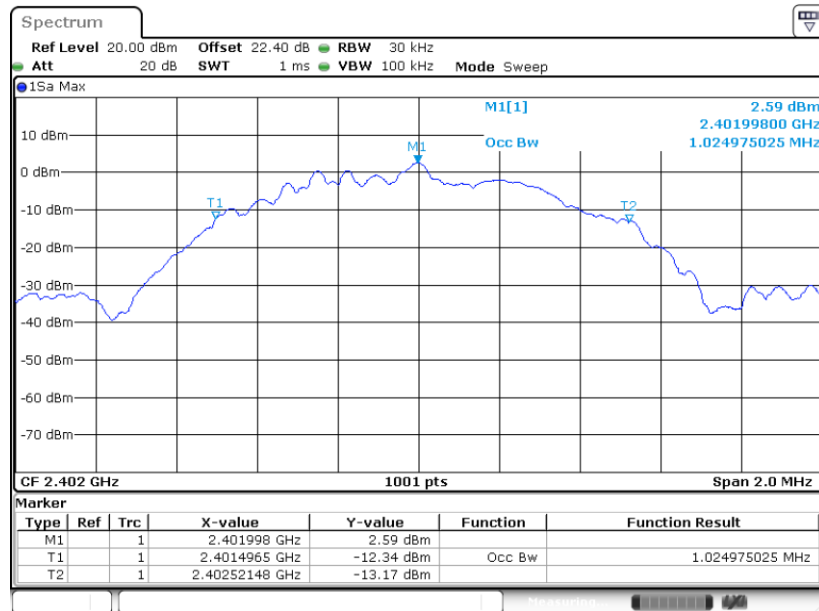
99% Bandwidth Plot on Channel 00_1Mbps
